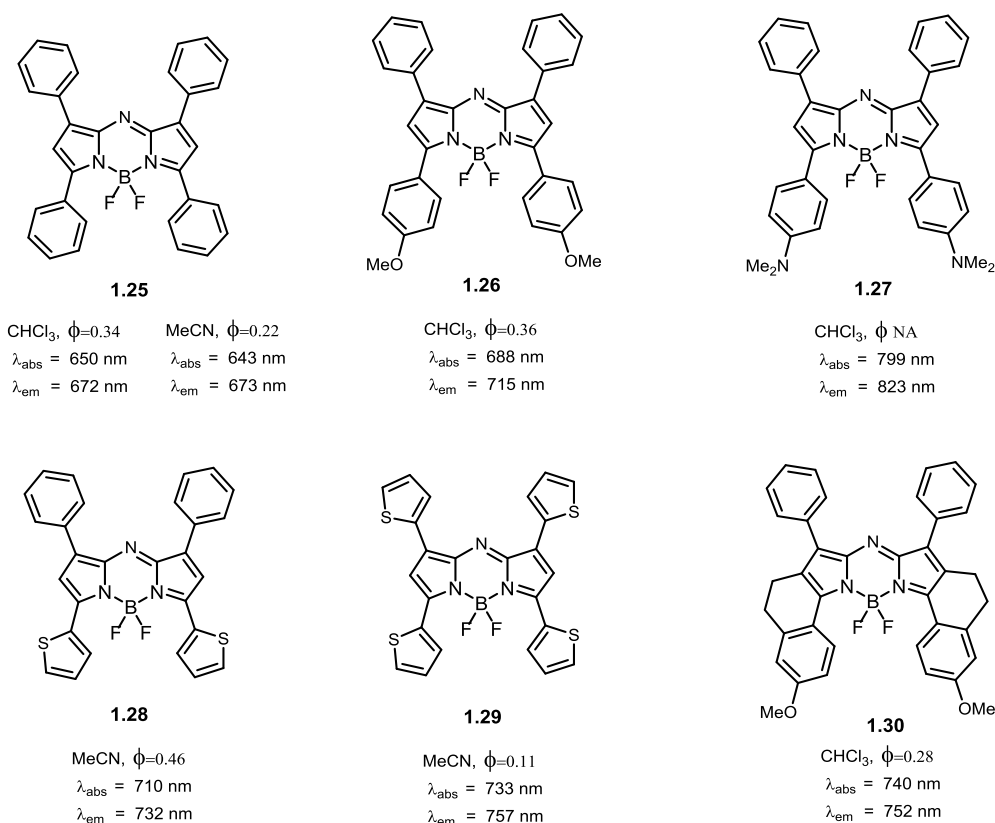
Figure 1.15. Examples of NIR azaBODIPYs. (The optical data in the figure are from the previous publications)
