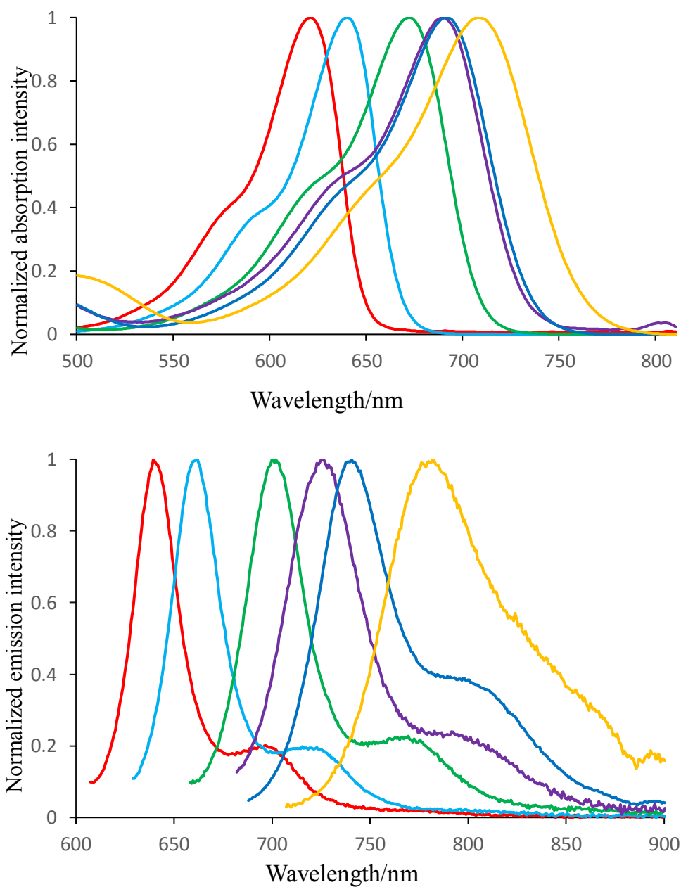
Figure 2.8. Normalized absorption and fluorescence (uncorrected) spectra of BODIPYs 2.1–2.6 in dichloromethane (DCM). They were excited at 600 nm, 620 nm, 650 nm, 680nm, 650nm and 670 nm, respectively. (red, 2.1 ; light blue, 2.2 ; green, 2.3 ; purple, 2.4 ; blue, 2.5 ; and yellow, 2.6 , respectively).
