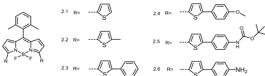
Figure 2.7. The structure of BODIPY dyes 2.1–2.6
