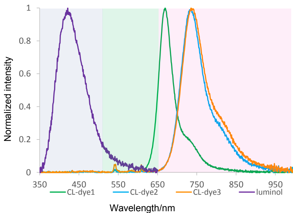
Figure 3.7. Normalized chemiluminescence emission spectra of dyes 3.1a–3.1c and luminol # . #: the spectra of luminol was recorded as the following condition: the mixture of the dye (80 \mu M in 0.1M K_2CO_3 aq., 500 \mu l), H_2O_2 (0.12 M in H_2O , 17 \mu l) and HRP (10 \mu M in 0.1M K_2CO_3 aq., 500 \mu l).
