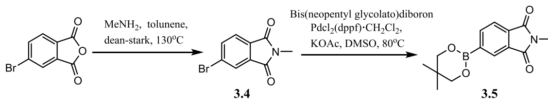
Figure 3.4 synthesis scheme for compound 3.5
