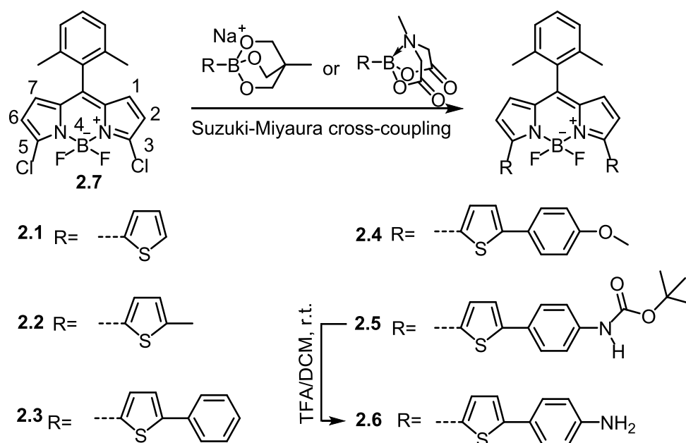
Figure 2.6. Synthetic scheme to NIR BODIPY dyes.
