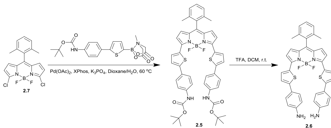
Figure 2.2. The synthesis scheme of dyes 2.5–2.6
