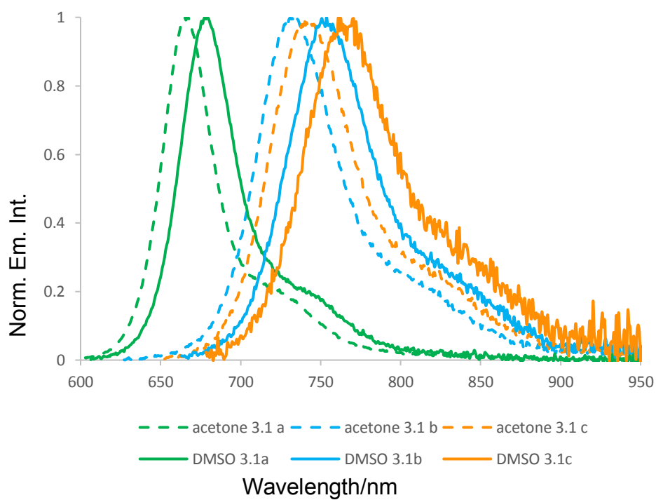
Figure 3.6. Normalized emission spectra of dyes 3.1a-3.1c in acetone and DMSO.
