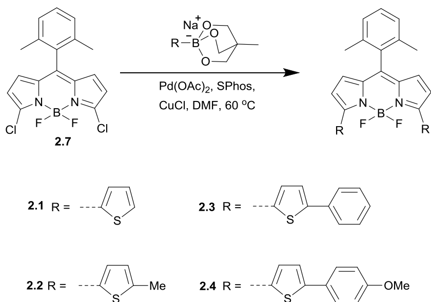
Figure 2.1. Synthesis scheme of dyes 2.1 – 2.4
