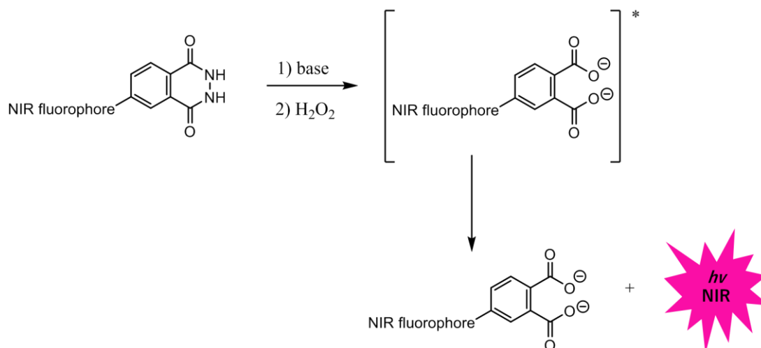
Figure 3.2. General design and chemiluminescence activation pathway of NIR luminophore based on luminol. The emitting light is expected to be varied by the choice of fluorophore.
