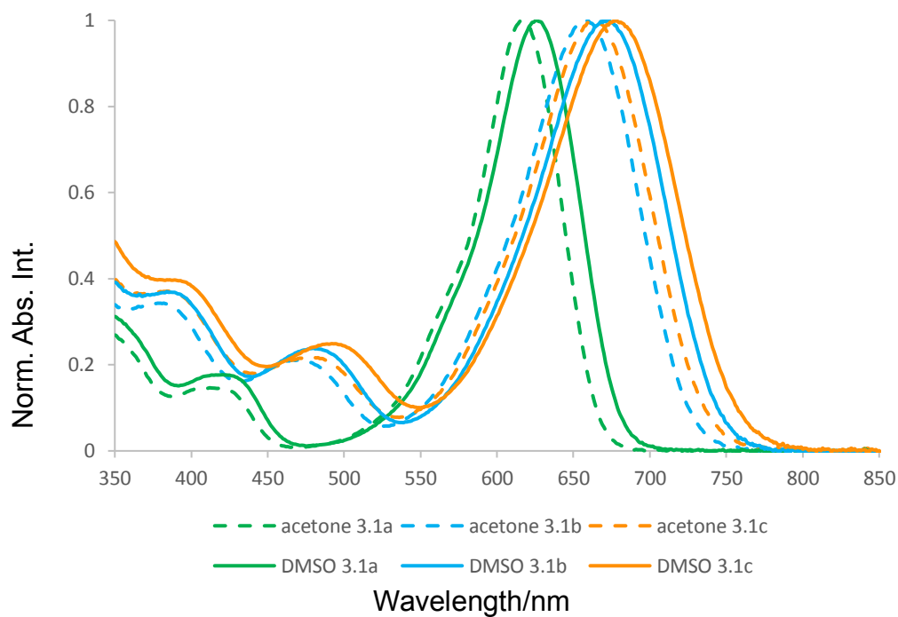
Figure 3.5. Normalized absorption spectra of dyes 3.1a-3.1c in acetone and DMSO.
