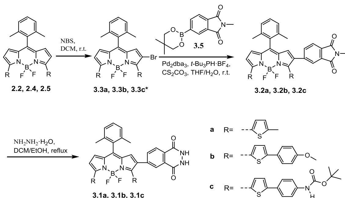
Figure 3.3. Synthesis scheme for chemiluminescent NIR BODIPY dyes 3.1a-3.1c .
