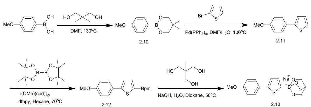
Figure 2.4. The synthesis scheme of 2.13
