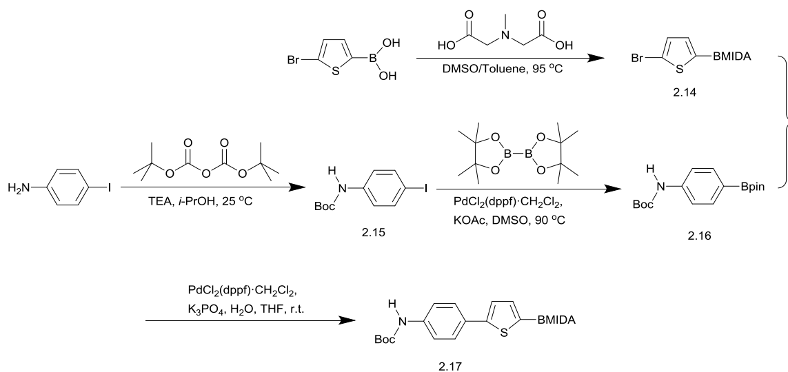
Figure 2.5. The synthesis scheme of 2.17
