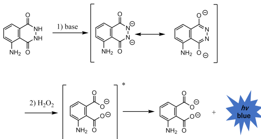
Figure 3.1. Mechanism and chemiluminescence activation pathway of luminol.
