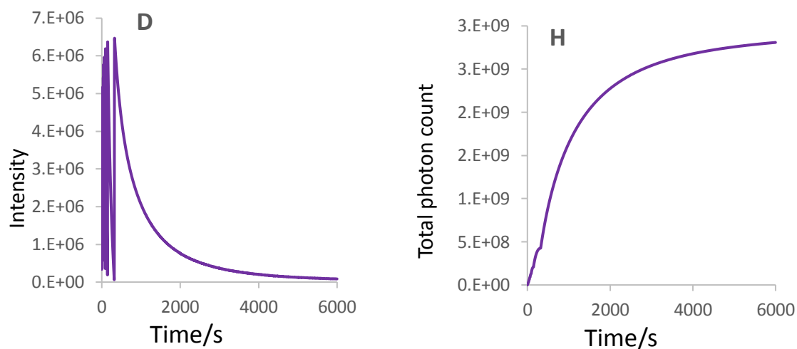
Figure 3.8. (A-D) Chemiluminescent kinetic profiles of 80 \mu M (A) dye 3.1a , (B) dye 3.1b , (C) dye 3.1c (D) luminol (green, blue, yellow, purple lines, respectively). (E-H) Total photon counts emitted from (E) dye 3.1a , (F) dye 3.1b , (G) dye 3.1c , (H) luminol.
