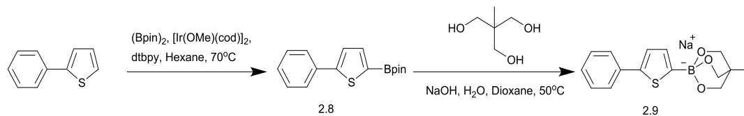
Figure 2.3. Synthesis scheme of compound 2.9
