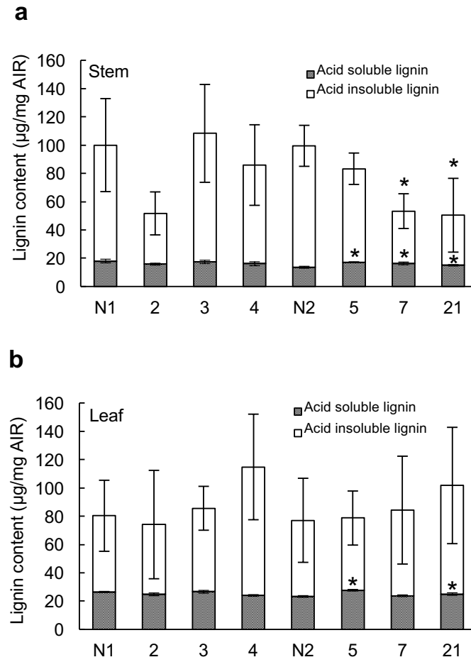
Figure 2.8 Lignin content in the AIR of (a) stems and (b) leaves. N1, N2, plants regenerated from non-transgenic calluses; 2–4, OsSWN2-SRDX plants generated from N1 callus; 5, 7, 21, OsSWN2-SRDX plants generated from N2 callus. Error bars represent SD of quadruplicate experiments. * Significantly different from the respective source plant by Dunnett's test at P < 0.05 .
