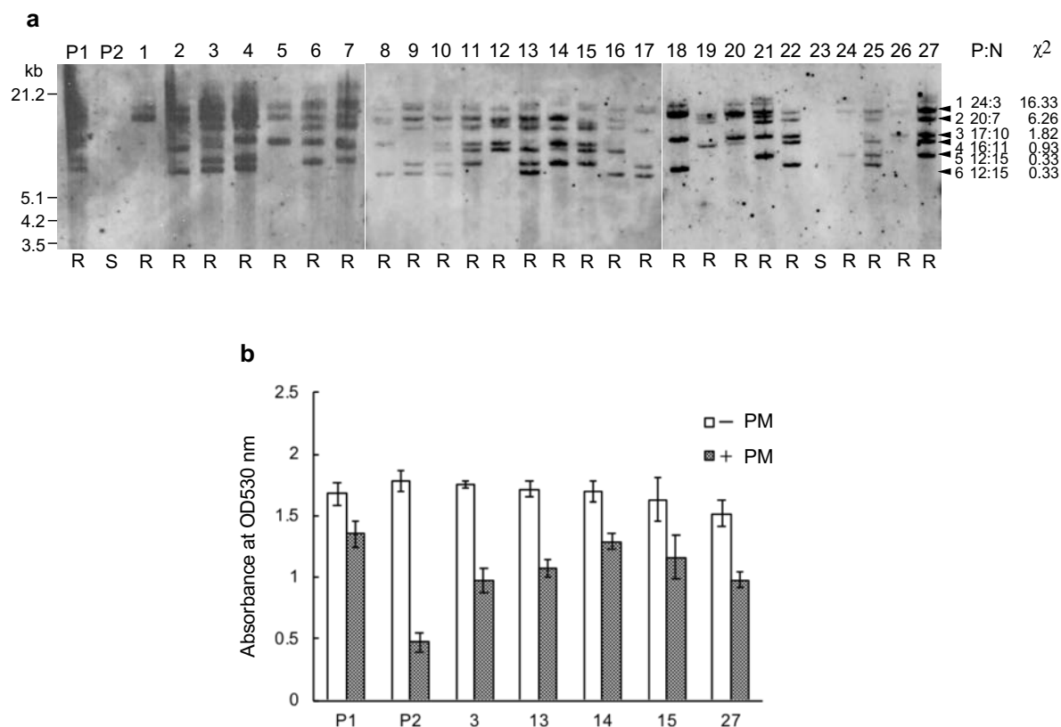
Figure 3.6 Inheritance of the OsALS (sm) gene in the T 1 progeny. (a) Southern blot analysis with the OsALS probe. P1, transgenic plant no. 1 (pollen parent); P2, wild-type plant (seed parent); 1–27, T 1 plants; R, resistant; S susceptible to PM. The segregation ratio of positive (P) to negative (N) plants was analyzed for each band by the chi-squared test. \chi^2 (0.05) = 3.84; \chi^2 (0.01) = 6.64. (b) ALS activity. Error bars represent SE of triplicate experiments.
