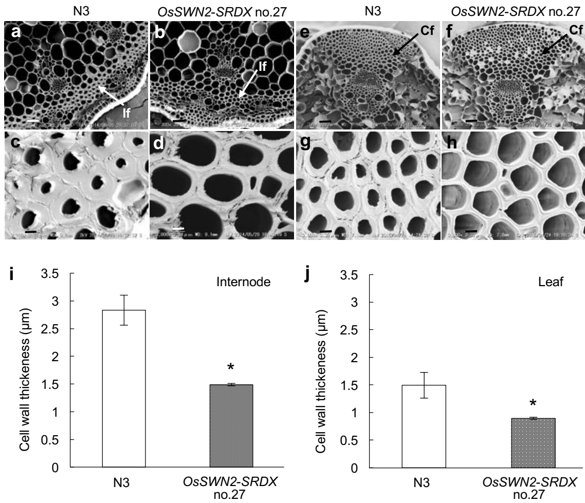
Figure 2.5 Secondary cell walls in cross-sections of (a, c, e, g) wild-type and (b, d, f, h) transgenic plants examined by scanning electron microscopy. (a, b) Internodes. If, Interfascicular fiber. (c, d) Interfascicular fibers of the internodes. (e, f) Leaf veins. Cf, Cortical fiber cells. (g, h) Cortical fiber cells between epidermal cells and the vascular bundle of the leaf vein. Bars indicate 33.3 μm (a, b, e, f) or 3.33 μm (c, d, g, h). (i) Cell wall thickness in internodes. (j) Cell wall thickness in leaves. Error bars represent SD of triplicate experiments. * Significantly different from the source plant by Welch's t -test at P < 0.05 .
