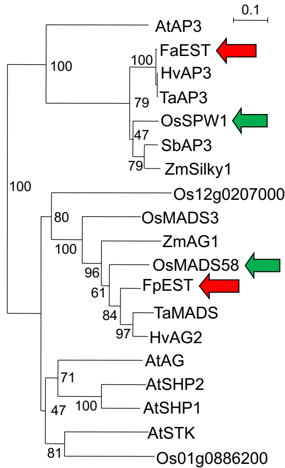
Figure 4.2 Neighbor-joining phylogenetic tree of AP3 - and AG -related Arabidopsis and monocot genes. Numbers at the nodes indicate bootstrap percentage of 1000 replicates. At, Arabidopsis ; Fa, tall fescue; Fp, meadow fescue; Hv, barley; Os, rice; Sb, sorghum; Ta, bread wheat; Zm, maize; EST, expressed sequence tag. Red arrows indicate partial EST sequences isolated from floral organs of Festuca species, which are orthologs of rice genes (green arrows). Scale bar indicates the number of substitutions per site.
