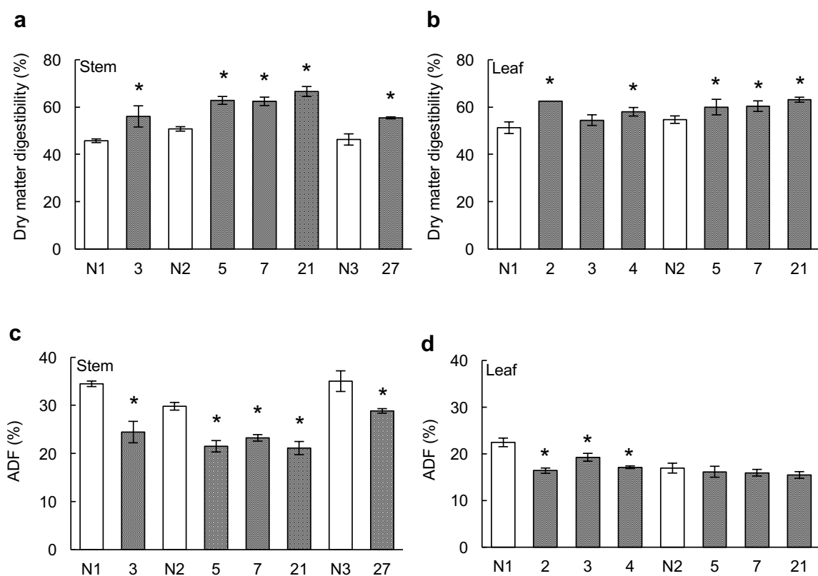
Figure 2.7 Digestibility of wild-type and transgenic plants. (a) Dry matter digestibility of stems. (b) Dry matter digestibility of leaves. (c) ADF of stems. (d) ADF of leaves. N1–N3, plants regenerated from non-transgenic calluses; 2–4, OsSWN2-SRDX plants generated from N1 callus; 5, 7, 21, OsSWN2-SRDX plants generated from N2 callus; 27, OsSWN2-SRDX plant generated from N3 callus. Error bars represent SD of triplicate clones. No error bar is displayed for no. 2 in b because of duplicate clones. * Significantly different from the respective source plant by Dunnett's test or Student's t -test at P < 0.05 .
