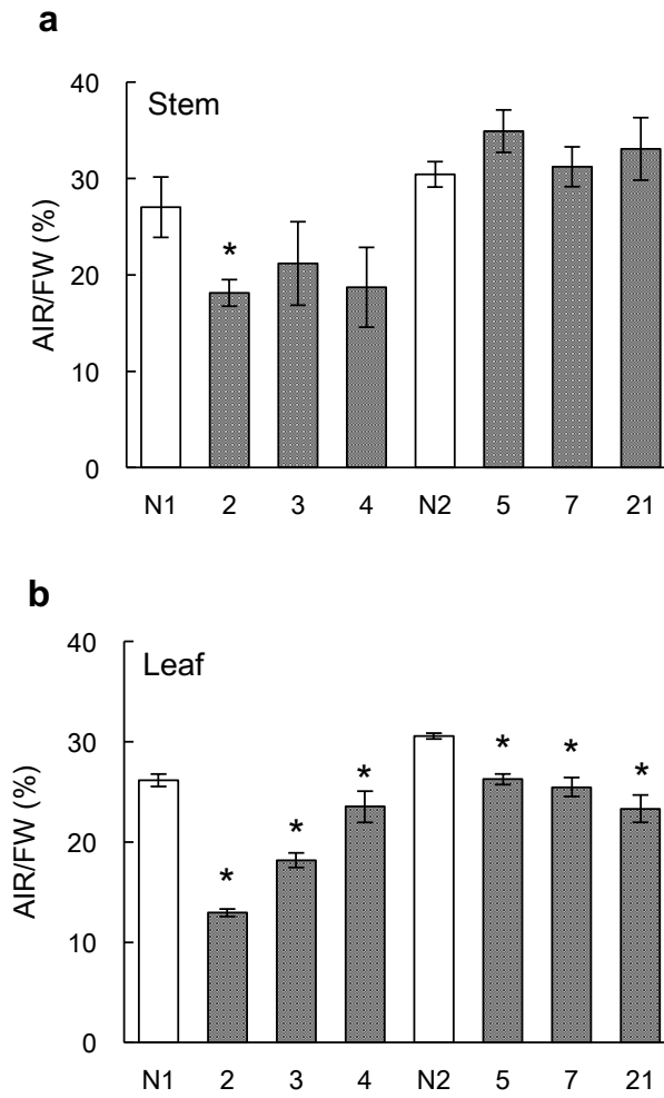
Figure 2.6 The AIR/FW ratio in (a) stems and (b) leaves. N1, N2, plants regenerated from non-transgenic calluses; 2–4, OsSWN2-SRDX plants generated from N1 callus; 5, 7, 21, OsSWN2-SRDX plants generated from N2 callus. Error bars represent SD of quadruplicate experiments. * Significantly different from the respective source plant by Dunnett's test at P < 0.05 .
