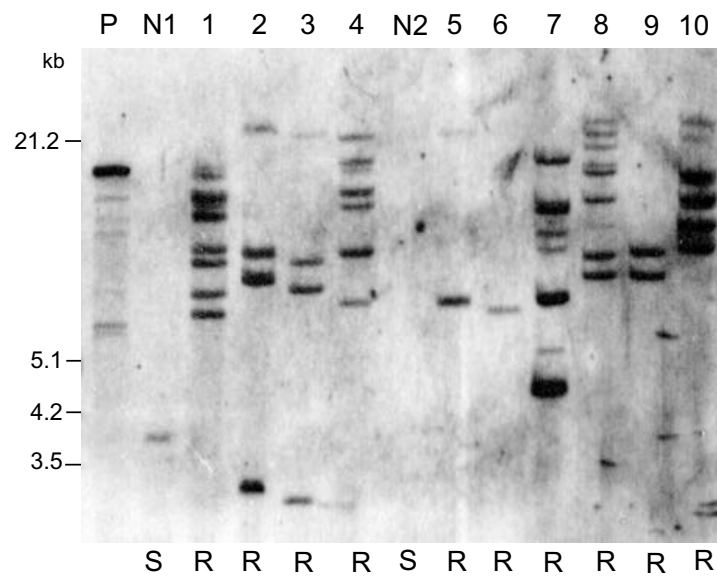
Figure 3.3 Southern blot analysis with the OsALS probe. P, binary vector; N1, N2, wild-type plants; 1–10, transgenic plants; R, resistant; S susceptible to PM.
