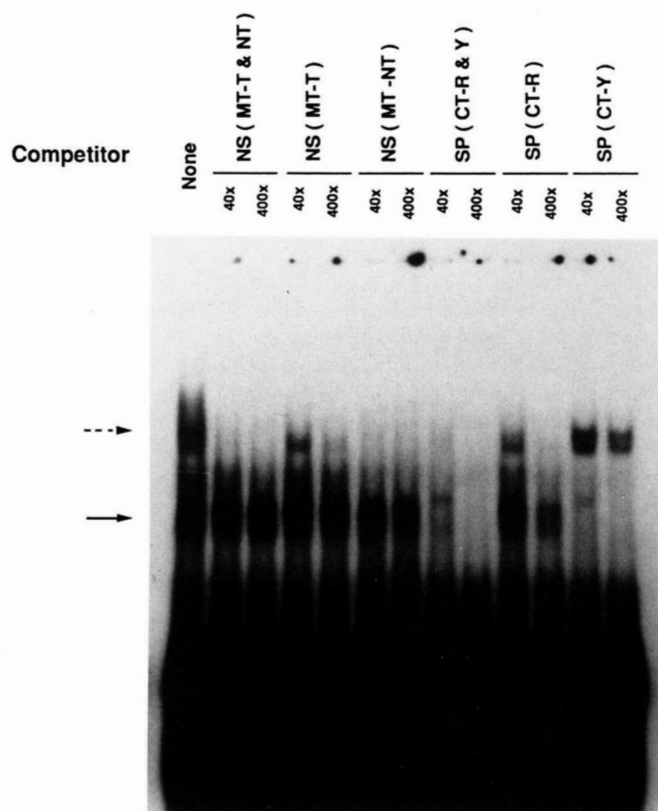
FIG. 5. Specific reduction of the CT binding activity of the affinity-purified proteins by single-stranded CT competitor oligonucleotides. The affinity-purified proteins and the radiolabeled CT oligonucleotide were mixed with or without competitor oligonucleotides, as described under "Experimental Procedures." SP and NS represent specific (wildtype CT) and nonspecific oligonucleotides, respectively. MT-T and MT-NT are the template and non-template strands of an irrelevant competitor oligonucleotide. CT-R and CT-Y indicate the purine-rich and pyrimidine-rich strands of the CT-element, respectively. CT-R and Y and MT-T and NT indicate annealed double-stranded oligonucleotides. Sequences of the oligonucleotides are described in Table I. The molar excess of competitor oligonucleotides compared with the probe is indicated. The thick arrow indicates specific DNA-protein complexes, while the dotted arrow indicates nonspecific ones.
