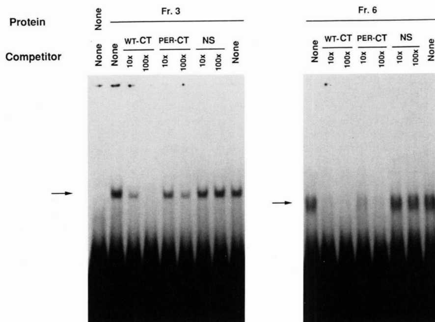
FIG. 4. Reduced binding activity of permuted CT oligonucleotides to hnRNP proteins K and A1 compared with wild-type CT oligonucleotides. The denatured/renatured proteins in fractions 3 and 6 were mixed with radiolabeled CT oligonucleotides, with or without competitor oligonucleotides, as described under "Experimental Procedures." WT-CT, per-CT, and NS indicate wild-type CT, permuted-CT, and nonspecific oligonucleotides, respectively. The molar excess of competitor oligonucleotides relative to the probe is indicated. The oligonucleotides are described in Table I. Arrows indicate specific DNA-protein complexes.
