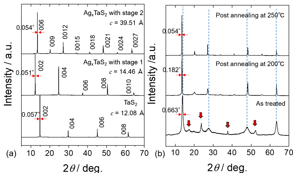
Fig. 2. (a) XRD patterns for pristine \text{TaS}_2 and \text{Ag}^+ intercalated \text{TaS}_2 with stage 1 and 2 structures. (b) Post annealing temperature dependence of normalized XRD patterns for \text{Ag}^+ -intercalated 4Hb- \text{TaS}_2 .
