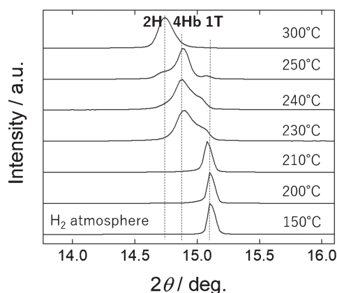
Fig. 3. Shift of the (002) XRD peak of 1T- \text{TaS}_2 after post annealing at various temperatures under a \text{H}_2 atmosphere. 1T- \text{TaS}_2 gradually transforms to 2H- \text{TaS}_2 via 4Hb- \text{TaS}_2 .
