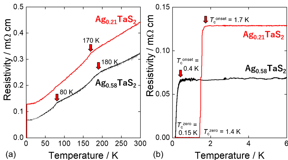
Fig. 4. (a) Temperature dependence of the resistivity for \text{Ag}_{0.58}\text{TaS}_2 and \text{Ag}_{0.21}\text{TaS}_2 from 0.15 to 300 K. (b) An expanded view of (a).
