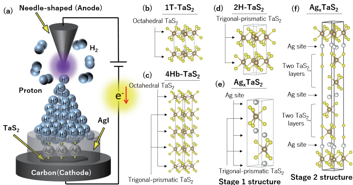
Fig. 1. (a) Schematic of the PDII process. Crystal structures of (b) 1T-TaS 2 , (c) 4Hb-TaS 2 , (d) 2H-TaS 2 , (e) Ag x TaS 2 with stage 1 structure, and (f) Ag x TaS 2 with stage 2 structure.
