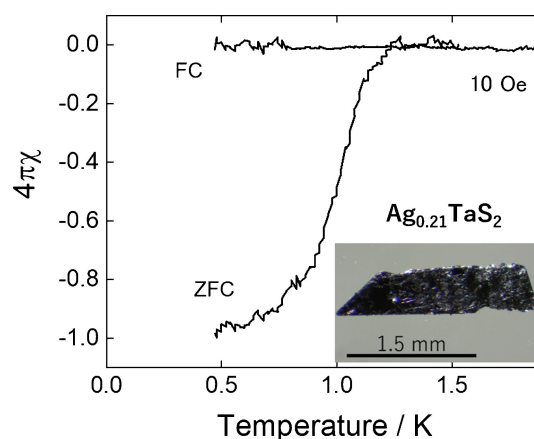
Fig. 5. Temperature dependence of magnetic susceptibility for \text{Ag}_{0.21}\text{TaS}_2 under a 10 Oe field. The inset image is a photograph of the single-crystalline \text{Ag}_{0.21}\text{TaS}_2 .
