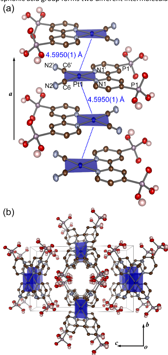
Fig. 2. (a) Stacking and (b) packing structures of 1P . The coordination planes of the Pt(II) ions are shown in blue. The blue, purple, brown, light-blue, and red ellipsoids represent Pt, P, C, N, and O atoms, respectively. The H atoms bonded to the O atoms of the
