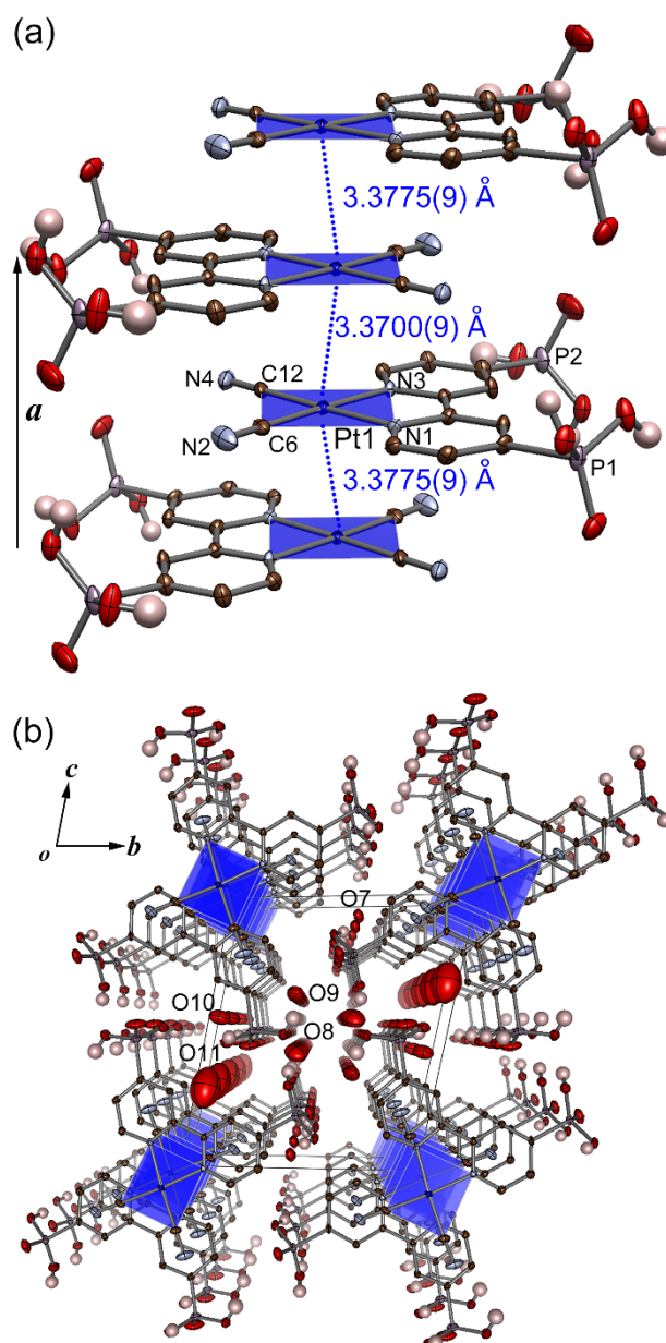
Fig. 1. (a) Stacking and (b) packing structures of 1P·5H 2 O at 200 K. The coordination planes of the Pt(II) ions are shown in blue. The blue, purple, brown, light-blue, and red ellipsoids represent Pt, P, C, N, and O atoms, respectively. The H atoms bonded to the O atoms of the phosphonic acid groups are shown in pink, while the others have been omitted for clarity. Displacement parameters are drawn at the 50% probability level.
