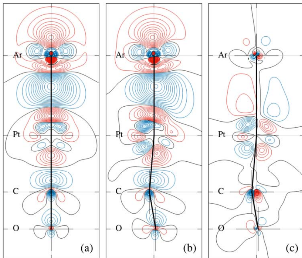
Fig. 3 The contour maps of the electron density difference \Delta\rho = \rho(\text{Ar-PtCO}) - (\rho(\text{Ar}) + \rho(\text{PtCO})) (a) at the equilibrium linear geometry (referred to as \Delta\rho_{\text{linear}} ) and (b) at the bent geometry with Q_4 = 44.2 bohr \text{emu}^{1/2} (referred to as \Delta\rho_{\text{bent}} ), on the y-z plane at the CCSD level; (c) the contour map of the difference of the electron density difference \Delta\rho_{\text{bent}} - \Delta\rho_{\text{linear}} . Blue color denotes an increase of the electron density, while red color denotes a decrease of the electron density. The contour interval is 0.001.
