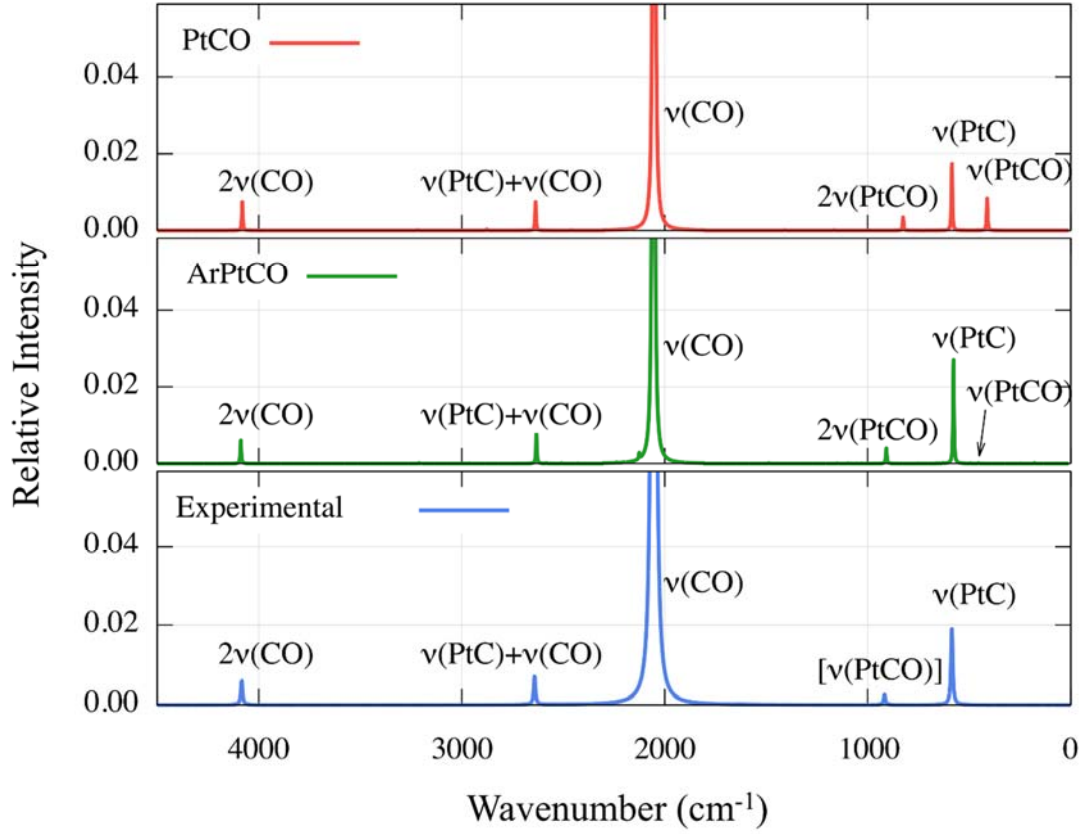
Fig. 1 The calculated IR spectra of PtCO and Ar-PtCO by the direct VCI method, and the experimental IR spectrum for PtCO in the Ar-matrix isolation. The Lorentzian function is plotted at each peak, with a half width of 5 cm -1 .
