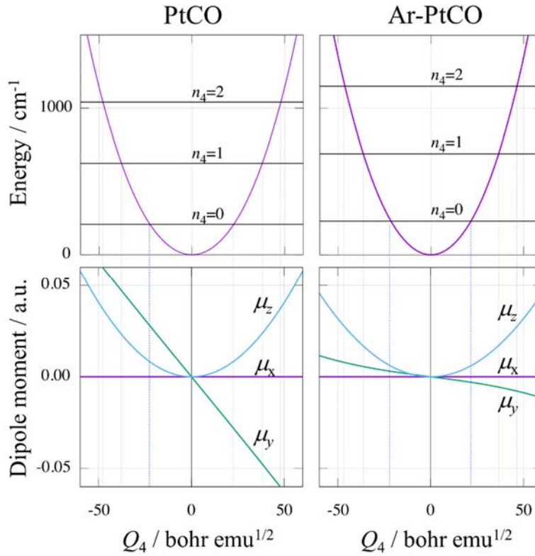
Fig. 2 Potential energy curves and variations of dipole moments of PtCO and Ar-PtCO, as a function of the Pt-C-O bending normal coordinate, Q_4 .
