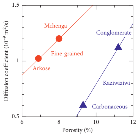
FIGURE 15: Dependence of water vapor diffusion coefficients of Malawi rocks on porosity.
