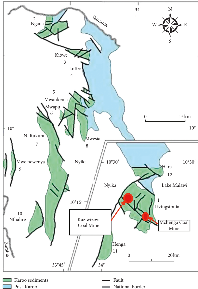
FIGURE 1: Distribution of Karoo basins in northern Malawi: North Nyika Basins and Livingstonia Basin (inset) based on an internal report at the Geological Survey Department in Zomba, Malawi.
