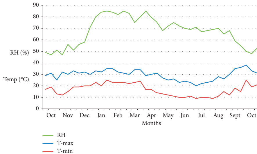
FIGURE 2: Relative humidity and temperature in the Northern Region, 2014-2015 season [16].
