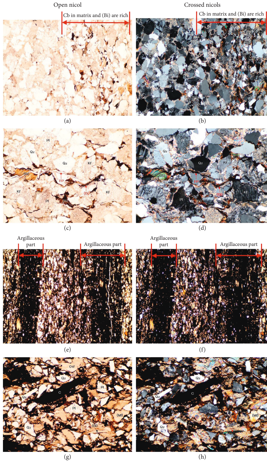
FIGURE 9: Microscopic images of Mchenga arkose sandstone (a, b, c, d) and Mchenga fine-grained sandstone (e, f, g, h). Qz: quartz; Kf: orthoclase; Pl: plagioclase; Bi: biotite; Mf: mafic minerals; C: coaly substances; Cb: carbonate minerals; (-): pseudomorphism; FP: fracture. Widths of the images are 6.0 mm for (a), (b), (e), and (f); 2.5 mm for (c) and (d); and 1.2 mm for (g) and (h).
