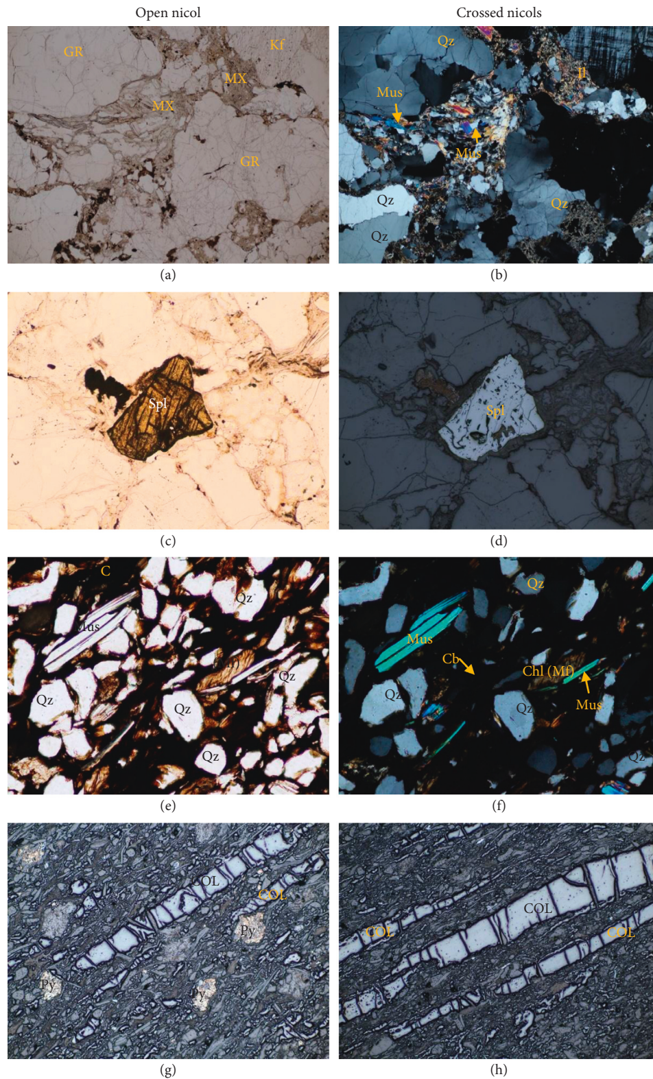
FIGURE 11: Microscopic images of Kaziwiziwi conglomerate (a, b, c, d) and Kaziwiziwi carbonaceous sandstone (e, f, g, h). GR: granites; MX: matrix; Mus: muscovite; Il: illite; Spl: sphalerite; Chl: chlorite; Py: pyrite; COL: coal. Widths of the images are 6.0 mm for (a) and (b); 1.2 mm for (c) and (d); 0.60 mm for (e) and (f); and 2.5 mm for (g) and (h).
