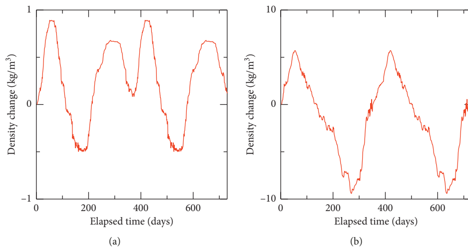
FIGURE 17: Density change for FEM simulation converted from smoothed humidity data. Time is from February 15. (a) Underground conditions. (b) Outside conditions.
