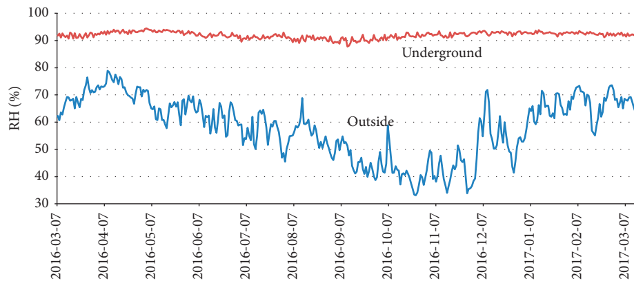
FIGURE 6: Humidity variation: inside the mine (logger #2) and outside.
