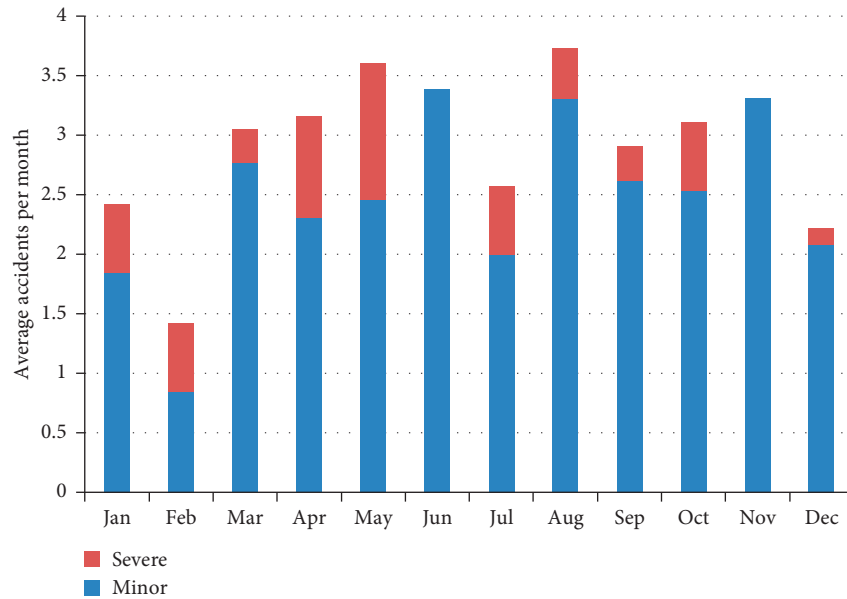
FIGURE 3: Average roof fall accidents per month for Mchenga Coal Mine (1995 to 2009).
