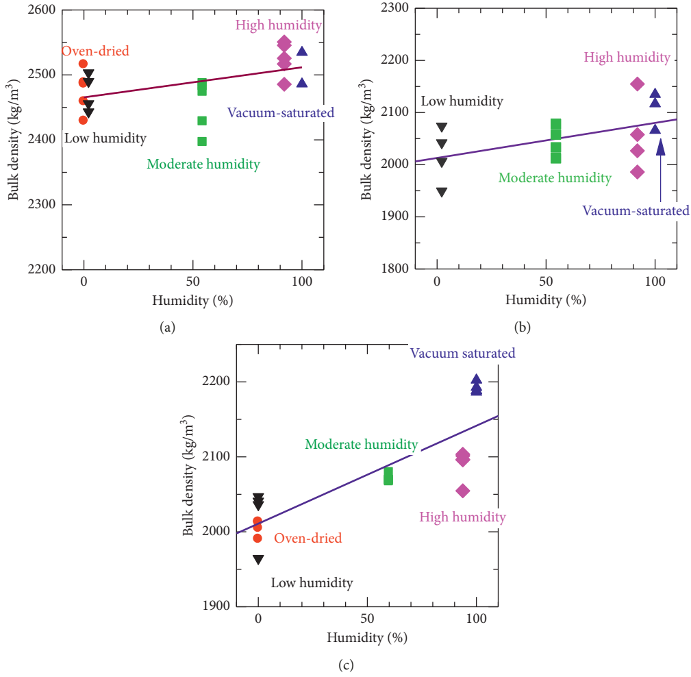
FIGURE 12: Bulk density variation against humidity. (a) Mchenga arkose sandstone. (b) Mchenga fine-grained sandstone. (c) Kimachi sandstone.
