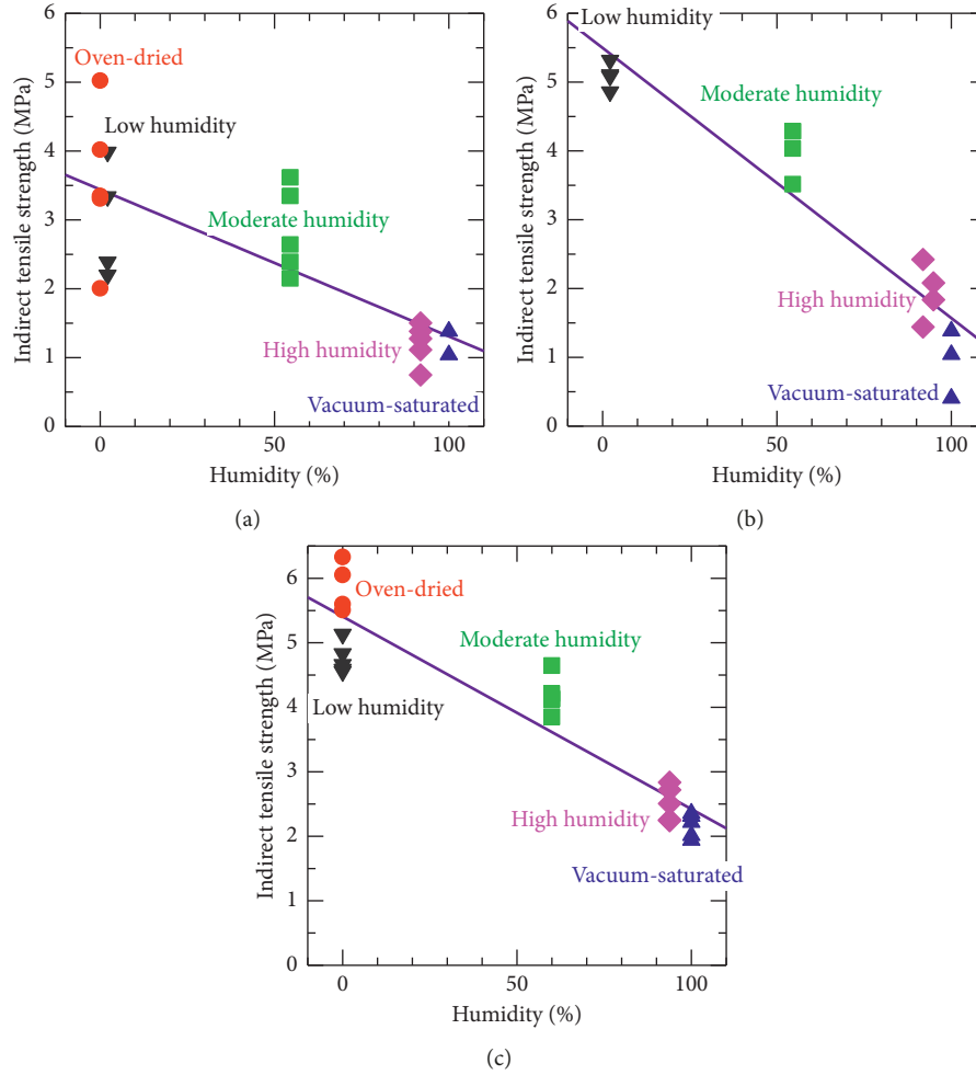
FIGURE 13: Indirect tensile strength variation against humidity. (a) Mchenga arkose sandstone. (b) Mchenga fine-grained sandstone. (c) Kimachi sandstone.
