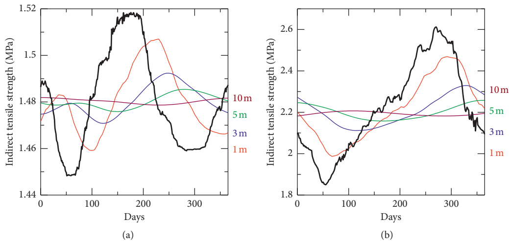
FIGURE 19: Simulation of annual variation. Time is from February 15. The thick black lines show the boundary condition at the bottom. (a) Underground. (b) Outside.
