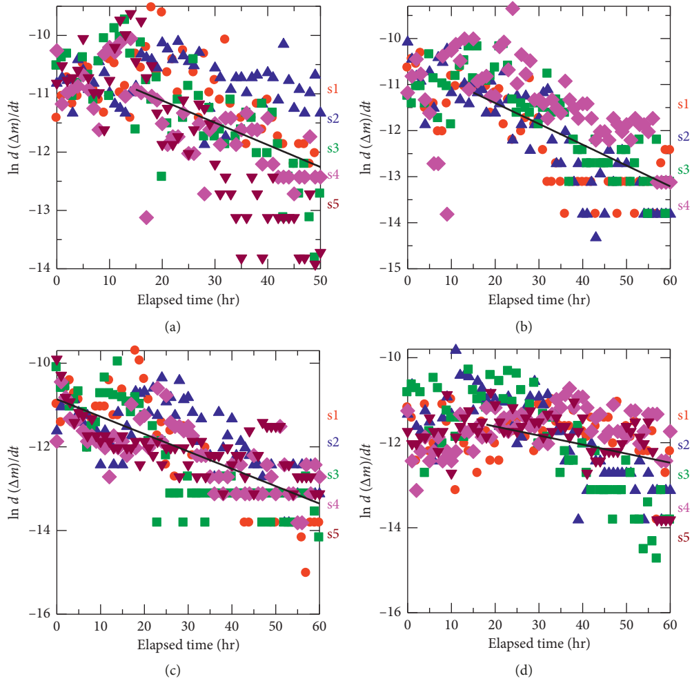
FIGURE 14: Mass change of specimens as a function of elapsed time. The thick black line gives the regression line to calculate average diffusion coefficient. (a) Mchenga arkose sandstone. (b) Mchenga fine-grained sandstone. (c) Kaziwiziwi conglomerate. (d) Kaziwiziwi carbonaceous sandstone.
