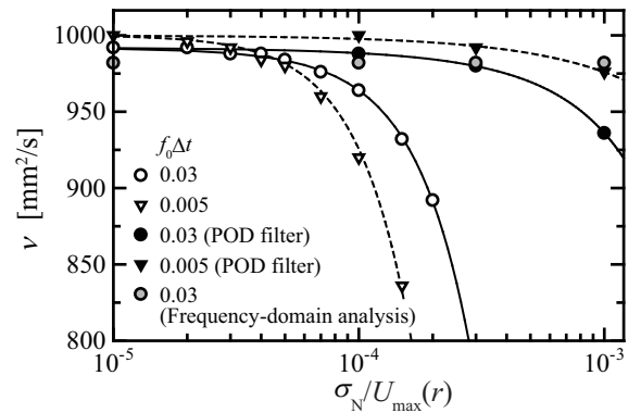
Fig. 3 Estimated values of \nu for different noise levels \sigma_N obtained using two different sampling times, w/o POD filtering and frequency domain analysis; the solid and dashed lines represent fitted parabolic curves of the plots obtained using the least-squares approximation
