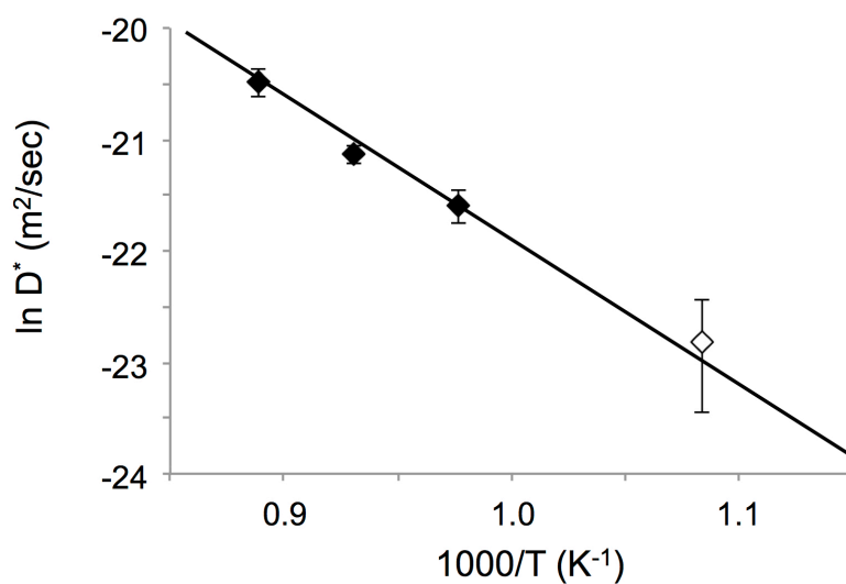
373 374 Figure 4. Arrhenius plot of D^* for silica glass. Error bars represent two standard deviations of D^* 375 evaluated from several diffusion profiles in samples heated for different periods. The D^* shows 376 the Arrhenius relation with the activation energy of 110 \pm 27 kJ/mol. The D^* at 650 °C (open 377 diamond) was not included to determine the activation energy because the error is much larger 378 compared to those of other plots.
