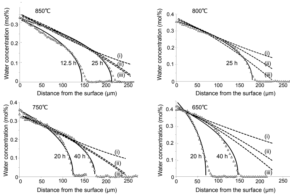
358 Figure 2. Water diffusion profiles in silica glass at 850, 800, 750 and 650 °C, at a water pressure 359 of 50 bar. The profiles are fitted with water diffusion models proposed in previous studies 360 (dashed curves) (see details in the text): (i) concentration-independent water diffusion 361 ( Wakabayashi and Tomozawa, 1989 ), (ii) water diffusion linearly proportional to water 362 concentration ( Doremus, 1969 ), and (iii) water diffusion exponentially proportional to water 363 concentration ( Zhang and Behrens, 2000 ). Fitted curves with the present water diffusion model 364 are shown as solid curves. Water concentrations near the surface of glasses seem to increase with 365 decreasing temperature, which is likely due to the temperature dependence of water solubility in 366 silica glass ( Wakabayashi and Tomozawa, 1989 )
