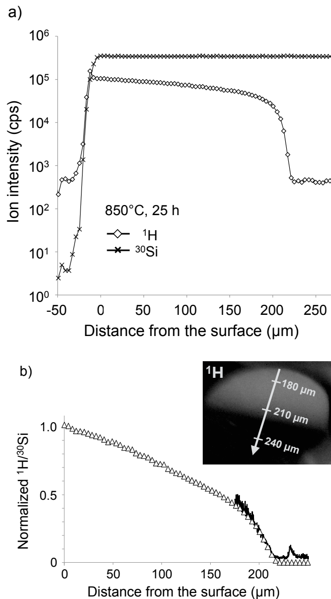
Figure 1. Typical water diffusion profile (#850-2; 850°C for 25 h). (a) Secondary ion intensity profiles of ^1\text{H} and ^{30}\text{Si} . ^1\text{H} signals in the region deeper than \sim 220 \mu\text{m} from the surface correspond to background signals. (b) ^1\text{H}/^{30}\text{Si} profile (triangles) calculated from the profiles shown in (a), normalized to ^1\text{H}/^{30}\text{Si} = 1 at the diffusion surface. The inset shows a secondary ion image of ^1\text{H} obtained by isotope microscope from the region deeper than \sim 170 \mu\text{m} from the surface, and the ^1\text{H}/^{30}\text{Si} profile (thick line) obtained from the ^1\text{H} and ^{30}\text{Si} images along the depth scale. The ^1\text{H}/^{30}\text{Si} ratios of the image analysis are adjusted by the ratio of ^1\text{H}/^{30}\text{Si} for the image and point analyses at 180 \mu\text{m} for comparison.
