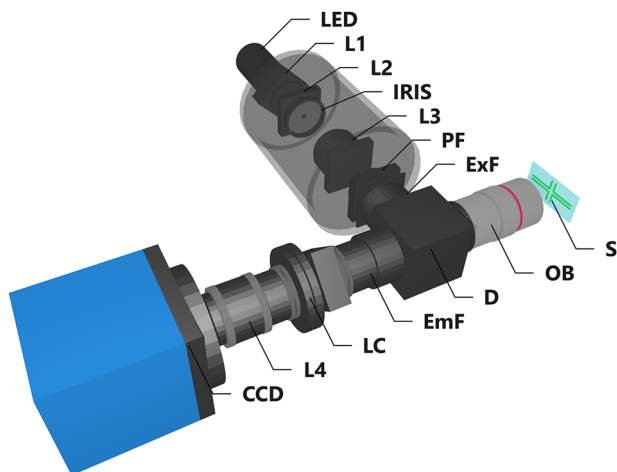
FIG. 1. Schematic illustration of the experimental setup for FP imaging (where L: lens, PF: polarizing filter, ExF: excitation filter, D: dichroic mirror, OB: objective lens, S: sample and EmF: emission filter, respectively).
