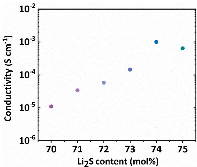
Figure 6 Ionic conductivity of the sulfide solid electrolytes in the x\text{Li}_2\text{S} \cdot 100-x\text{P}_2\text{S}_5 system, obtained by liquid phase and heat treatment at 220 °C.
