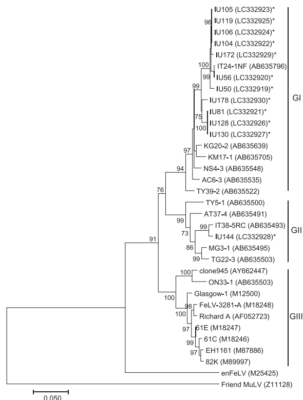
Fig. 1. Phylogenetic tree of env of feline leukemia virus (FeLV). The nucleotide sequences of env were analyzed by using the maximum-likelihood method (MEGA7 software). A bootstrap test was performed with 1000 replicates; bootstrap values >70% are indicated at branches. Reference sequences were obtained from GenBank; accession numbers are shown in parentheses. Asterisk indicates proviruses isolated in the current study. The env sequences were classified into 3 genotypes, as previously reported 21 . A Friend murine leukemia virus env was used as an out-group.
