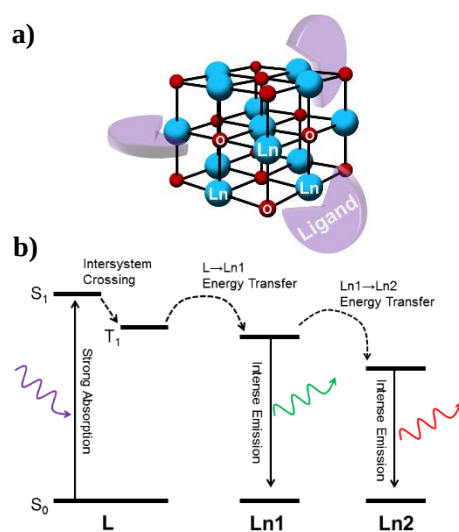
Figure 1 a) Schematic representation of polynuclear Ln clusters, and b) energy diagram depicting luminescence mechanism. L: Ligand, S 0 : singlet ground state, S 1 : singlet excited state, T 1 : triplet excited state.
