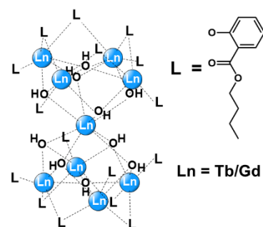
Figure 2 Nonanuclear Tb n Gd 9-n clusters. Ln: Tb or Gd, and L: butyl salicylate ligands.
