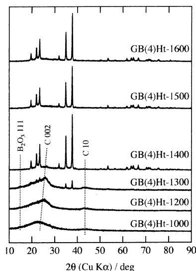
Fig.3 XRD pattern of the products from GB(4)Ht. Diffraction peaks without index are all assigned to \text{B}_4\text{C} (JCPD 35-798).
