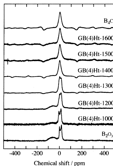
Fig.4 MAS-NMR spectra of the products from GB(4)Ht.
