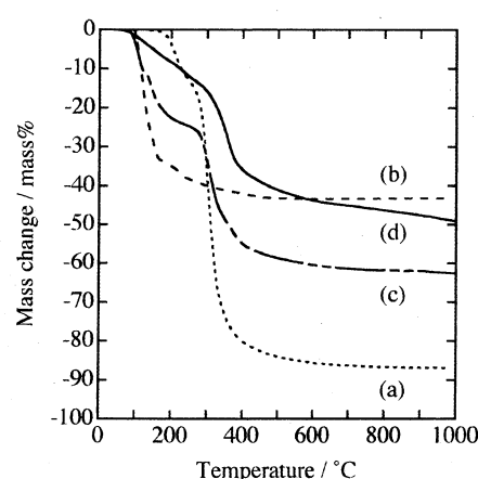
Fig.1 Thermogravimetric curves at 10 K min -1 in pure argon: (a) glucose, (b) boric acid, (c) mixed powder of BA/GL = 2/1, (d) GB(2) (cf. text 2.1.).
