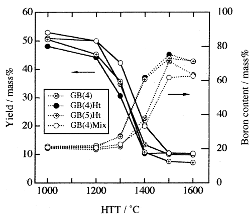
Fig.2 Yield by 1 h heat treatment and boron content of the products from glucose-based precursors.
