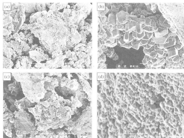
Fig.9 SEM images of the products from CB(4)Ht which were single phase by XRD: (a) (b) CB(4)Ht-1500, and (c) (d) CB(4)Ht-1600. Bars are 10 \mu\text{m} for (a) and (c), and 1 \mu\text{m} for (b) and (d).
