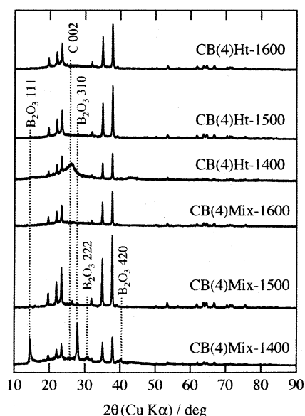
Fig.7 XRD patterns of the products from cellulose-based precursors. Diffraction peaks without index are all assigned to \text{B}_4\text{C} (JCPDS 35-798).
