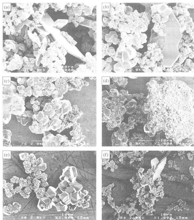
Fig.8 SEM images of the products from glucose-based precursors which were single phase by XRD: (a) GB(4)Ht-1500, (b) GB(4)Ht-1600, (c) GB(4)-1500, (d) GB(4)-1600, (e) GB(5)Ht-1500, and (f) GB(5)Ht-1600. Bars are 10 \mu\text{m} .
