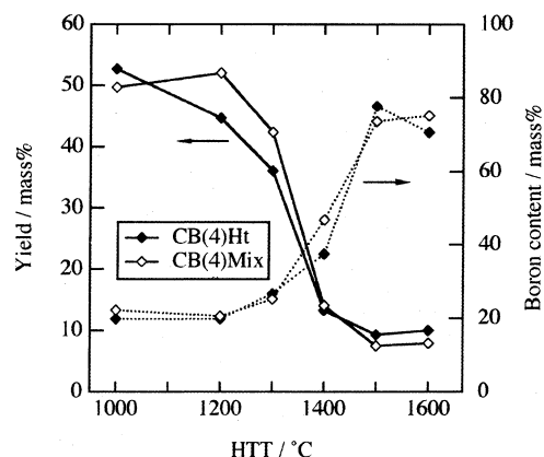
Fig.6 Yield by 1 h heat treatment and boron content of the products from cellulose-based precursors.
