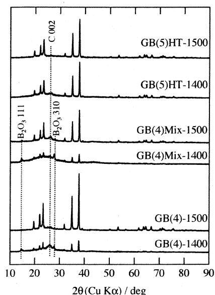
Fig.5 XRD patterns of the products from different precursors. Diffraction peaks without index are all assigned to \text{B}_4\text{C} (JCPDS 35-798).
