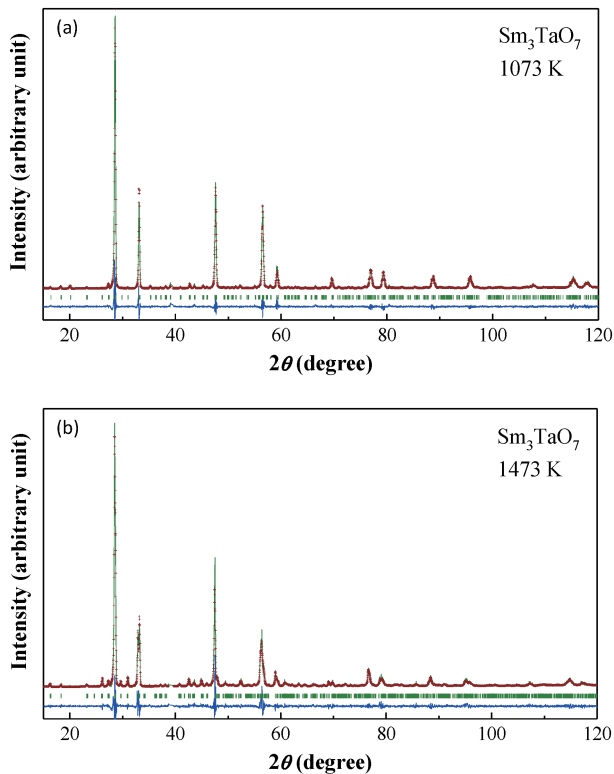
Fig. 3. Powder X-ray diffraction profiles for \text{Sm}_3\text{TaO}_7 measured at (a) 1073 K and (b) 1473 K. The calculated profiles are shown on the top solid line. The vertical marks in the middle show positions calculated for Bragg reflections. The lower trace is a plot of the difference between calculated and observed intensities. Diffraction data 2\theta = 39.14\text{--}39.47^\circ which are ascribed to Pt heater were deleted from the Rietveld analysis.
