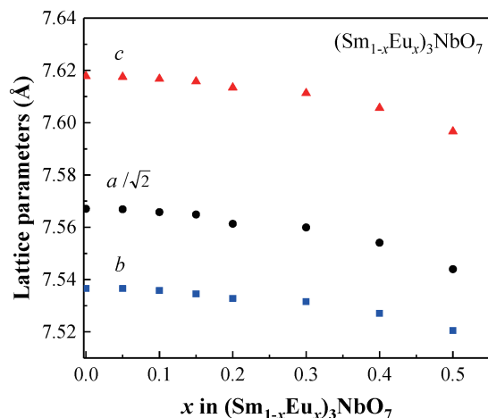
Fig. 5. Variation of lattice parameters for (\text{Sm}_{1-x}\text{Eu}_x)_3\text{NbO}_7 with the ratio of Eu ( x value).
