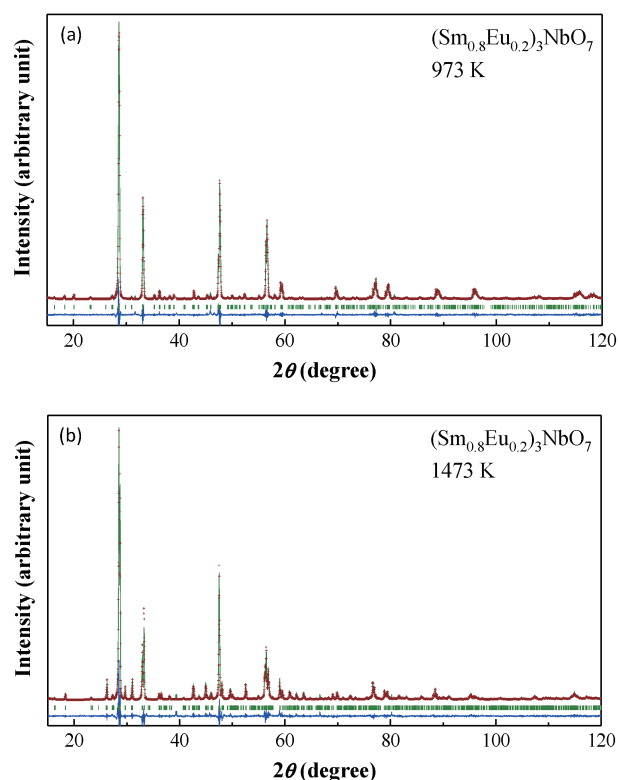
Fig. 8. Powder X-ray diffraction profiles for (\text{Sm}_{0.8}\text{Eu}_{0.2})_3\text{NbO}_7 measured at (a) 973 K and (b) 1473 K. The calculated profiles are shown on the top solid line. The vertical marks in the middle show positions calculated for Bragg reflections. The lower trace is a plot of the difference between calculated and observed intensities. Diffraction data 2\theta = 39.14\text{--}39.47^\circ were deleted from the Rietveld analysis.
