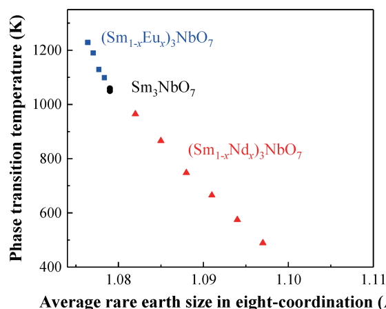
Fig. 13. Variation of phase transition temperatures for (\text{Sm}_{1-x}\text{Ln}_x)_3\text{NbO}_7 ( \text{Ln} = \text{Nd}, \text{Eu} ) against average rare earth size in eight-coordination.
