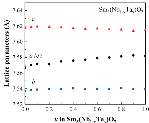
Fig. 1. Variation of lattice parameters for \text{Sm}_3(\text{Nb}_{1-x}\text{Ta}_x)\text{O}_7 with the ratio of Ta ( x value).
