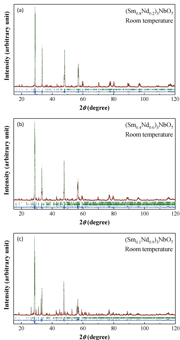
Fig. 9. Powder X-ray diffraction profiles for (a) (\text{Sm}_{0.8}\text{Nd}_{0.2})_3\text{NbO}_7 , (b) (\text{Sm}_{0.4}\text{Nd}_{0.6})_3\text{NbO}_7 , and (c) (\text{Sm}_{0.1}\text{Nd}_{0.9})_3\text{NbO}_7 . The calculated profiles are shown on the top solid line. The vertical marks in the middle show positions calculated for Bragg reflections. The lower trace is a plot of the difference between calculated and observed intensities.
