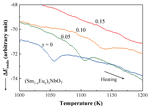
Fig. 6. DTA profiles of \text{Sm}_3\text{NbO}_7 and (\text{Sm}_{1-x}\text{Eu}_x)_3\text{NbO}_7 solid solutions ( x = 0.05, 0.10, 0.15 ) in the temperature range between 1000 and 1200 K. The heating rate is 5 K/min.
