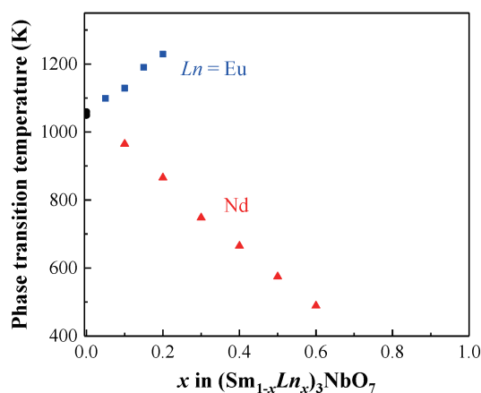
Fig. 7. Variation of phase transition temperatures for (\text{Sm}_{1-x}\text{Ln}_x)_3\text{NbO}_7 ( \text{Ln} = \text{Nd}, \text{Eu} ) with the ratio of Ln ( x value).
