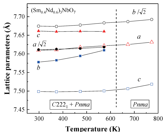
Fig. 12. Variation of lattice parameters for (\text{Sm}_{0.4}\text{Nd}_{0.6})_3\text{NbO}_7 with temperature in the temperature range between 295 and 773 K. Closed symbols are for C222 1 phase and open symbols are for Pnma phase.
