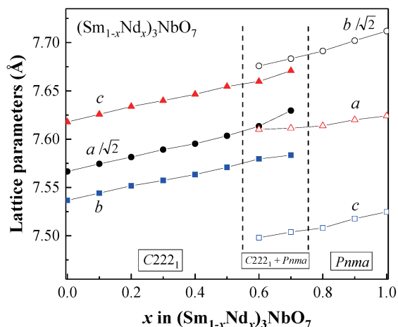
Fig. 10. Variation of lattice parameters for (\text{Sm}_{1-x}\text{Nd}_x)_3\text{NbO}_7 with the ratio of Nd ( x value). Closed symbols are for C222 1 phase and open symbols are for Pnma phase.
