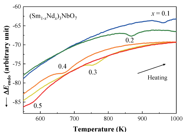
Fig. 11. DTA profiles of (\text{Sm}_{1-x}\text{Nd}_x)_3\text{NbO}_7 solid solutions ( x = 0.1, 0.2, 0.3, 0.4, 0.5 ) in the temperature range between 500 and 1000 K. The heating rate is 5 K/min.
