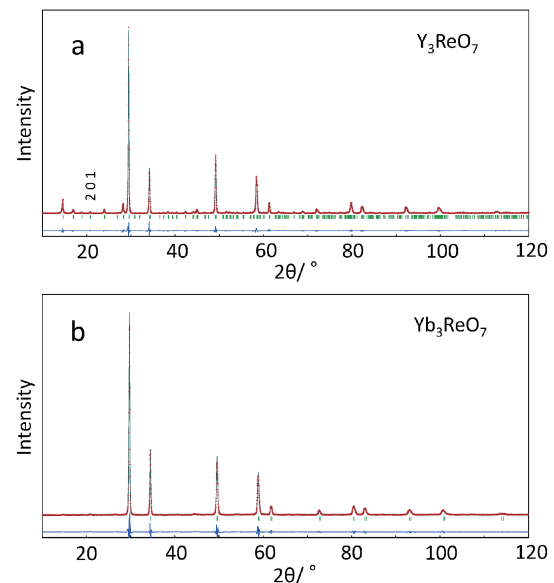
Fig. 1. Powder X-ray diffraction profiles for (a) \text{Y}_3\text{ReO}_7 and (b) \text{Yb}_3\text{ReO}_7 . The calculated and observed profiles are shown on the top solid line and cross markers, respectively. The vertical marks in the middle show positions calculated for Bragg reflections. The lower trace is a plot of the difference between calculated and observed intensities.
