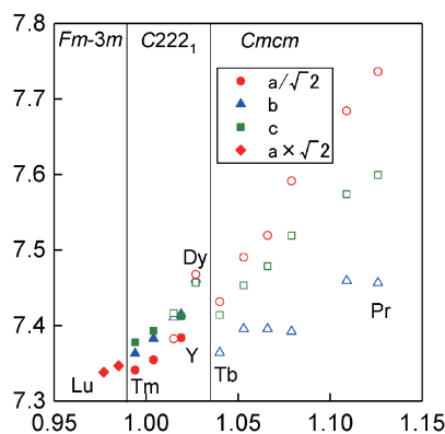
Fig. 3. Variation of lattice parameters for Ln_3ReO_7 with ionic radius of eight-coordinate Ln^{3+} ions. Open symbols correspond to lattice parameters for Ln = Pr, Nd, Sm-Ho compounds with Cmcm or C222_1 space group previously reported.
