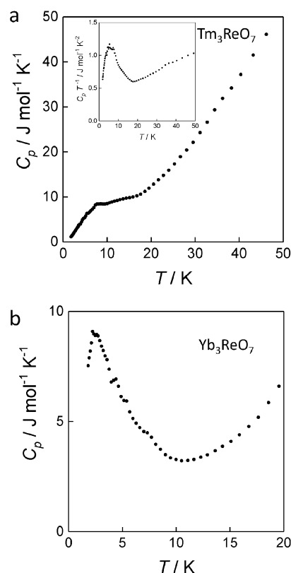
Fig. 6. (a) Temperature dependence of the specific heat ( C_p ) for \text{Tm}_3\text{ReO}_7 below 50 K. The inset shows the specific heat divided by temperature ( C_p/T ). (b) Temperature dependence of the specific heat ( C_p ) for \text{Yb}_3\text{ReO}_7 below 20 K.
