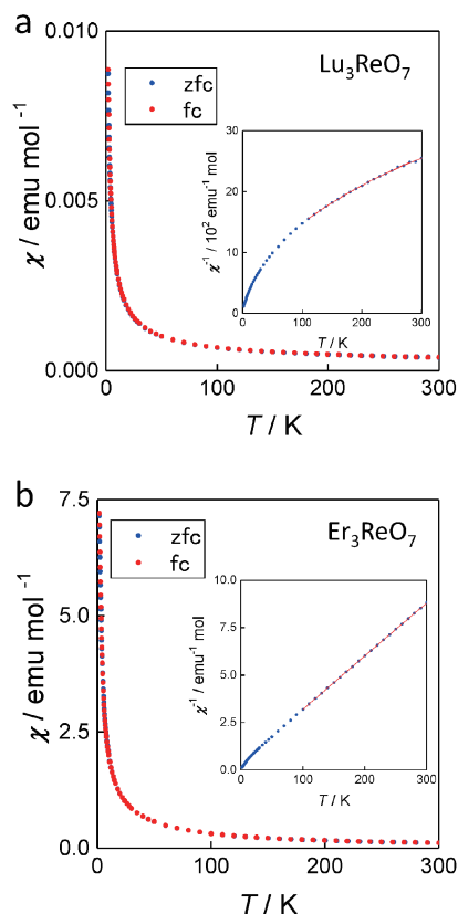
Fig. 5. (a) Temperature dependence of the magnetic susceptibility for \text{Lu}_3\text{ReO}_7 in the temperature range from 1.8 to 300 K. The inset shows the reciprocal susceptibility vs. temperature curve. The red solid line is the Curie–Weiss fitting. (b) Temperature dependence of the magnetic susceptibility for \text{Er}_3\text{ReO}_7 in the temperature range from 1.8 to 300 K. The inset shows the reciprocal susceptibility vs. temperature curve. The red solid line is the Curie–Weiss fitting.
