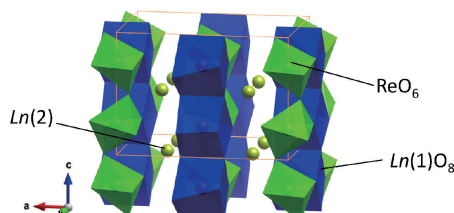
Fig. 2. Schematic crystal structures of Ln_3ReO_7 ( Ln = Y, Dy-Tm , space group: C222_1 ).
