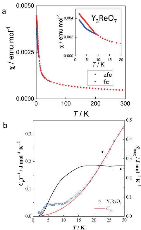
Fig. 4. (a) Temperature dependence of the magnetic susceptibility for Y_3ReO_7 in the temperature range from 1.8 to 300 K. The inset shows the detailed magnetic susceptibility vs. temperature curve below 20 K. (b) Temperature dependence of specific heat divided by temperature ( C_p/T ) and magnetic entropy change ( S_{mag} ) for Y_3ReO_7 below 30 K.
