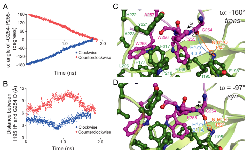
Figure 4. Molecular dynamics simulation of cis/trans isomerization by TF PPD . A, plots of the \omega dihedral angle for the peptidyl-prolyl bond between MBP Gly 254 and Pro 255 . The simulation was started from the NMR structure of MBP-TF PPD complex in which the \omega angle for the peptidyl-prolyl bond between MBP Gly 254 and Pro 255 is -174^\circ ( trans state). Because of the \omega angle constraint at a rate of 0.2^\circ per 2 ps, the \omega angle changed linearly as a function of time. B, plots of the distance between the H N atom of TF Ile 195 and the carbonyl oxygen of MBP Gly 254 as a function of time when the \omega angle was rotated clockwise (blue) or counterclockwise (red). When the \omega angle was rotated in clockwise direction, the two atoms approached each other, and the distance became shorter than 2.5 Å at \sim 0.8 ns. As seen in A, the \omega dihedral angle at 0.8 ns was at approximately -90^\circ ( syn state). C and D, snap shots of the cis/trans isomerization at the trans state (0.200 ns) (C) and the syn state (0.794 ns) (D). The intermolecular hydrogen bond between backbone amide group of TF PPD Ile 195 and the backbone carbonyl oxygen of MBP Gly 254 is formed at the syn state, which tethers the peptidyl-prolyl bond closer onto the hydrophobic cleft formed by TF PPD Ile 195 , Phe 217 , and Pro 218 .
