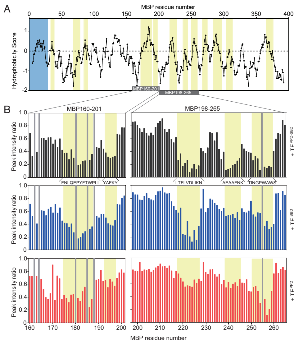
Figure 1. Recognition of unfolded MBP by TF. A, plot of the hydrophobicity score (Roseman algorithm, window = 9) of MBP as a function of its primary sequence. A hydrophobicity score higher than 0 denotes increased hydrophobicity. The regions recognized by TF as identified by NMR titration experiments are highlighted in yellow. The signal sequence is highlighted in blue. The MBP segments depicted in the B are indicated as a gray bar. B, plots of peak intensity change of MBP160–201 (left panels) and MBP198–265 (right panels) by the addition of TF PPD-SBD at a ratio of MBP:TF PPD-SBD 1:0.1 (top panels), TF SBD at a ratio of MBP:TF SBD 1:0.2 (middle panels), and TF PPD at a ratio of MBP:TF PPD 1:0.5 (bottom panels), as a function of the primary sequences of the MBP peptides. The regions recognized by TF are highlighted in yellow and labeled with the primary sequences. The proline residue and unassigned residue are indicated by gray bar.
