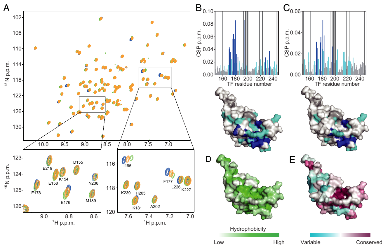
Figure 2. The substrate-binding sites on TF PPD . A, ^1\text{H} - ^{15}\text{N} HSQC spectra of TF PPD in the absence (blue) and presence of MBP160–201 (green) or MBP198–265 (orange). The spectra were recorded with several titration points, TF PPD :MBP 1:0.1, 1:0.2, 1:0.5, 1:1, and 1:2, but only the spectra at 1:2 ratio are shown for clarity. The regions indicated by boxes in the top panel are expanded in the bottom panels with resonance assignments. B and C, chemical shift perturbations of amide moieties of TF PPD upon binding to MBP160–201 (B) or MBP198–265 (C), plotted as a function of the residue number of TF PPD . Proline and unassigned residues are indicated by bars colored dark gray. The lower panels show chemical shift perturbation mapping on the structure of TF PPD (PDB code 1W26). The residues with perturbations larger than the threshold values of 0.015 and 0.025 ppm are colored light blue and dark blue, respectively. Proline and unassigned residues are colored dark gray. D, mapping of the hydrophobicity on the structure of TF PPD . E, TF PPD sequence conservation mapped on the structure of TF PPD .
