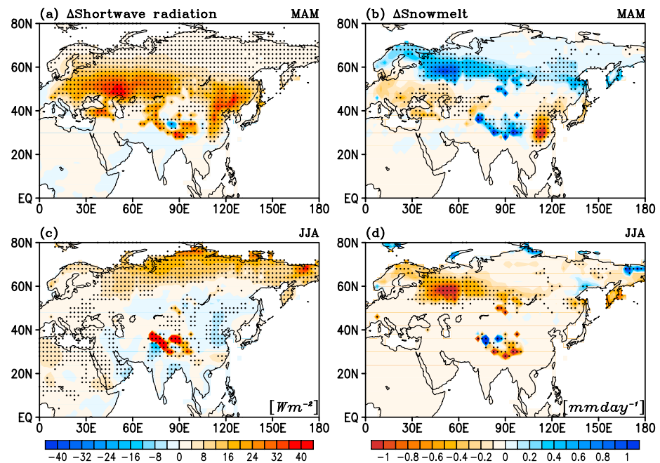
Figure 4. Spatial distributions of SDE-induced anomalies in (a) surface shortwave radiation ( Wm^{-2} ) and (b) snowmelt ( mm day^{-1} ) during MAM. (c and d) The same as (a) and (b), respectively, except for JJA. Dots represent statistical significance at 95% confidence level.
