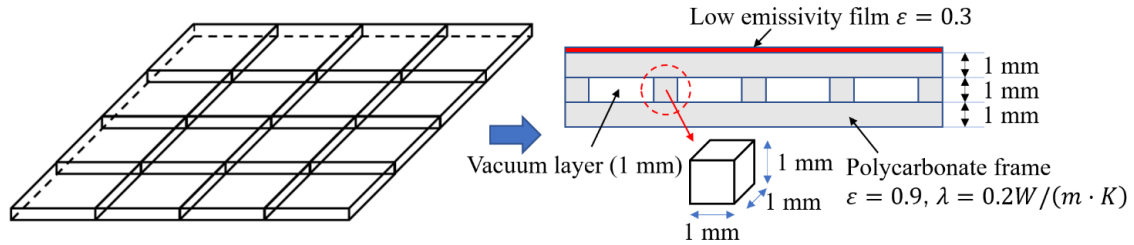
Figure 4-21 Concept diagram of the VIP specimen and model for the case study
