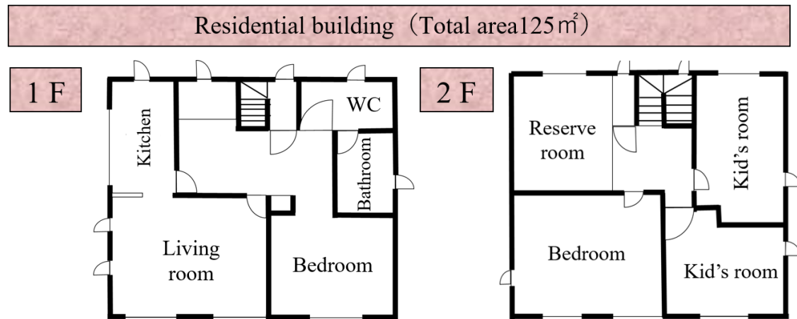
Figure 6-20 Building outline
