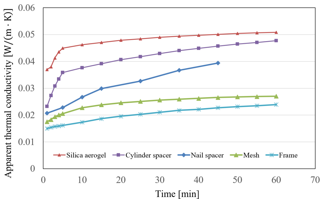
Figure 5-13 Measured apparent thermal conductivity according to elapsed time. Also, the trial production of VIP and measurement of thermal conductivity is carried
