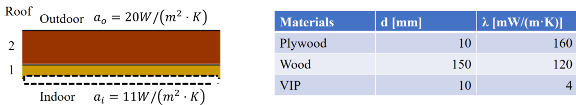
Figure 6-19 Roof conditions
