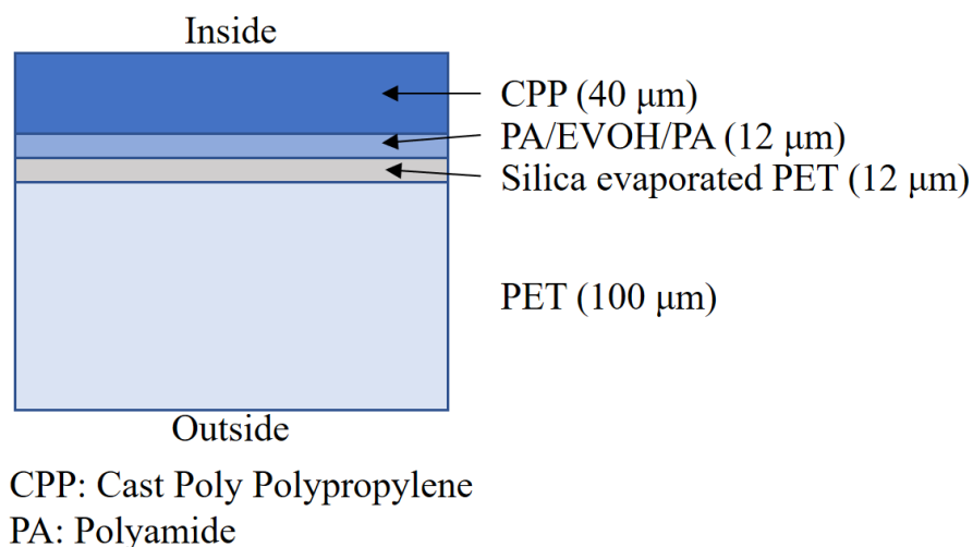
Figure 4-18 Component diagram of the gas barrier film
