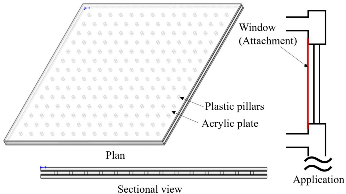
Figure 1-5 Concept diagram of the VIP application to buildings
