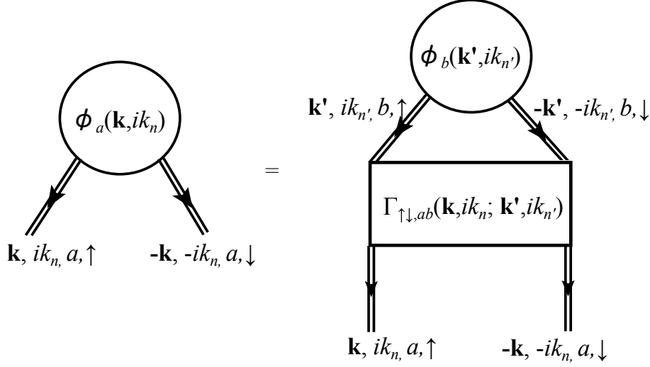
Figure 26: Diagrammatic representation of the linearized gap equation. The circle is the pairing gap function and the box is the pairing interaction; the arrowed double line is the full Green's function.
