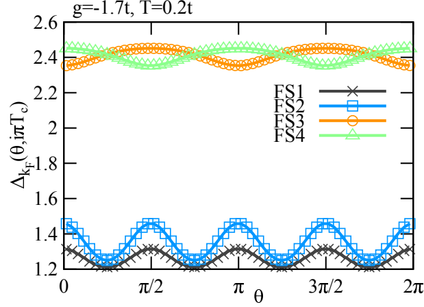
Figure 71: Momentum dependence of the pairing gap due to orbital nematic fluctuations without the self-energy effect ( g/t = -1.7 ).
