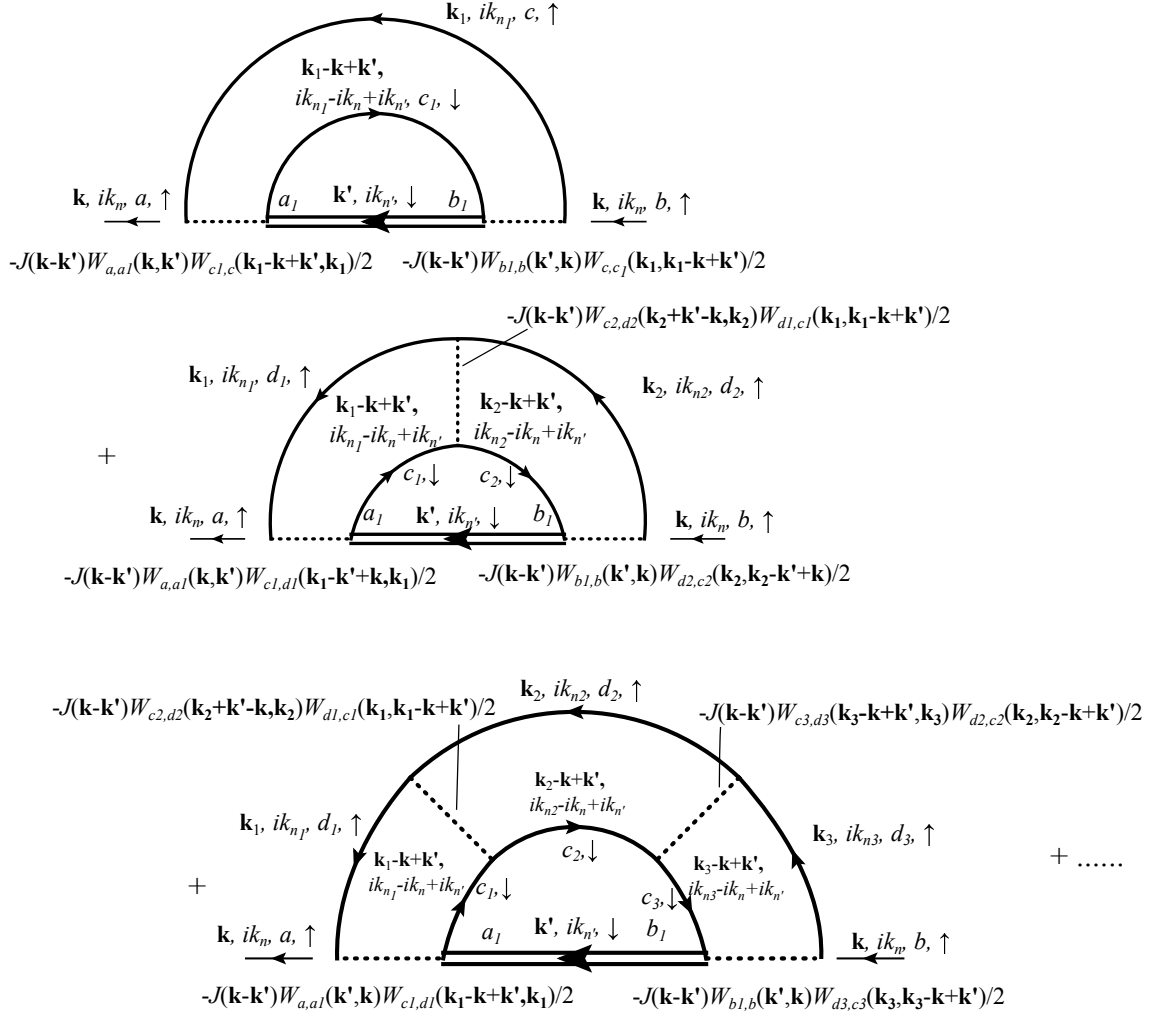
Figure 25: Self-energy due to the transverse spin interaction. The curves with an arrow are the bare Green's functions, and the dotted lines are the bare transverse spin interactions (see Fig.22). The double lines with an arrow are the full Green's functions of electrons.
