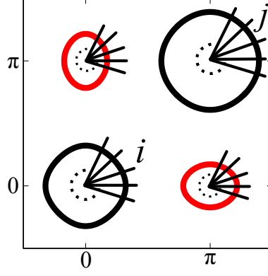
Figure 27: Fermi surfaces in the first quadrant of the first Brillouin zone. Each Fermi pocket is divided into small segments to include the momentum dependence of \Delta_a(\mathbf{k}, ik_n) and Z_a(\mathbf{k}, ik_n) .
