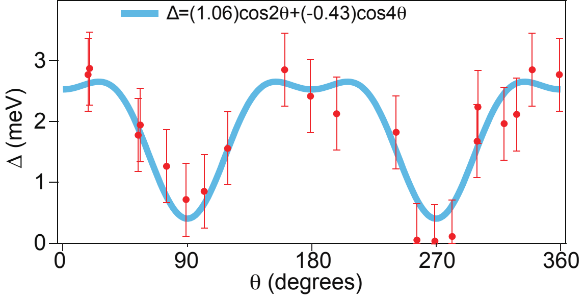
Figure 65: Pairing gap observed on a hole pocket in \text{FeSe}_{0.93}\text{S}_{0.07} [52] (Red filled circles). The horizontal axis \theta is an angle measured by k_x axis. The blue curve is fitted line of the gap.
