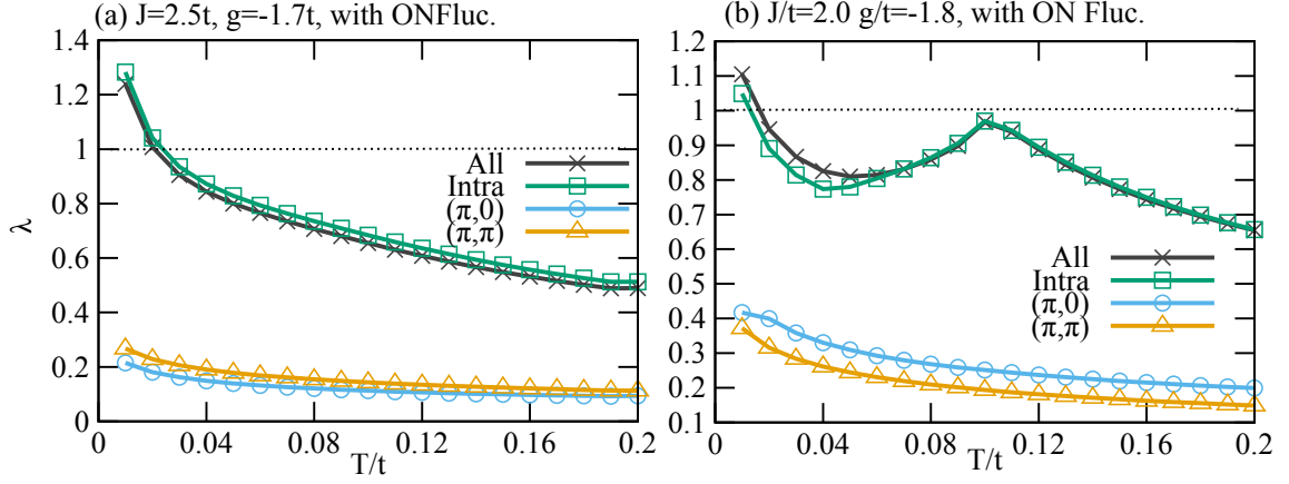
Figure 51: Temperature dependence of the eigenvalues of the Eliashberg equations due to both orbital nematic and Lorentz-type spin fluctuations (a) in the tetragonal phase ( J/t = 2.5, g/t = -1.7 ) and (b) in the nematic phase ( J/t = 2.0, g/t = -1.8 ). The eigenvalues are also computed by selecting specific scattering processes, “Intra”, “ (\pi, 0) ” and “ (\pi, \pi) ”; see Fig.33.
