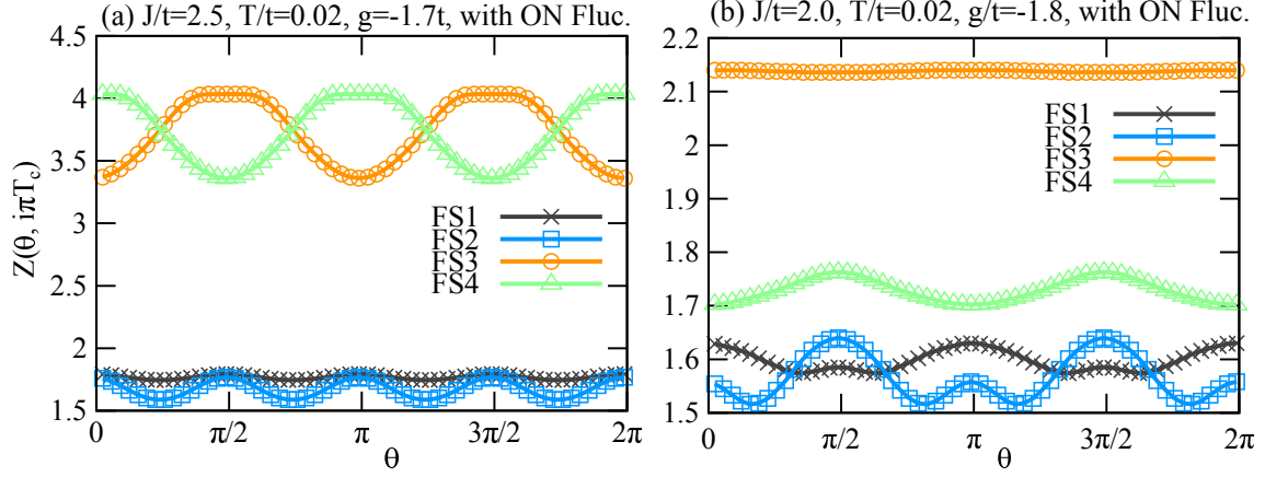
Figure 53: Momentum dependence of the renormalization function at T = T_c in the presence of both orbital nematic and Lorentz-type spin fluctuations (a) in the tetragonal phase ( J/t = 2.5, g/t = -1.7 ) and (b) in the nematic phase ( J/t = 2.0, g/t = -1.8 ).
