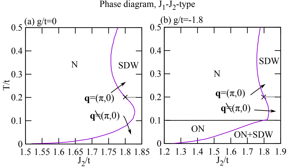
Figure 45: Magnetic phase diagram due to the J_1 - J_2 -type spin fluctuations (a) in the absence of the nematic order ( g/t = 0 ) and (b) in the presence of the nematic order at low temperature ( g/t = -1.8 ). “N” stands for the normal metallic (tetragonal) phase and the SDW phase can be characterized by the momentum slightly far away from \mathbf{q} = (\pi, 0) below the temperature marked by cross. Black solid line denotes the orbital nematic transition at T_{\text{ON}} \simeq 0.10t .
