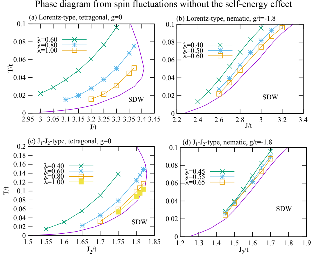
Figure 75: Phase diagram in the plane of the strength of the spin interaction and temperature in the absence of the self-energy effect for the Lorentz-type spin fluctuations (a) in the tetragonal phase and (b) in the nematic phase. Contour lines of the largest eigenvalue of the Eliashberg equations are plotted near the SDW phase. (c) and (d) corresponding results for the J_1 - J_2 -type spin fluctuations.
