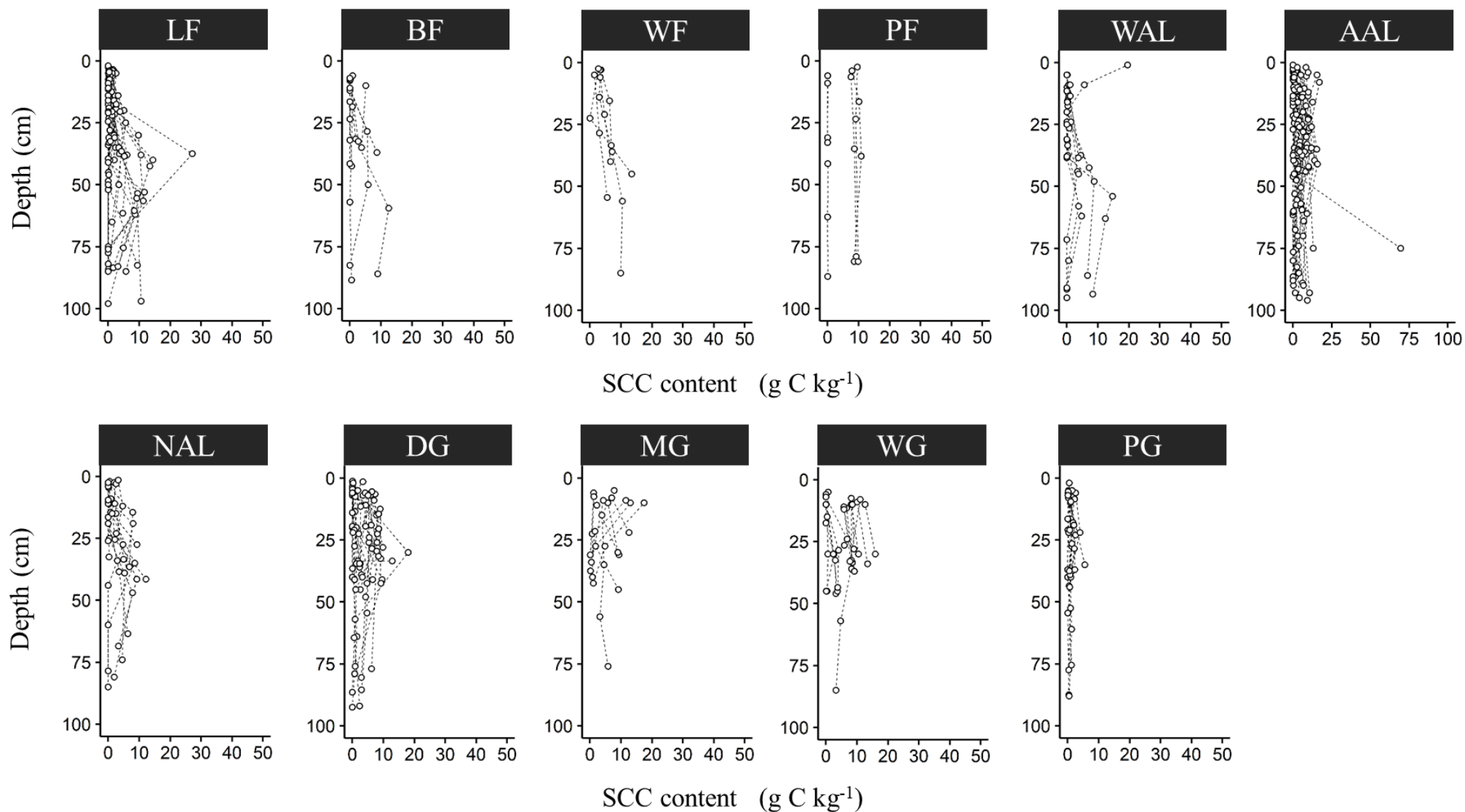
Fig. 6.3. Vertical distribution of soil carbonate carbon content. SCC: Soil carbonate carbon, LF: Larch forest, BF: Burned larch forest, WF: Water damaged larch forest, PF: Pine forest, WAL: Working arable land, AAL: Abandoned arable land, NAL: Abandoned arable land invaded by new-growing trees, DG: Dry grassland, MG: Moderately wet grassland, WG: Wet grassland, PG: Pingo.
