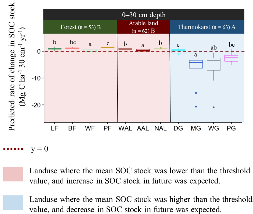
Fig. 6.14. Predicted rate of change in soil organic carbon (SOC) stock in Central Yakutia. Box plots visualize the five-number summary of a data set (minimum, lower quartile, median, upper quartile and maximum) and points indicate outlier value. Different uppercase letters indicate significant differences between ecosystems, and different lowercase letters indicate significant differences between land use types in the same ecosystem. SOC: Soil organic carbon, LF: Larch forest, BF: Burned larch forest, WF: Water damaged larch forest, PF: Pine forest, WAL: Working arable land, AAL: Abandoned arable land, NAL: Abandoned arable land invaded by new-growing trees, DG: Dry grassland, MG: Moderately wet grassland, WG: Wet grassland, PG: Pingo.
