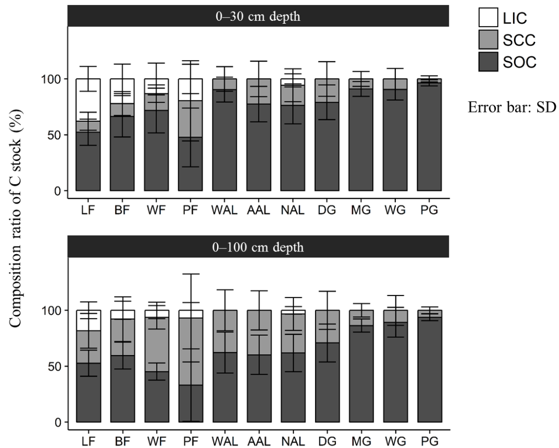
Fig. 6.7. Composition ratio of carbon stocks in the 0–30 and 0–100 cm soil layers. LIC: Litter carbon, SOC: Soil organic carbon, SCC: Soil carbonate carbon, LF: Larch forest, BF: Burned larch forest, WF: Water damaged larch forest, PF: Pine forest, WAL: Working arable land, AAL: Abandoned arable land, NAL: Abandoned arable land invaded by new-growing trees, DG: Dry grassland, MG: Moderately wet grassland, WG: Wet grassland, PG: Pingo
