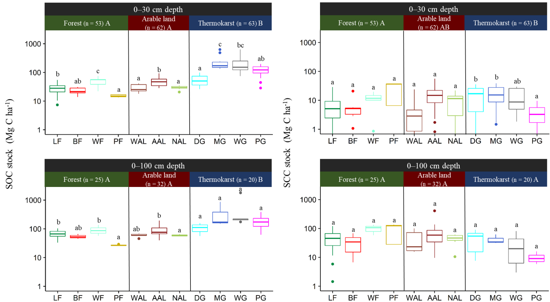
Fig. 6.4. Soil organic carbon and soil carbonate carbon stocks in the 0–30 and 0–100 cm soil layers. Box plots visualize the five-number summary of a data set (minimum, lower quartile, median, upper quartile and maximum) and points indicate outlier value. Different uppercase letters indicate significant differences between ecosystems, and different lowercase letters indicate significant differences between land use types in the same ecosystem. SOC: Soil organic carbon, SCC: Soil carbonate carbon, LF: Larch forest, BF: Burned larch forest, WF: Water damaged larch forest, PF: Pine forest, WAL: Working arable land, AAL: Abandoned arable land, NAL: Abandoned arable land invaded by new-growing trees, DG: Dry grassland, MG: Moderately wet grassland, WG: Wet grassland, PG: Pingo.
