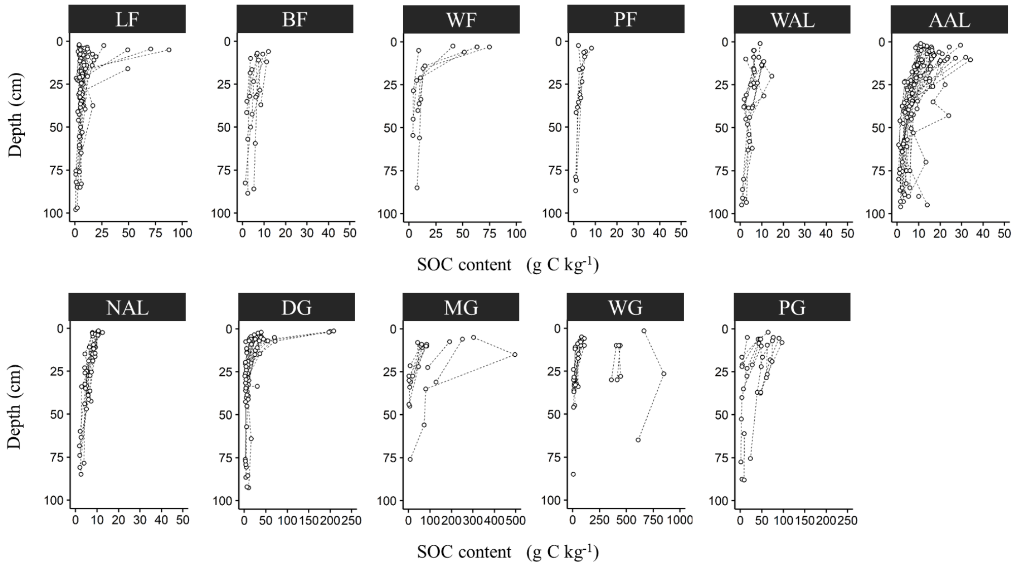
Fig. 6.2. Vertical distribution of soil organic carbon content. SOC: Soil organic carbon, LF: Larch forest, BF: Burned larch forest, WF: Water damaged larch forest, PF: Pine forest, WAL: Working arable land, AAL: Abandoned arable land, NAL: Abandoned arable land invaded by new-growing trees, DG: Dry grassland, MG: Moderately wet grassland, WG: Wet grassland, PG: Pingo.
