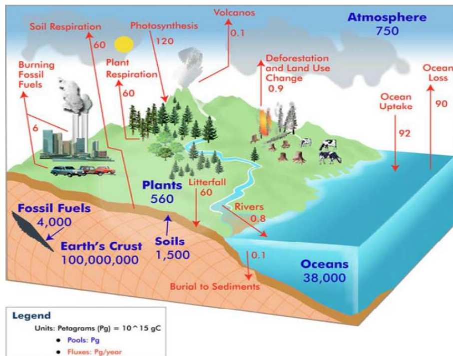
Fig. 1.1. The global carbon cycle showing carbon stocks in blue (in Pg C = Gt C) and carbon fluxes in red (in Gt C yr -1 ) (Conijn and Lesschen, 2015).
