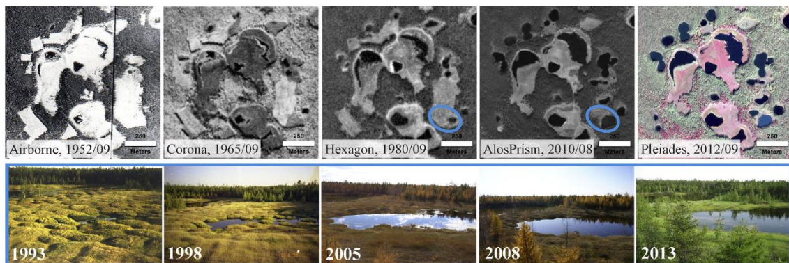
Fig. 2.6. Landscape change at Yukechi alas during recent years. Several thermokarst lakes around the Yukechi alas have developed rapidly in areas ploughed until the 1950s. The blue ellipse in the upper satellite image time series marks the view of the photographs below (Crate et al., 2017).
