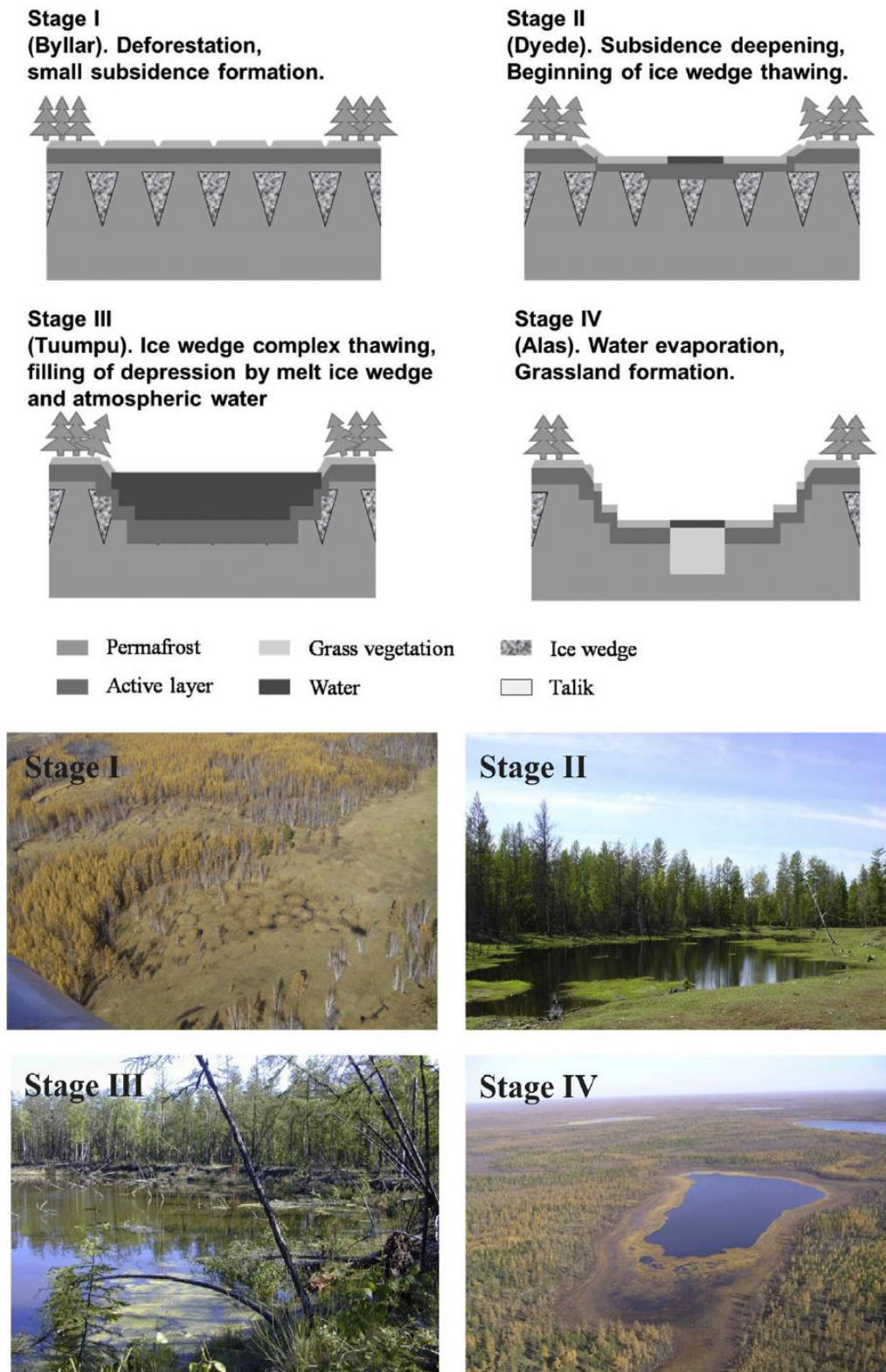
Fig. 2.4. Thermokarst stages in ice-rich permafrost in the boreal zone of Central Yakutia. For each stage corresponding pictures are shown below ( Crate et al., 2017 ).
