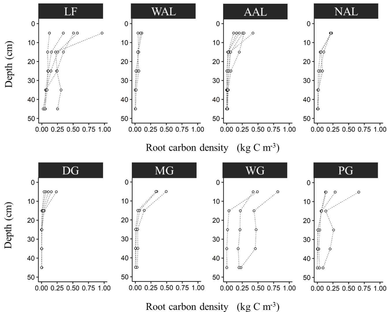
Fig. 6.9. Vertical distribution of root carbon density. LF: Larch forest, WAL: Working arable land, AAL: Abandoned arable land, NAL: Abandoned arable land invaded by new-growing trees, DG: Dry grassland, MG: Moderately wet grassland, WG: Wet grassland, PG: Pingo.
