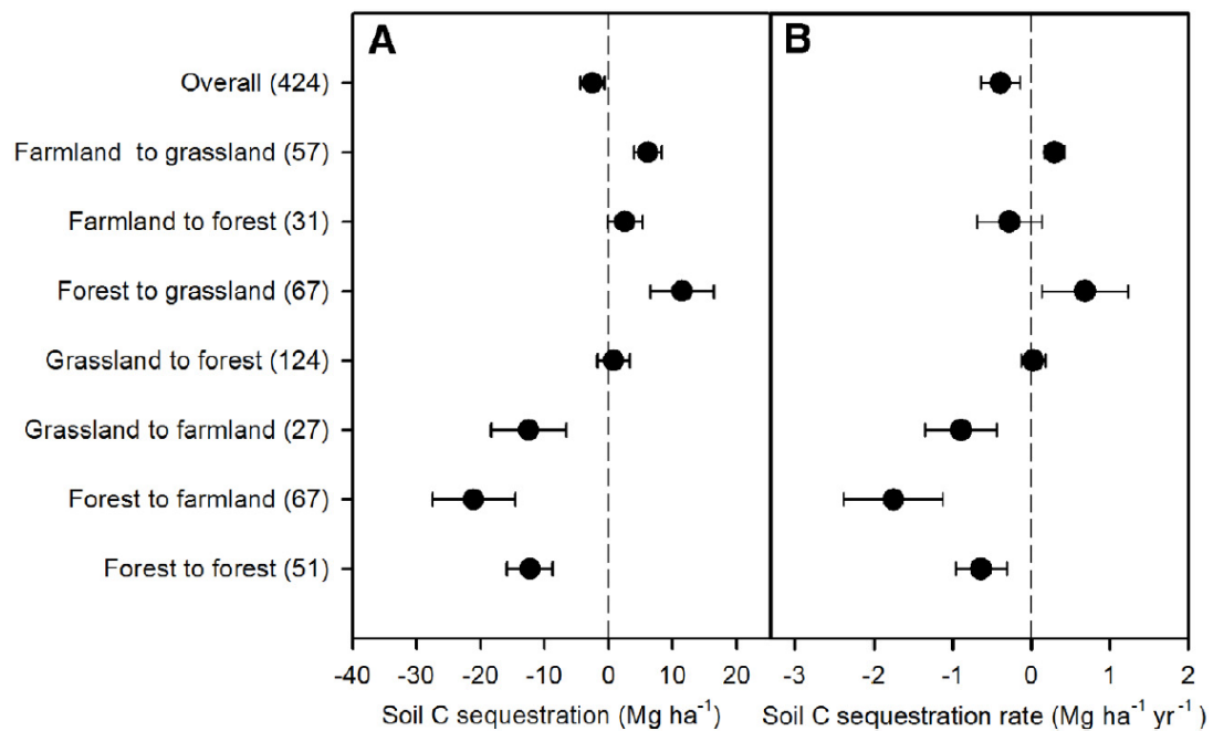
Fig. 2.2. The effects of the land use changes on soil C sequestration and soil C sequestration rate. Dots with error bars denote the overall mean values and the 95% confidence interval, and numbers of observations are in the parenthesis. The dash line indicates x = 0 (Deng et al., 2016).
