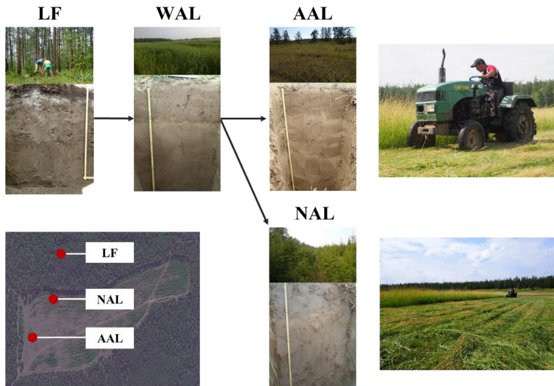
Fig. 3.5. Typical land uses in the arable land ecosystem. LF: Larch forest, WAL: Working arable land, AAL: Abandoned arable land, NAL: Abandoned arable land invaded by new-growing trees
