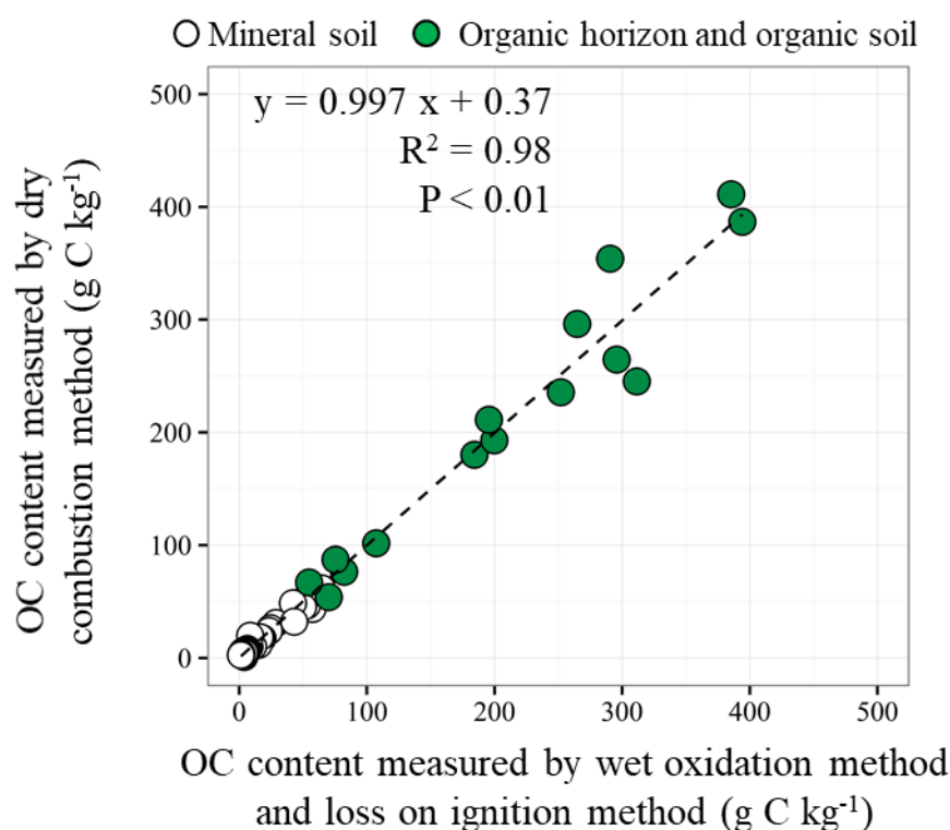
Fig. 5.2. Comparison of the organic carbon content between the methodologies. OC; Organic carbon. OC content measured by the loss on ignition method was modified by using Eq.3.1. OC content measured by the dry combustion method was determined from the difference between total carbon content (TC) and carbonate carbon (CC) content.
