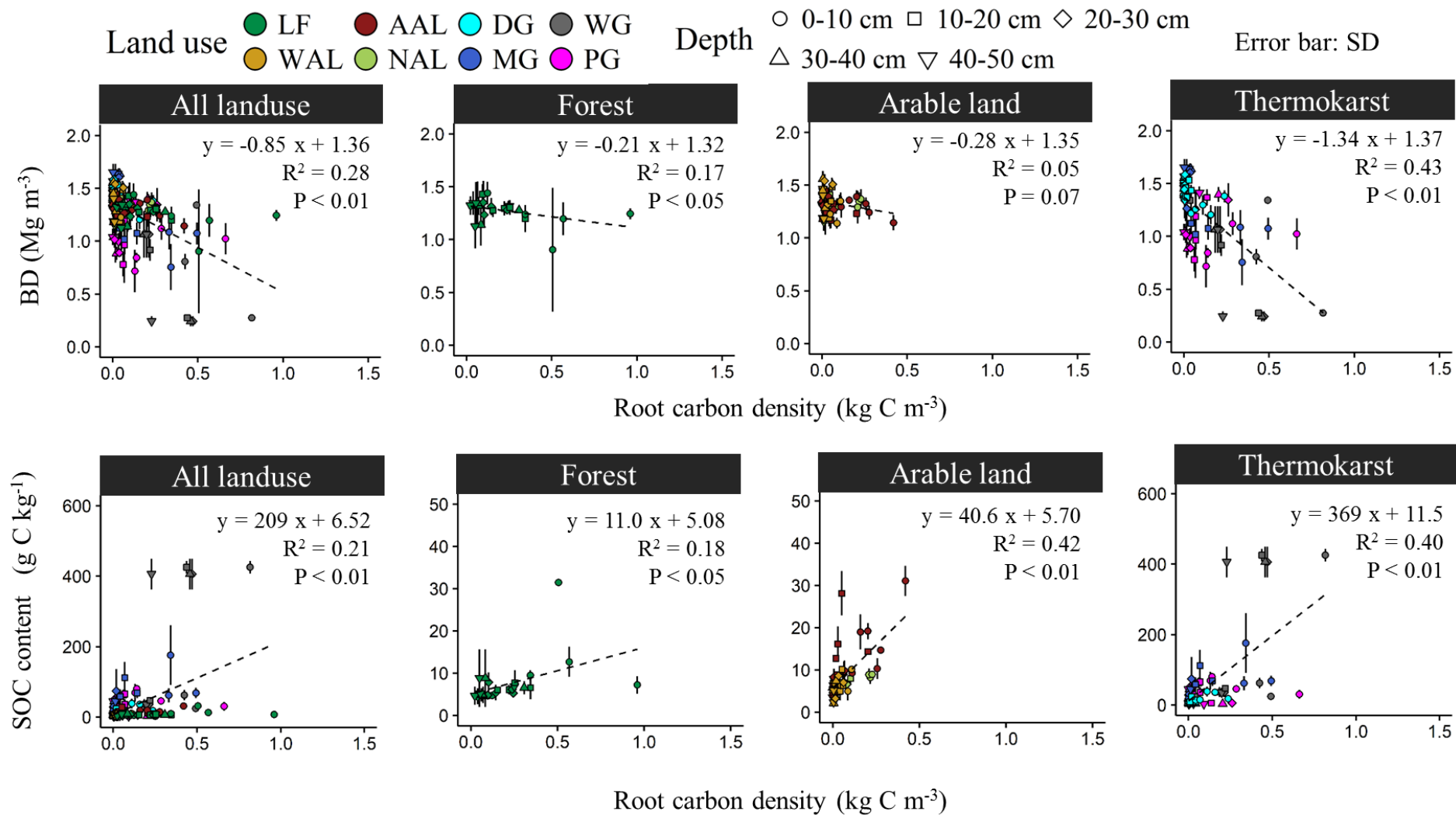
Fig. 6.11. Relationships between root carbon density and bulk density and between root carbon density and the soil organic carbon content. SOC: Soil organic carbon, BD: Bulk density. LF: Larch forest, WAL: Working arable land, AAL: Abandoned arable land, NAL: Abandoned arable land invaded by new-growing trees, DG: Dry grassland, MG: Moderately wet grassland, WG: wet grassland, PG: Pingo.
