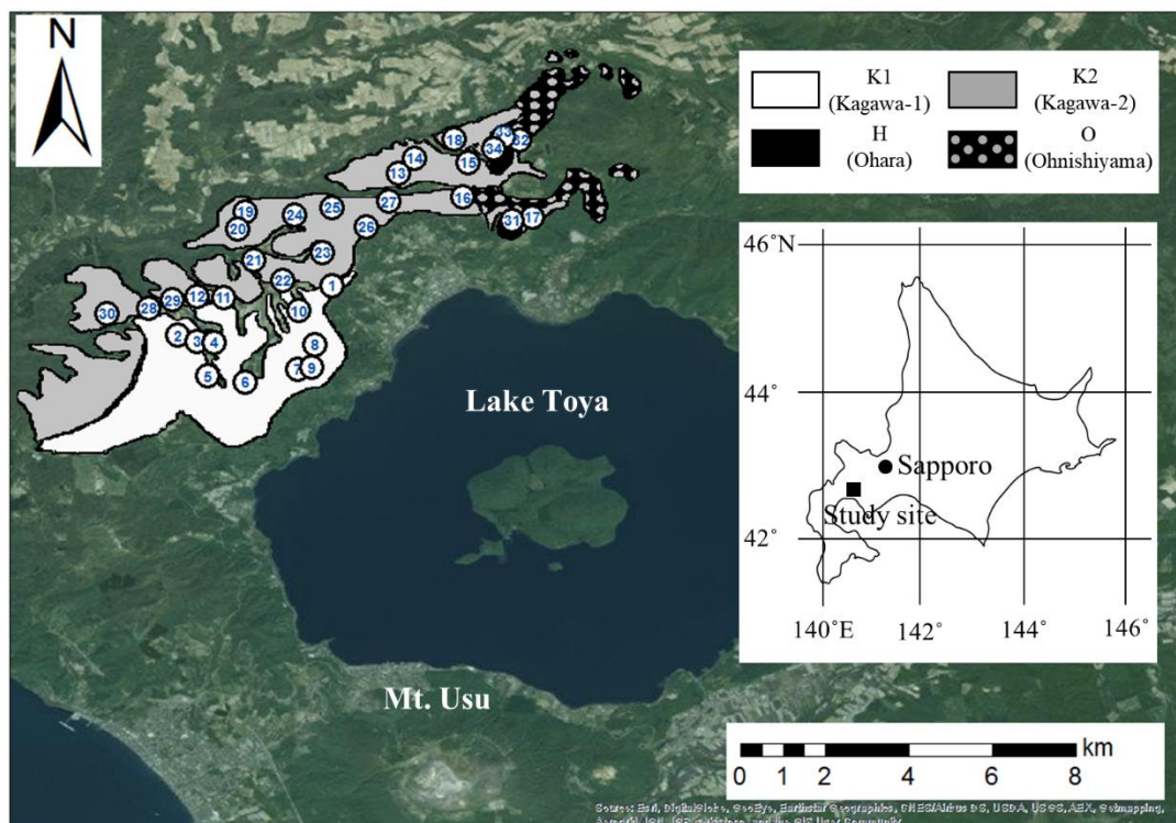
Fig. 4.1. Distribution of the soil series and location of the study fields.
