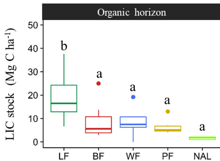
Fig. 6.5. Litter carbon stock in the organic horizon. Box plots visualize the five-number summary of a data set (minimum, lower quartile, median, upper quartile and maximum) and points indicate outlier value. Different lowercase letters indicate significant differences between land use types. LIC: Litter carbon, LF: Larch forest, BF: Burned larch forest, WF: Water damaged larch forest, PF: Pine forest, NAL: Abandoned arable land invaded by new-growing trees.
