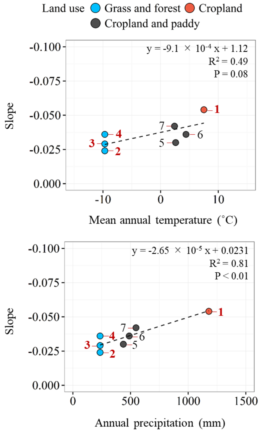
Fig. 7.1 The relationship between climate condition and the slope of the regression equation between initial soil organic carbon (SOC) stock and rate of change ( \Delta ) in SOC stock. 1: Cropland (Chapter 4), 2, 3, and 4: Grassland and forest (Chapter 5), 5, 6, and 7; Cropland and paddy (Li et al., 2016).
