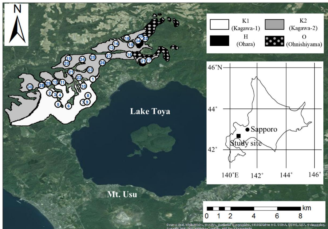
Fig. 3.2. Distribution of the soil series and location of the study fields in Toya region.
