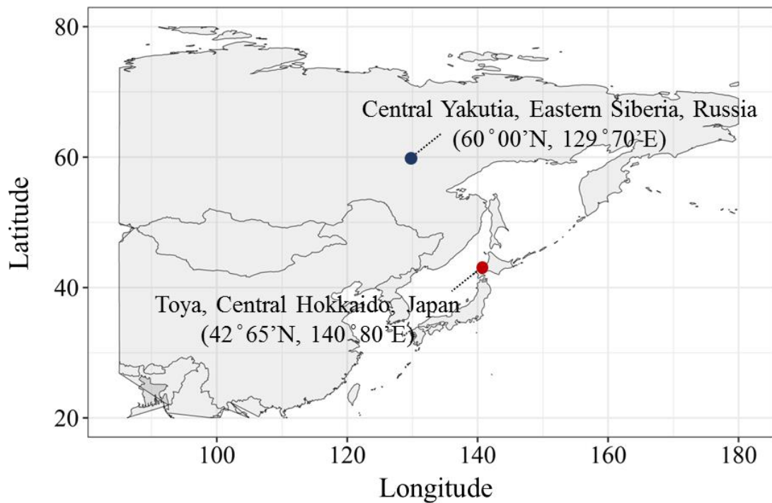
Fig. 3.1. Map of the research sites.
