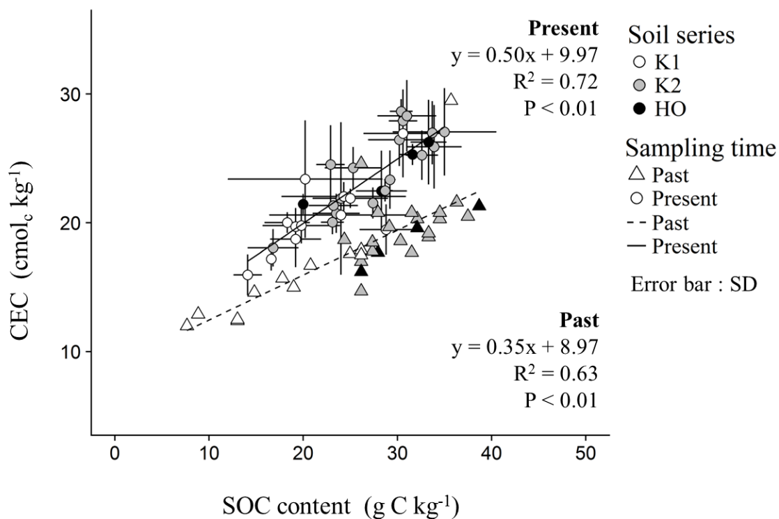
Fig. 4.4. Relationship between soil organic carbon (SOC) content and cation exchange capacity (CEC). Present: 2012, Past: 2001–2003.
