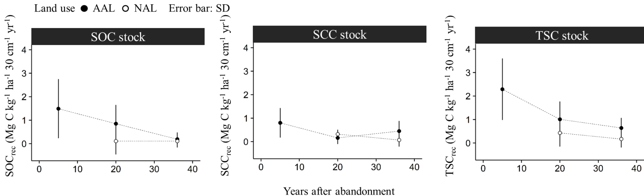
Fig. 6.12. Annual average carbon recovery rate on abandoned arable land and new-growth arable land after abandonment. \text{SOC}_{\text{rec}} : annual average rate of soil organic carbon stock recovery after the abandonment of working arable land. \text{SCC}_{\text{rec}} : annual average rate of soil carbonate carbon stock recovery after the abandonment of working arable land. \text{TSC}_{\text{rec}} : annual average rate of soil total carbon stock recovery after the abandonment of working arable land. \text{SOC}_{\text{rec}} , \text{SCC}_{\text{rec}} , and \text{TSC}_{\text{rec}} were calculated based on Kurganova et al. (2014) . AAL: Abandoned arable land, NAL: Abandoned arable land invaded by new-growing trees.
