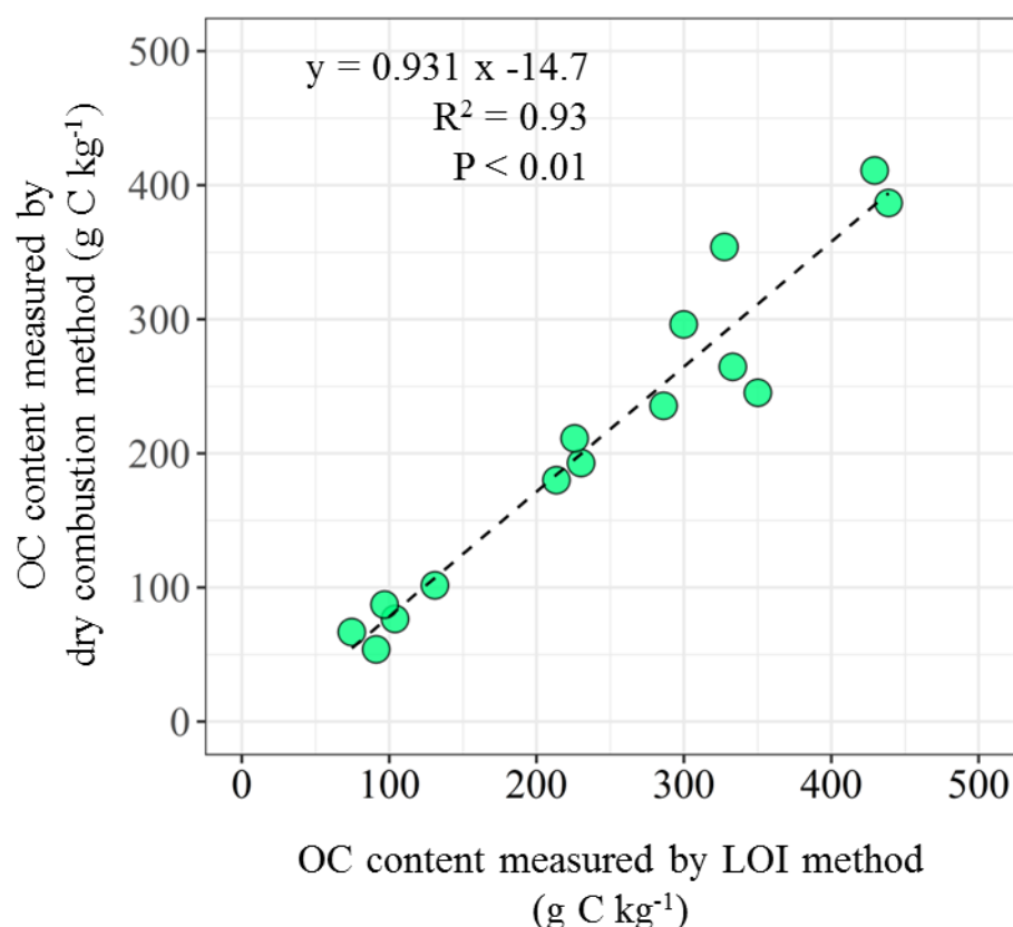
Fig. 3.7. The relationship between the organic carbon content measured by loss on ignition method and by dry combustion method. OC: Organic carbon, LOI: Loss on ignition.
