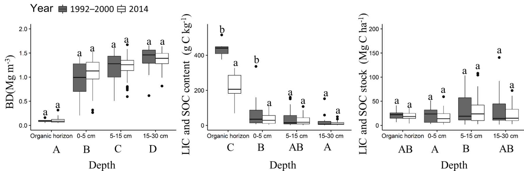
Fig. 5.3. Comparison of bulk density, carbon content, and carbon stock between 1992–2000 and 2014 at each depth. Different lower-case letters indicate significant differences between 1992–2000 and 2014. Different capital letters indicate significant differences between depths. SOC: Soil organic carbon, LIC: Litter carbon.
