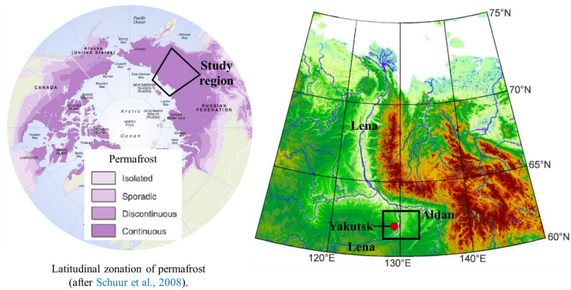
Fig. 3.3. Location of the study site in Eastern Siberia adapted from ( http://www.ipf.tuwien.ac.at/permafrost/ ).
