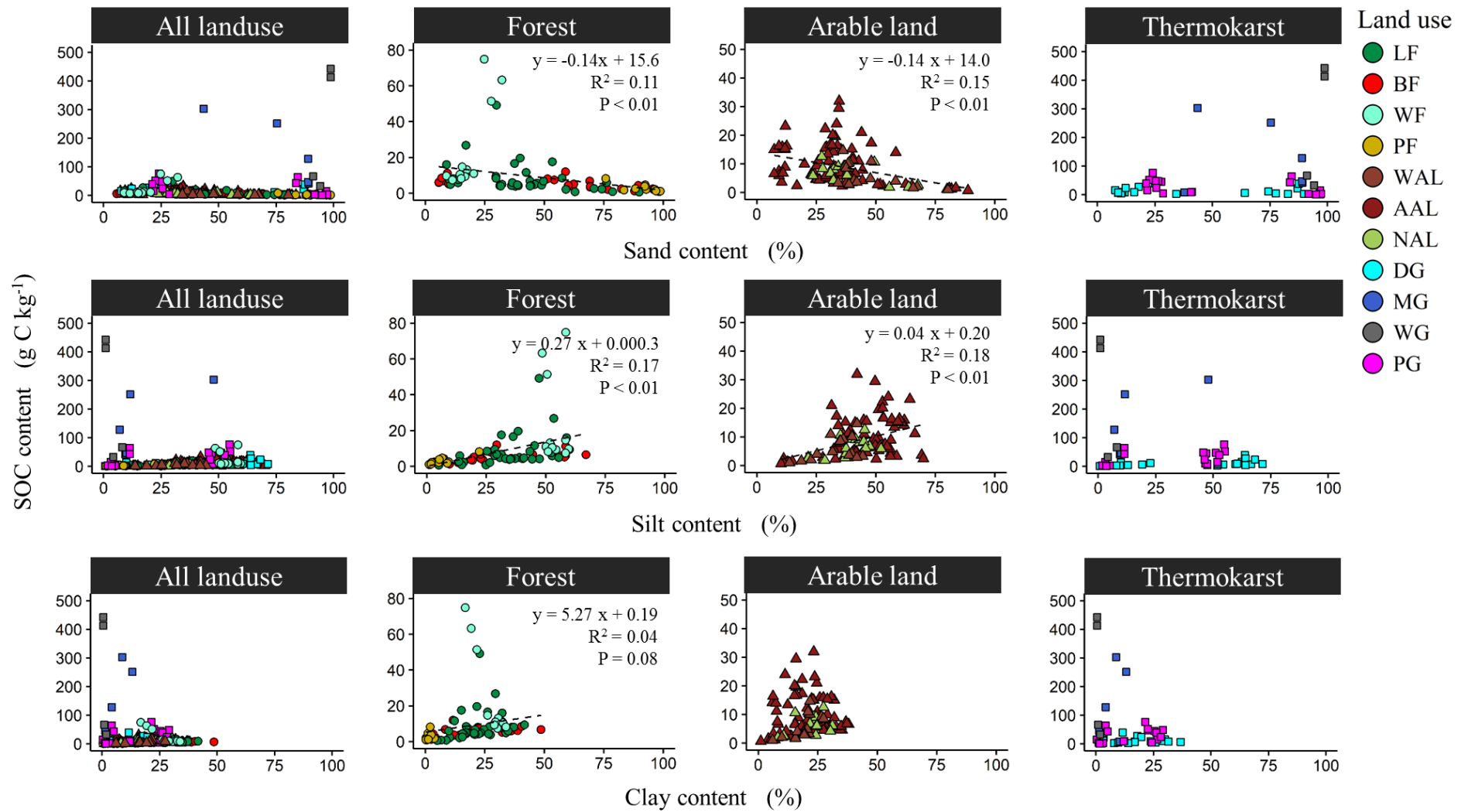
Fig. 6.15. The relationship between the soil texture and soil organic carbon (SOC) content. SOC: Soil organic carbon, LF: Larch forest, BF: Burned larch forest, WF: Water damaged larch forest, PF: Pine forest, WAL: Working arable land, AAL: Abandoned arable land, NAL: Abandoned arable land invaded by new-growing trees, DG: Dry grassland, MG: Moderately wet grassland, WG: Wet grassland, PG: Pingo.
