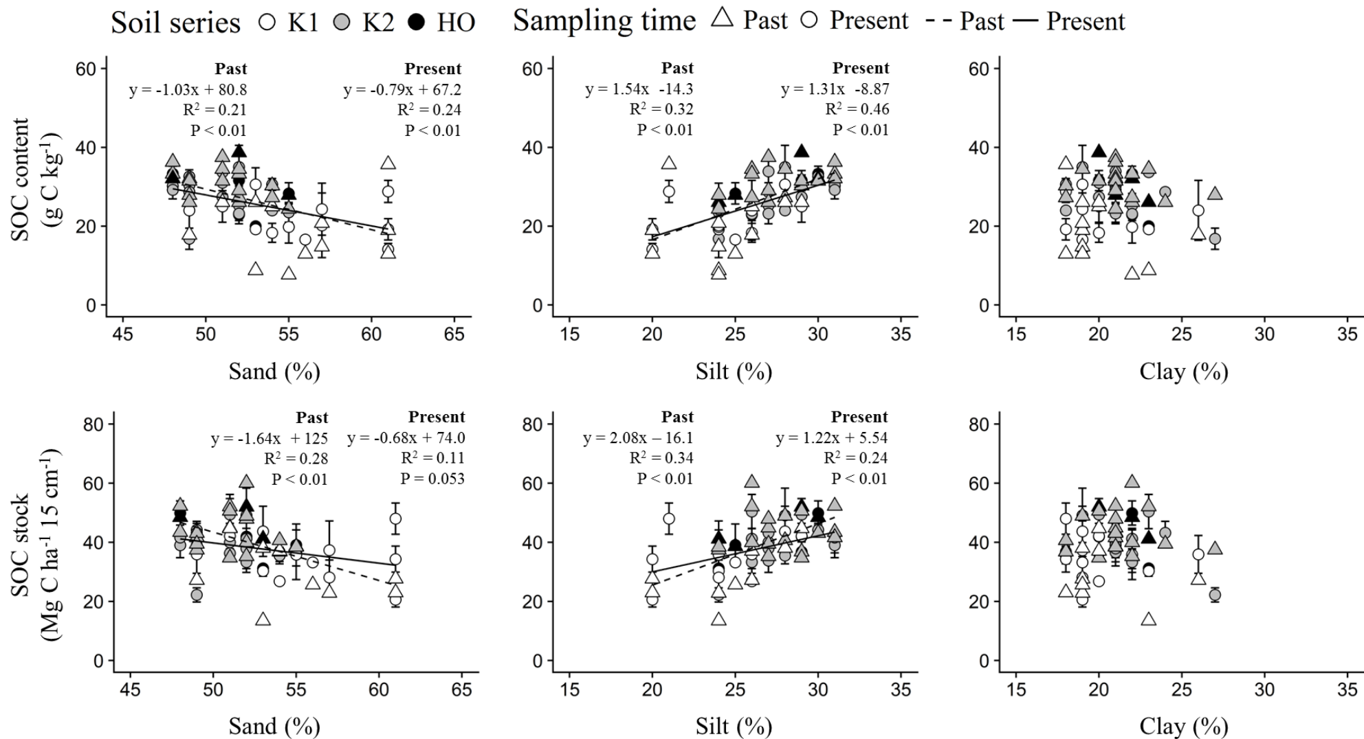
Fig. 4.2. Relationship between soil texture and soil organic carbon (SOC). Present: 2012; Past, 2001–2003.
