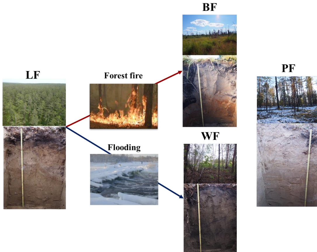
Fig. 3.4. Typical land uses in the forest ecosystem. LF: Larch forest, BF: Burned larch forest, WF: Water damaged larch forest, PF: Pine forest.
