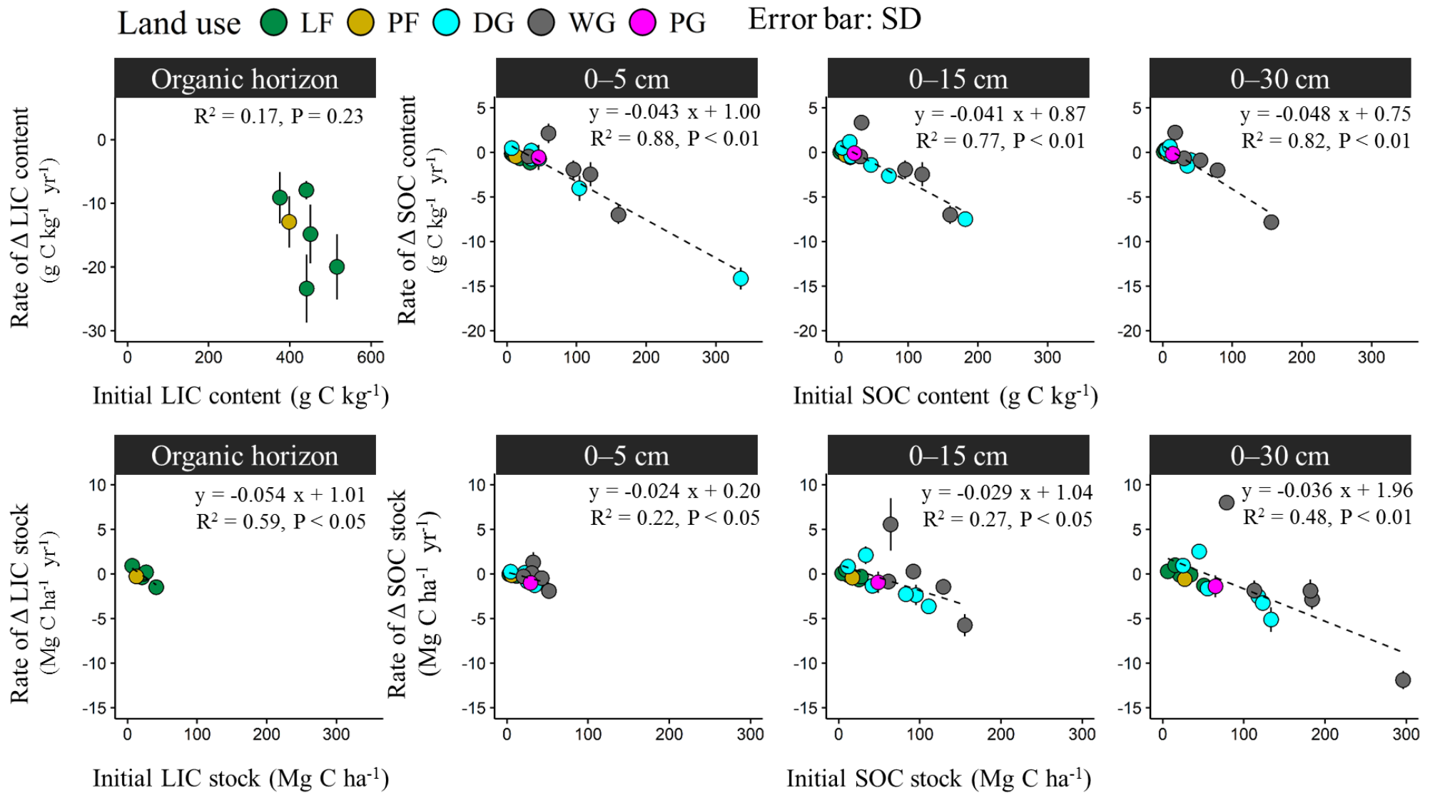
Fig. 5.4. Relationship between initial carbon and \Delta carbon. SOC: Soil organic carbon, LIC: Litter carbon. LF: Larch forest, PF: Pine forest, DG: Dry grassland, WG: Wet grassland PG: Pingo
