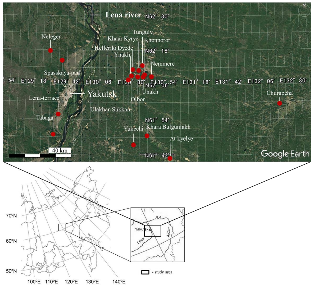
Fig. 6.1. Location of the study sites.
