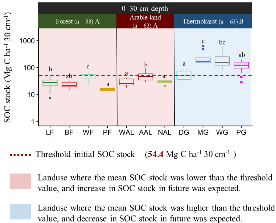
Fig. 6.13. Future prediction of soil organic carbon (SOC) stock in Central Yakutia. Box plots visualize the five-number summary of a data set (minimum, lower quartile, median, upper quartile and maximum) and points indicate outlier value. Different uppercase letters indicate significant differences between ecosystems, and different lowercase letters indicate significant differences between landscape types in the same ecosystem. SOC: Soil organic carbon, LF: Larch forest, BF: Burned larch forest, WF: Water damaged larch forest, PF: Pine forest, WAL: Working arable land, AAL: Abandoned arable land, NAL: Abandoned arable land invaded by new-growing trees, DG: Dry grassland, MG: Moderately wet grassland, WG: Wet grassland, PG: Pingo.
