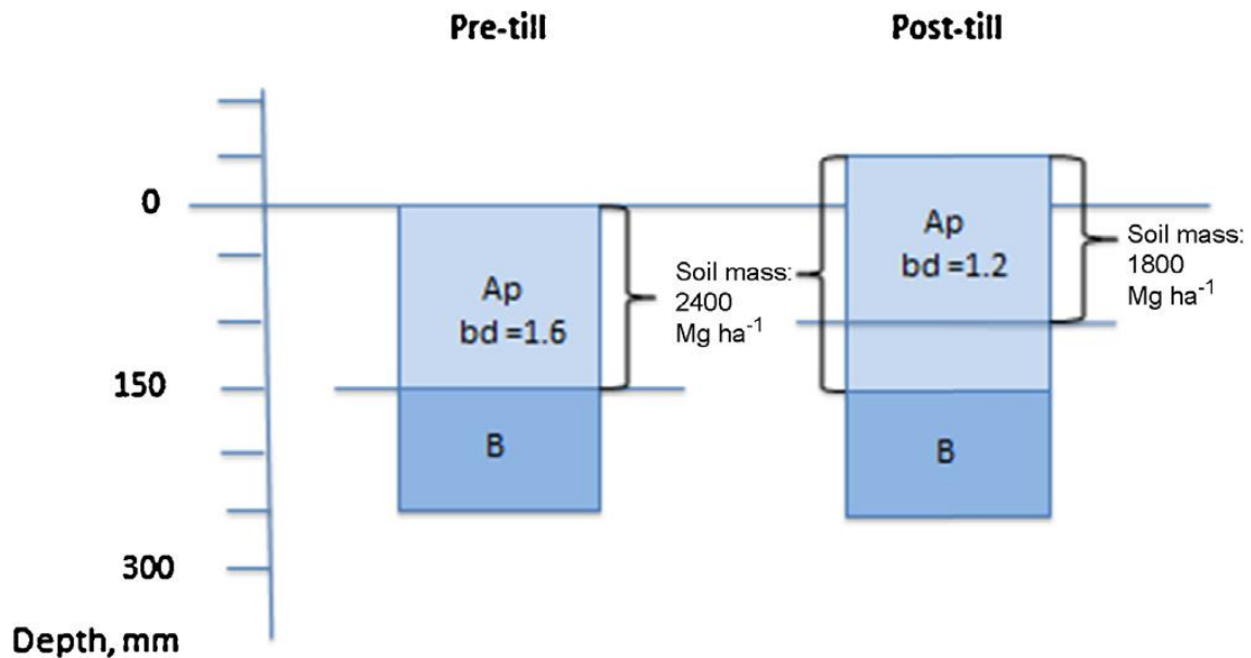
Fig. 2.3. Illustration showing the differences between sampling a soil that is tilled or not tilled to a fixed depth or an equivalent soil mass basis (Palm et al., 2014, edited from Ellert and Bettany, 1995).
