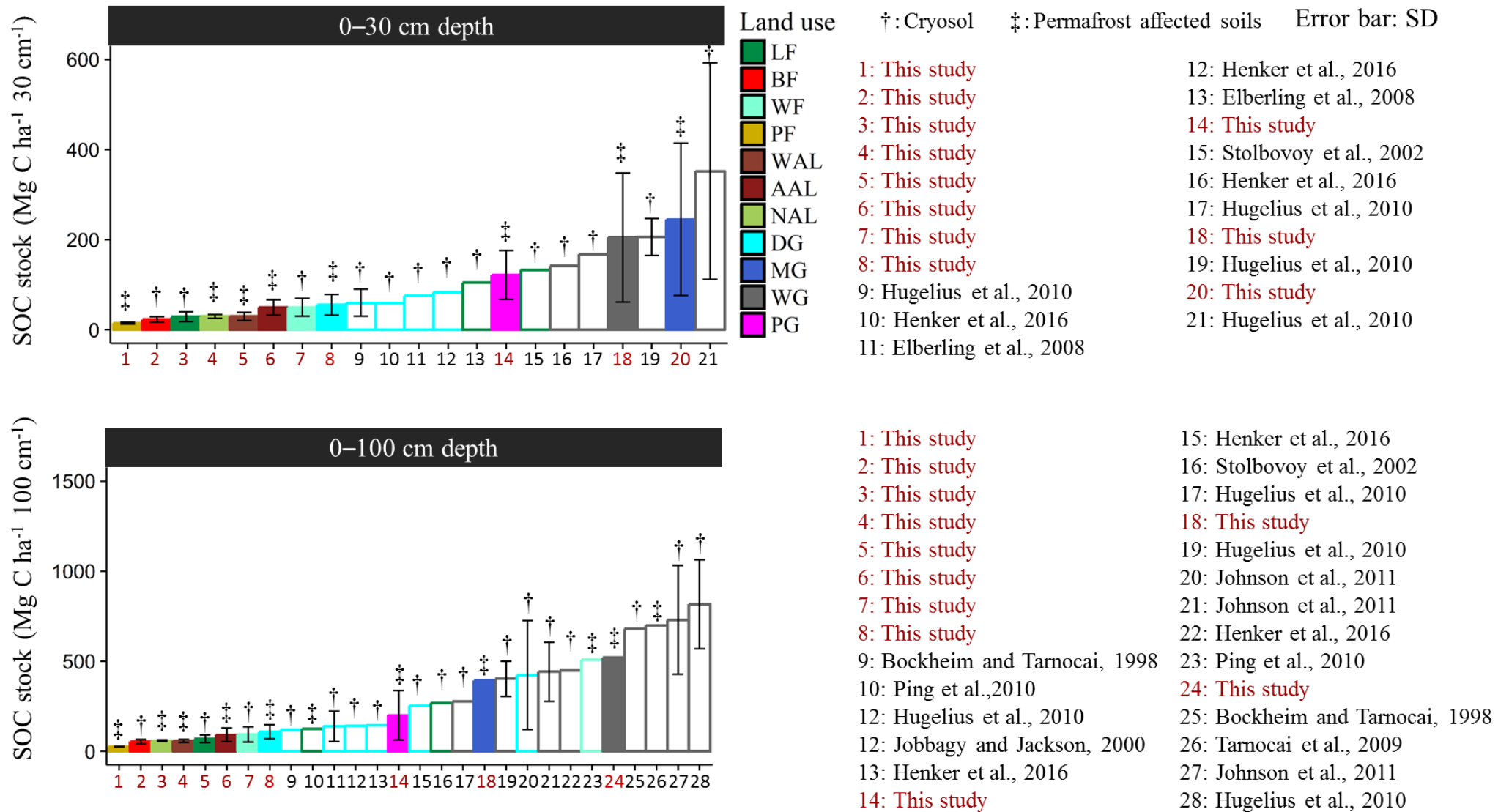
Fig. 6.8. Comparison of soil organic carbon (SOC) stocks in the 0–30 and 0–100 cm soil layers in permafrost and permafrost-affected soils.
