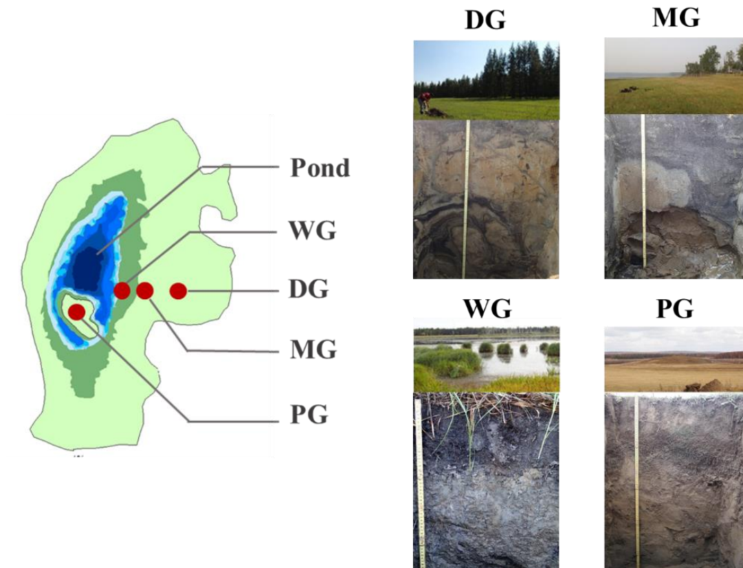
Fig. 3.6. Typical land uses in the arable land ecosystem. DG: Dry grassland, MG: Moderately wet grassland, WG: Wet grassland, PG: Pingo.
