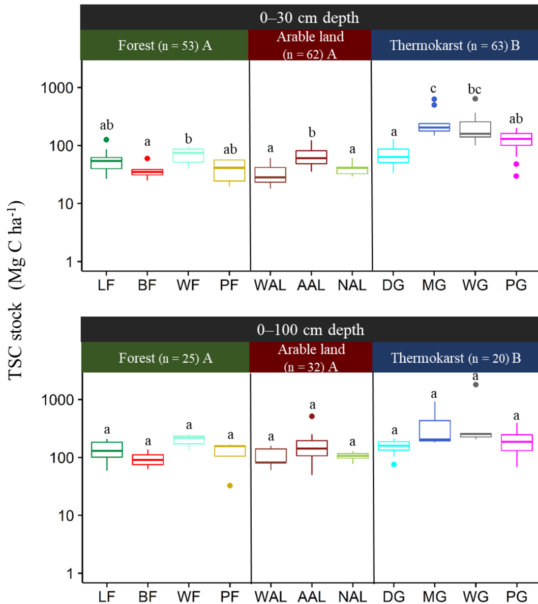
Fig. 6.6. Total soil carbon stock in the 0–30 and 0–100 cm soil layers. Box plots visualize the five-number summary of a data set (minimum, lower quartile, median, upper quartile and maximum) and points indicate outlier value. Different uppercase letters indicate significant differences between ecosystems, and different lowercase letters indicate significant differences between land use types in the same ecosystem. TSC: Total soil carbon, LF: Larch forest, BF: Burned larch forest, WF: Water damaged larch forest, PF: Pine forest, WAL: Working arable land, AAL: Abandoned arable land, NAL: Abandoned arable land invaded by new-growing trees, DG: Dry grassland, MG: Moderately wet grassland, WG: Wet grassland, PG: Pingo.
