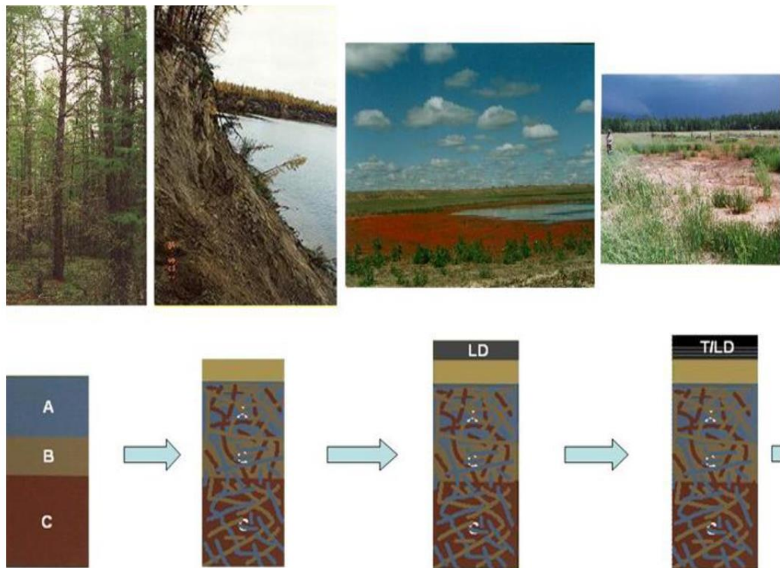
Fig. 2.5. Scheme of the transformation of the parent material upon the alas formation (Desyatkin et al., 2013). LD: lacustrine deposit, T/LD: peat and lacustrine deposit.
