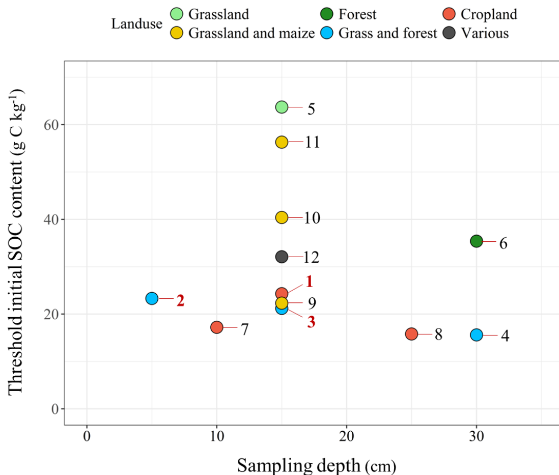
Fig. 7.2. Comparison of threshold initial soil organic carbon (SOC) content. The sampling depth of 10, 11, and 12 (Hanegraaf et al., 2009) was estimated as a mean value of grass land and maize field (0–5 cm for grassland fields and 0–25 cm for maize fields). 1: Cropland (Chapter 4), 2, 3, and 4: Grassland and forest (Chapter 5), 5: Grassland
