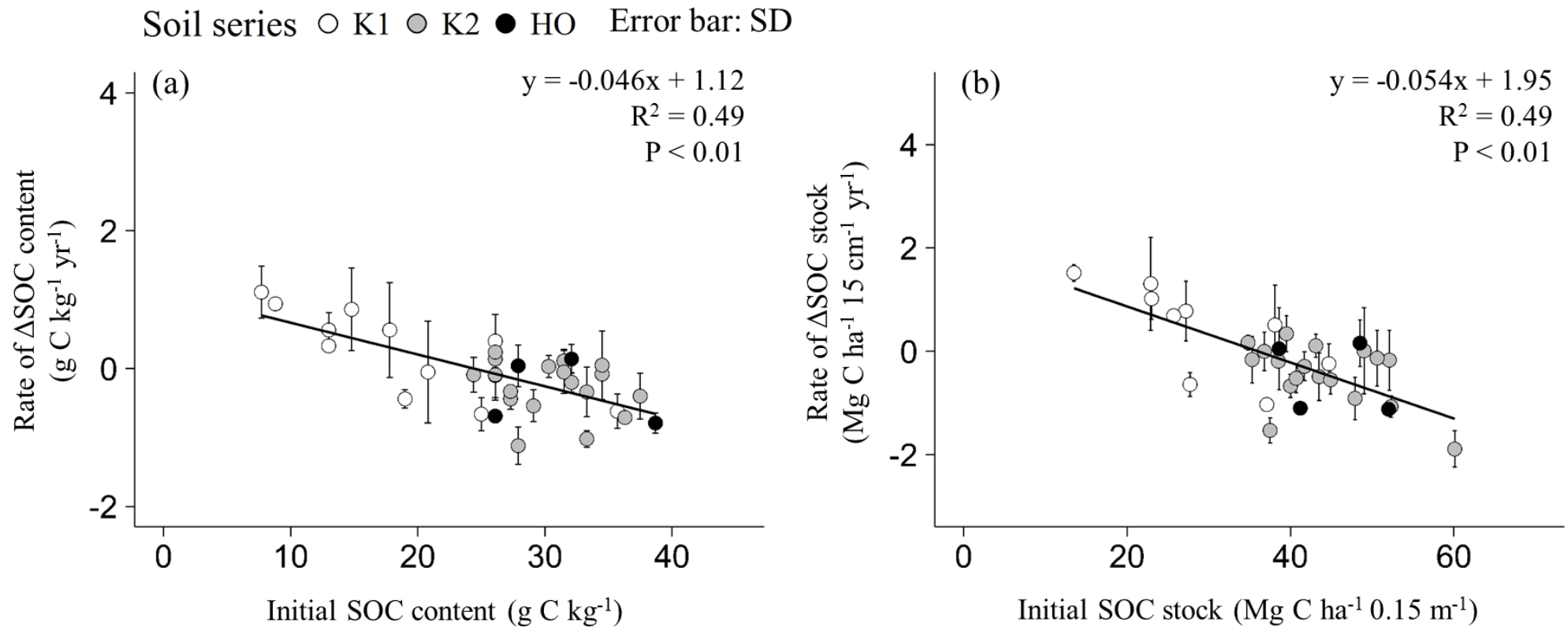
Fig. 4.3. Relationship between: (a) Initial soil organic carbon (SOC) content and rate of \Delta SOC content; (b) Initial SOC stock and rate of \Delta SOC stock.
