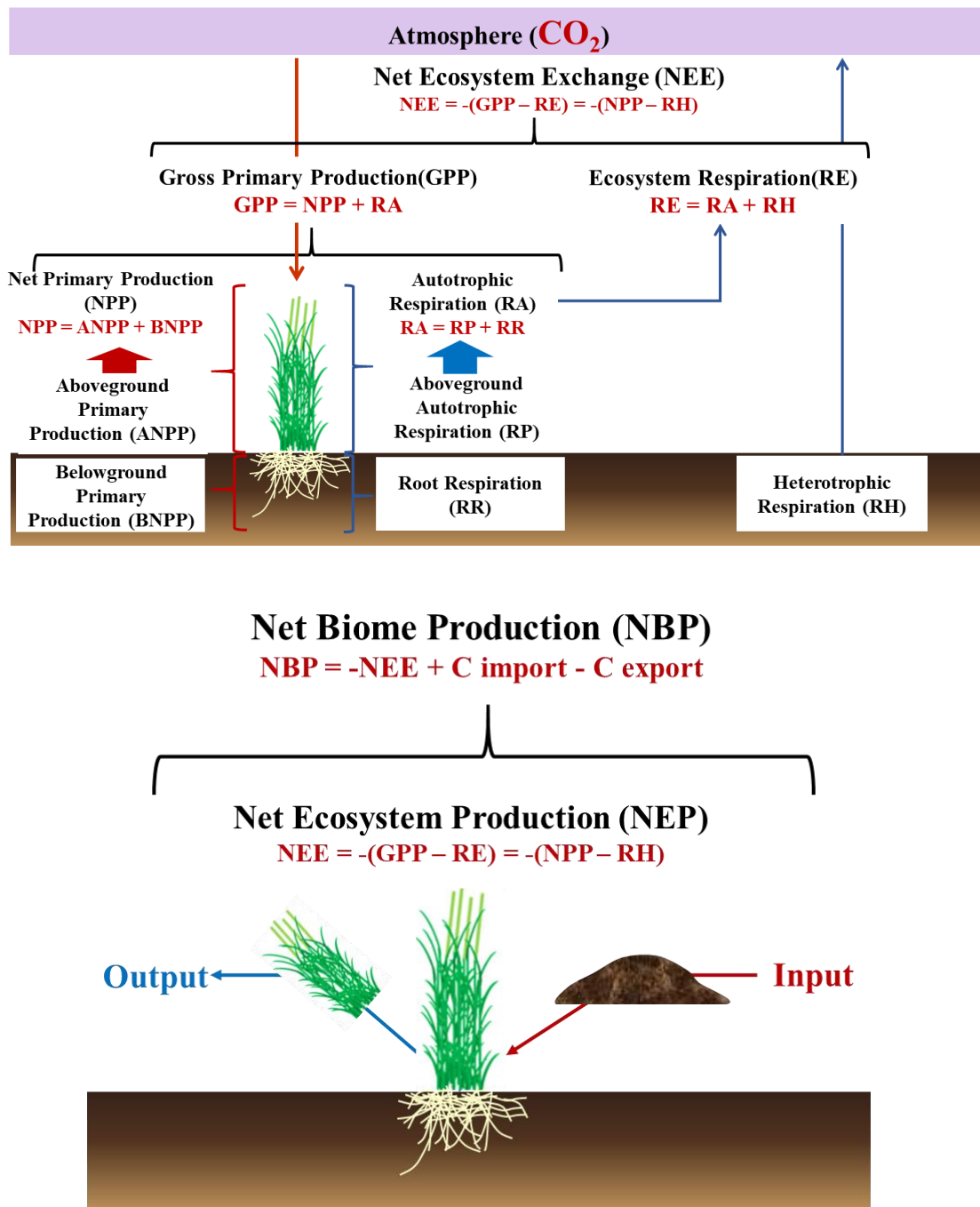
Fig. 1.2. Schematic diagram of carbon budget in the ecosystem.
