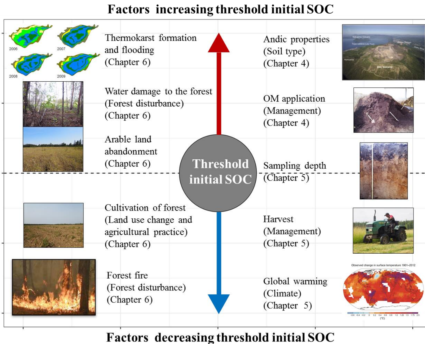
Fig. 7.4. Factors controlling threshold initial SOC. Photos were cited from Desyatkin et al., 2014 , IPCC, 2013 , and Miyabuchi et al., 2014 .
