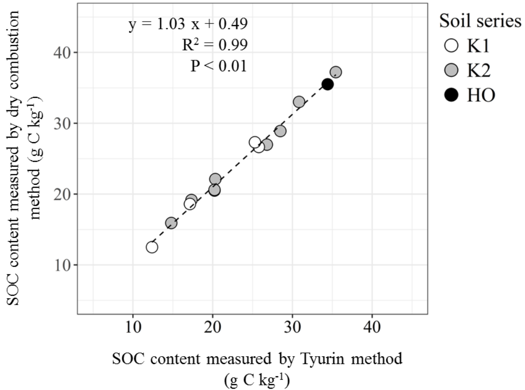
Fig. 3.8. The relationship between soil organic carbon (SOC) content measured by Tyurin method and dry combustion method.
