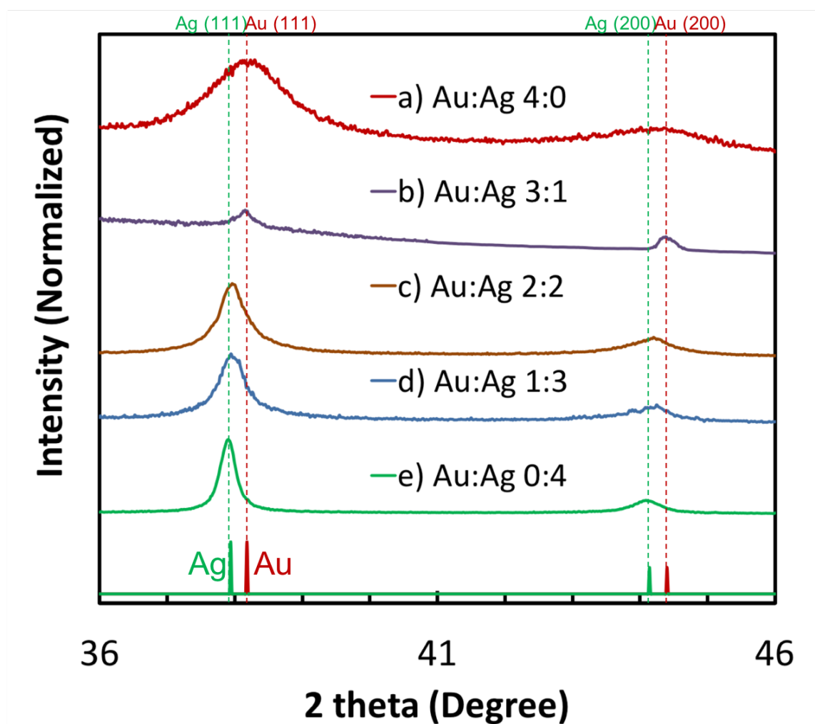
Figure 4.2 XRD patterns of NPs synthesized using different initial molar ratios Au:Ag = 4:0 (a), 3:1 (b), 2:2 (c), 1:3 (d), and 0:4 mol/mol (e). The dashed lines are for visual guide to mark position of (111) and (200) peaks for both Au and Ag. The reference patterns of Au (JCPDS no. 04-0784) and Ag (JCPDS no. 01-1164) are shown at the bottom.
