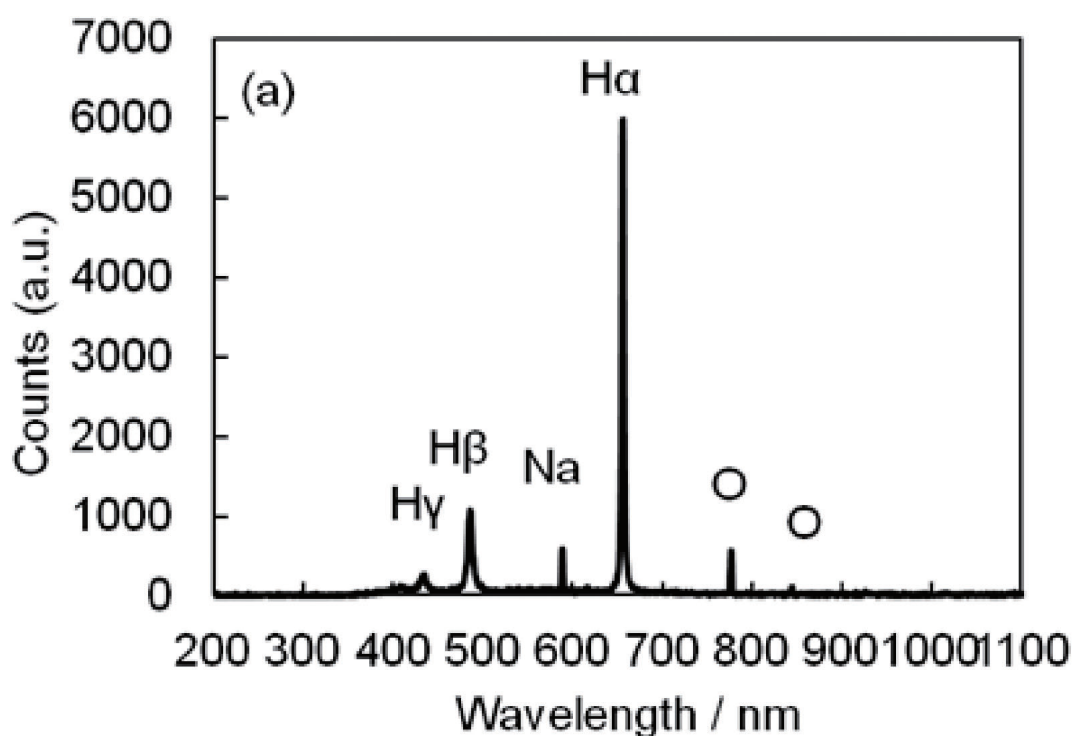
Figure 1.12 Plasma emission spectra 51
