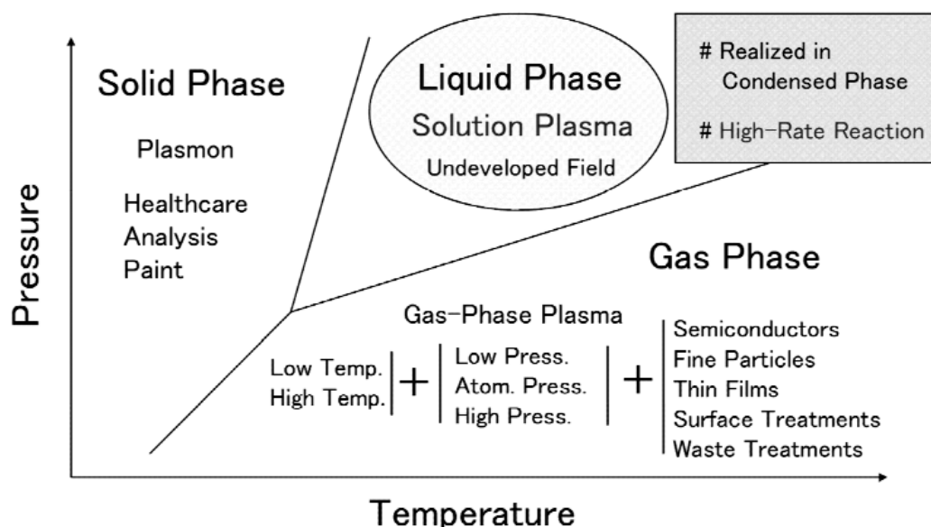
Figure 1.3 Three categories of plasma corresponding to the pressure-temperature relationship of three phases. 41
