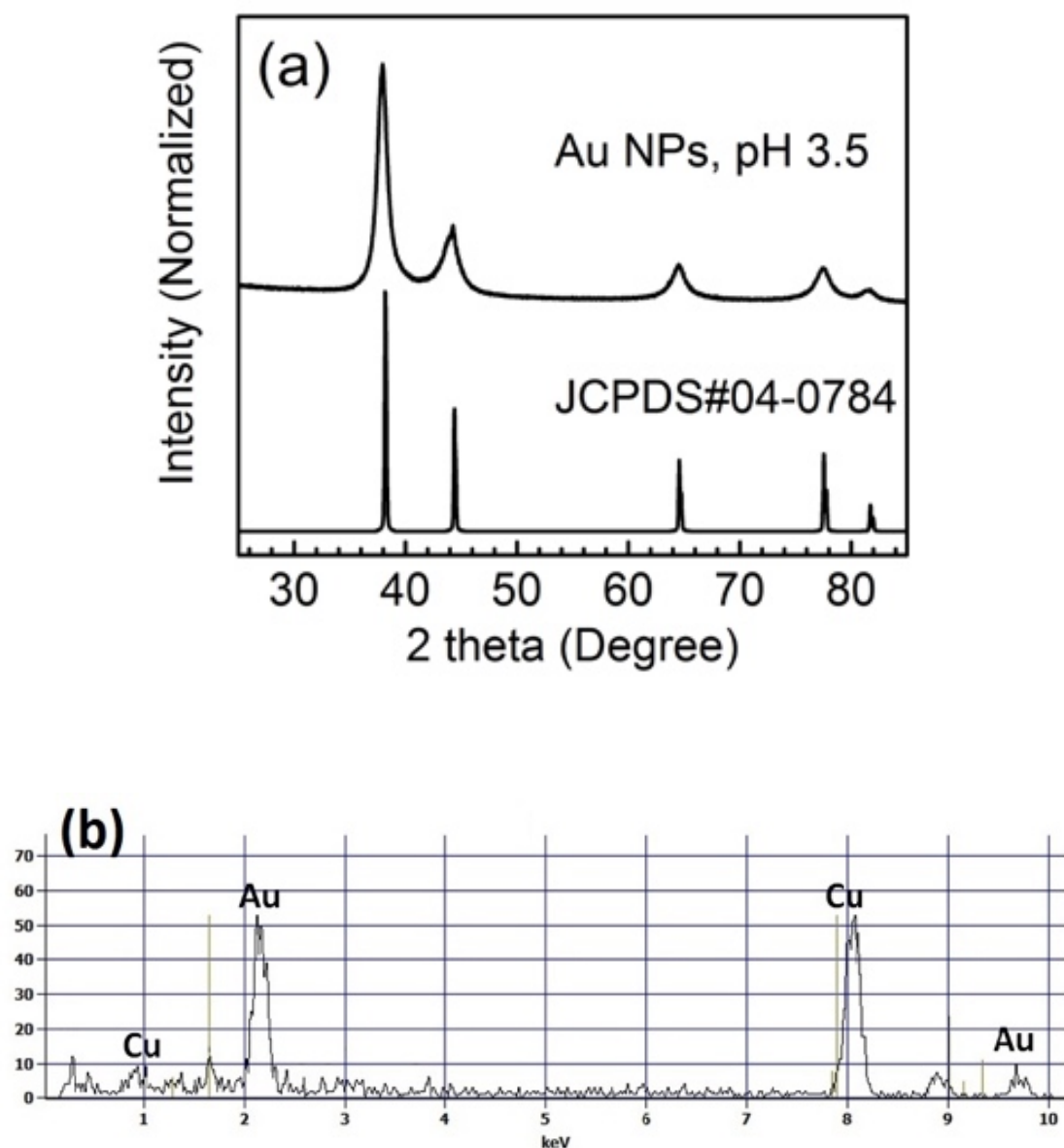
Figure 2.4 (a) XRD pattern and (b) EDS spectrum of Au NPs synthesized in solution pH 3.5. The JCPDS number of XRD reference for cubic Au was indicated.
