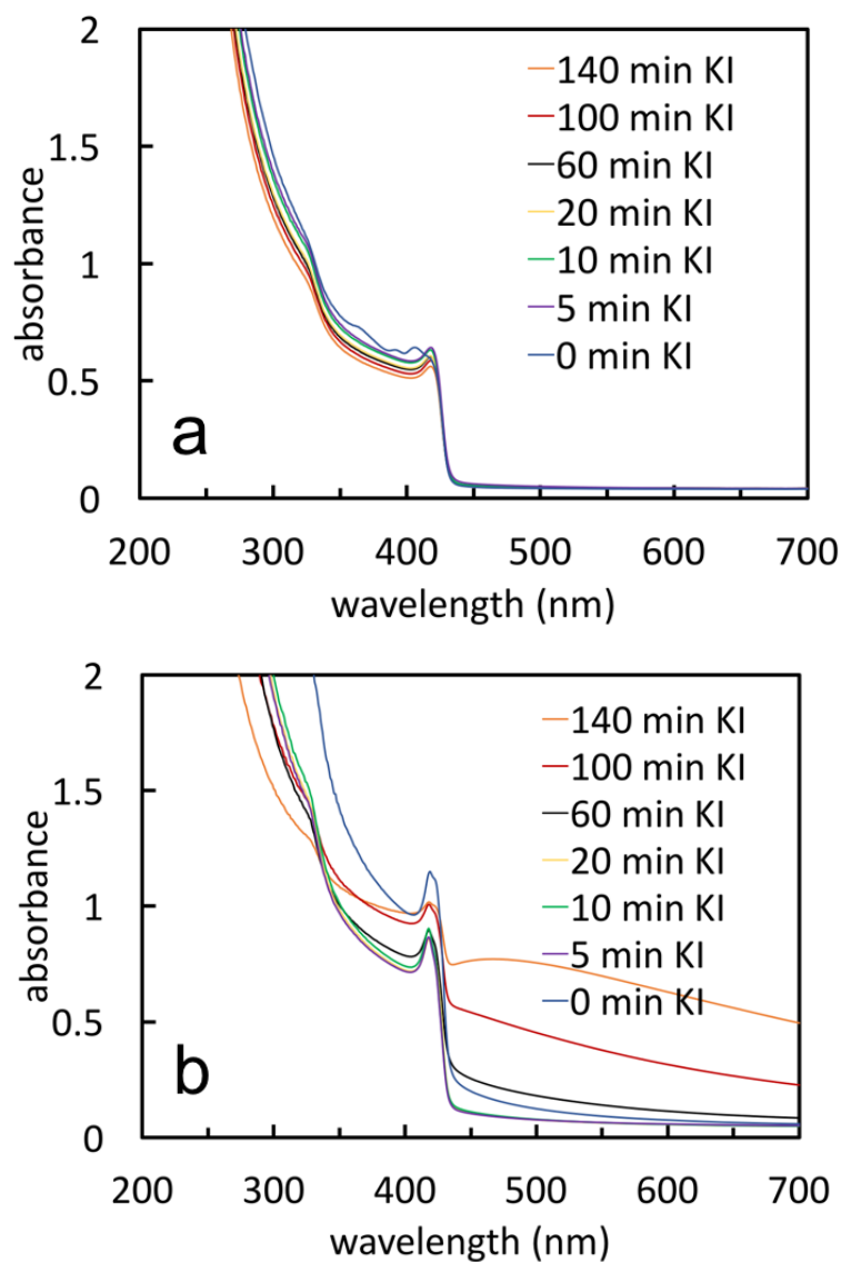
Figure 3.3 (a,b) Time dependent UV-Vis spectra observation of AgI at ca. 420 nm, formed by addition of KI into the taken out samples, during preparation of Ag NPs with: a) AgNO 3 , b) [Ag(NH 3 ) 2 ] + as the precursors.
