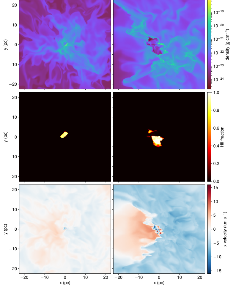
Figure 4.6: The gas density (top), H II fraction (middle), and x-velocity (bottom) on a slice for the feedback runs in the isolated cloud case (left) and 10 \text{ km s}^{-1} collisional case (right). Images are centered around the most massive sink particle a few Myr after it begins to emit radiation. The isolated cloud is shown at 5.2 Myr, while the colliding case is at 3.7 Myr as the sink formation time differs between these runs. The off-set in the velocity colourbar matches the shock propagation speed in the colliding cloud case of 5 \text{ km s}^{-1} .
