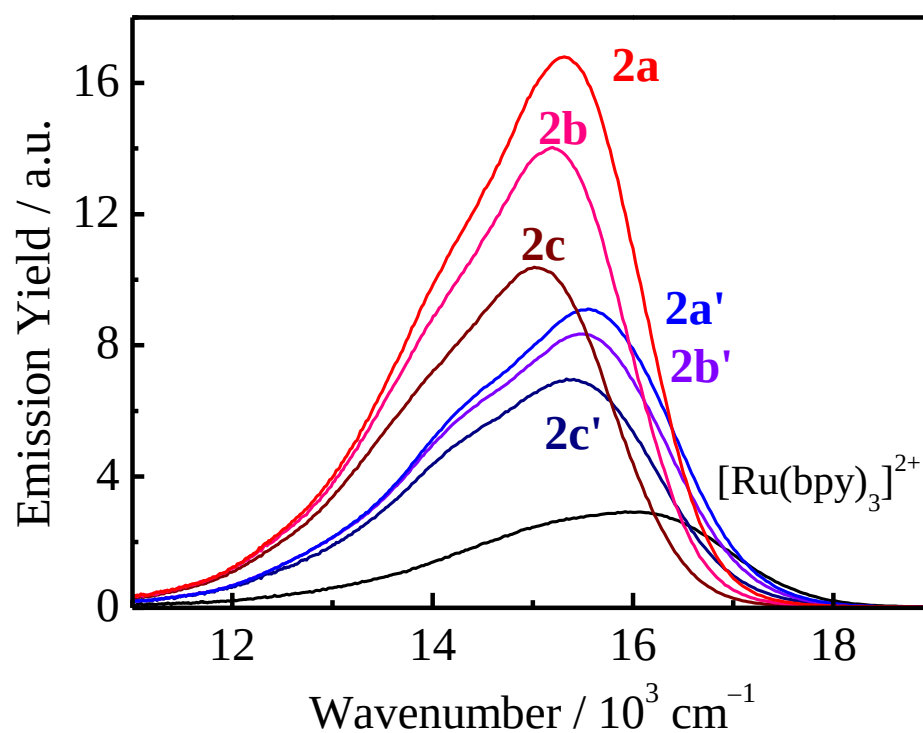
Figure 2-10. Corrected emission spectra of the complexes in \text{CH}_3\text{CN} at 298 K whose spectral integrations correspond to the relative emission quantum yields of the complexes.
