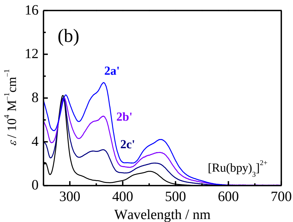
Figure 2-3. Absorption spectra of the complexes ( 2a–c (a) and 2a'–c' (b)) in \text{CH}_3\text{CN} at 298 K.
