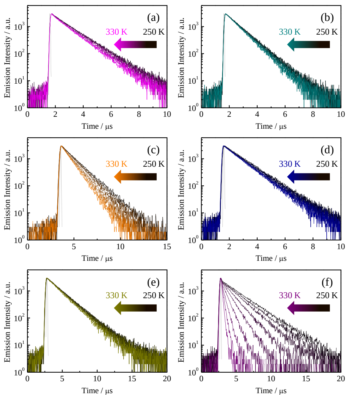
Figure 4-16. T -dependences ( T = 250–330 K) of the emission decay profiles of 4dmbpy (a), 4dmbpy (b), 4dpphen (c), 4dmphen (d), 4phen (e) and [Ru(bpy)(phen) 2 ] 2+ (f) in propylene carbonate. Gray curves represent instrumental response functions.
