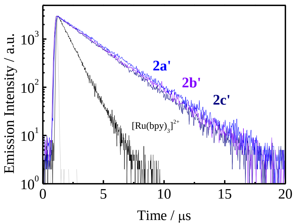
Figure 2-11. Emission decay profiles of the complexes in CH 3 CN at 298 K. Gray curves represent instrumental response functions.
