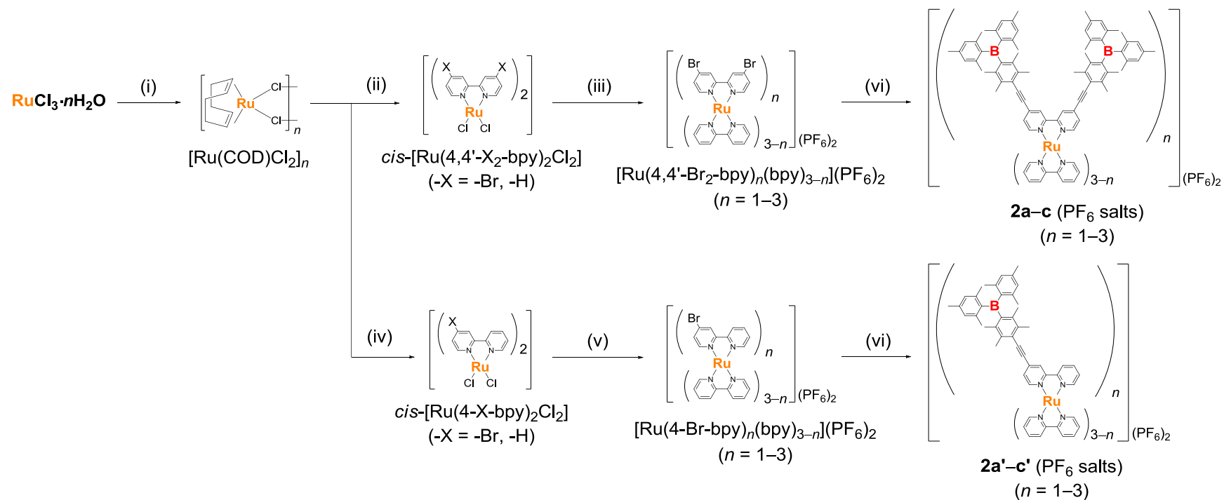
Scheme 2-1. Synthetic routes for the \text{PF}_6^- salts of the complexes: (i) 1,5-cyclooctadiene, ethanol, 80^\circ\text{C} , 45 h, (ii) 4,4'- \text{Br}_2 -bpy or bpy, o -dichlorobenzene, 160^\circ\text{C} , 2 h, (iii) 4,4'- \text{Br}_2 -bpy or bpy, ethanol/water, 80^\circ\text{C} , 5 h, (iv) 4-Br-bpy or bpy, o -dichlorobenzene, 160^\circ\text{C} , 2 h, (v) 4-Br-bpy or bpy, ethanol/water, 80^\circ\text{C} , 5 h, (vi) EDDB, \text{Pd}(\text{PPh}_3)_2\text{Cl}_2 , \text{CuI} , \text{NEt}_3 , \text{CH}_3\text{CN}/\text{THF} , 50^\circ\text{C} , 4 h.
