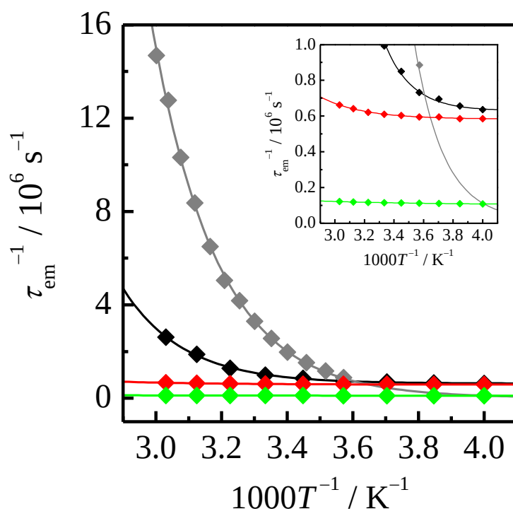
Figure 3-8. T -dependences ( T = 250\text{--}330\text{ K} ) of \tau_{em} of the complexes in propylene carbonate. The colors of the data points correspond to those indicated in Figure 3-1. The curves represent the best fits of the experimental data by eq. 3-1. Inset: enlarged view. The data on [\text{Ru}(\text{phen})_3]^{2+} and [\text{Ru}(\text{bpy})_3]^{2+} are taken from ref. [2] and Figure 2-14 in Chapter 2, respectively.
