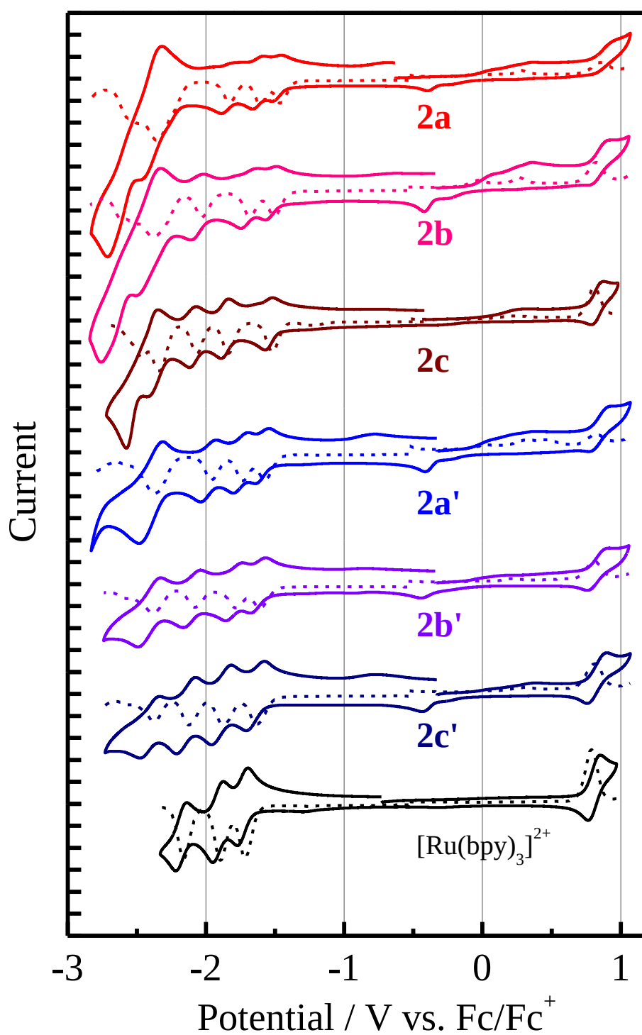
Figure 2-1. CVs (solid curves) and DPVs (broken curves) of 2a–c , 2a'–c' and [\text{Ru}(\text{bpy})_3]^{2+} in DMF containing 0.1-M TBAPF 6 . The vertical-axis scale is 5 μA per division.
