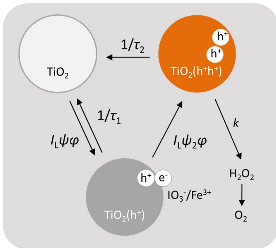
Scheme 1 two-electron transfer reaction model of photocatalytic oxygen evolution
