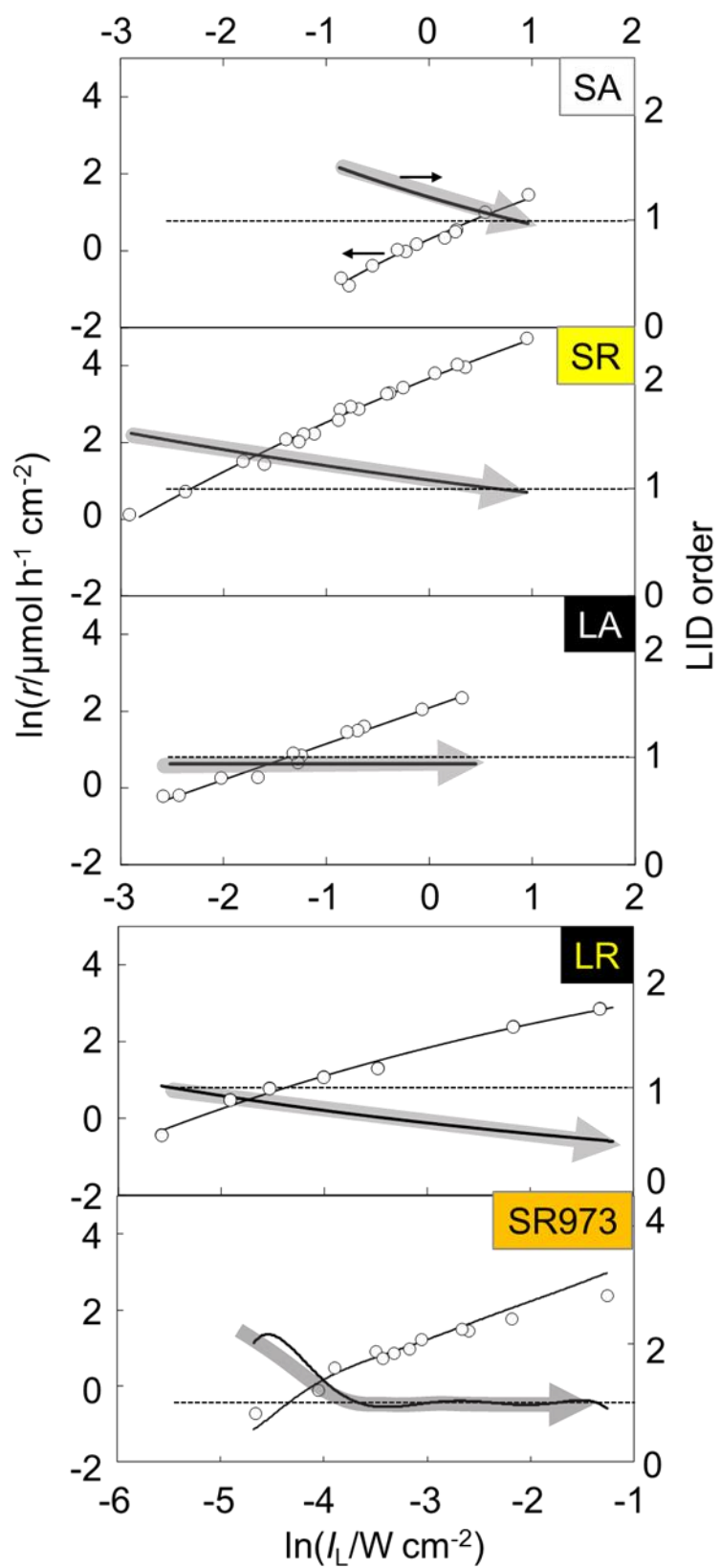
Fig. 3-9 Double-logarithm plot of corrected light-intensity dependence of reaction rate for each titania samples in the presence of \text{Fe}^{3+} as an electron acceptor.
