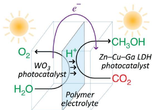
Fig. 1-3 Carbon dioxide-reduction system using double-layered photocatalyst device under visible-light irradiation [Morikawa 2014]
