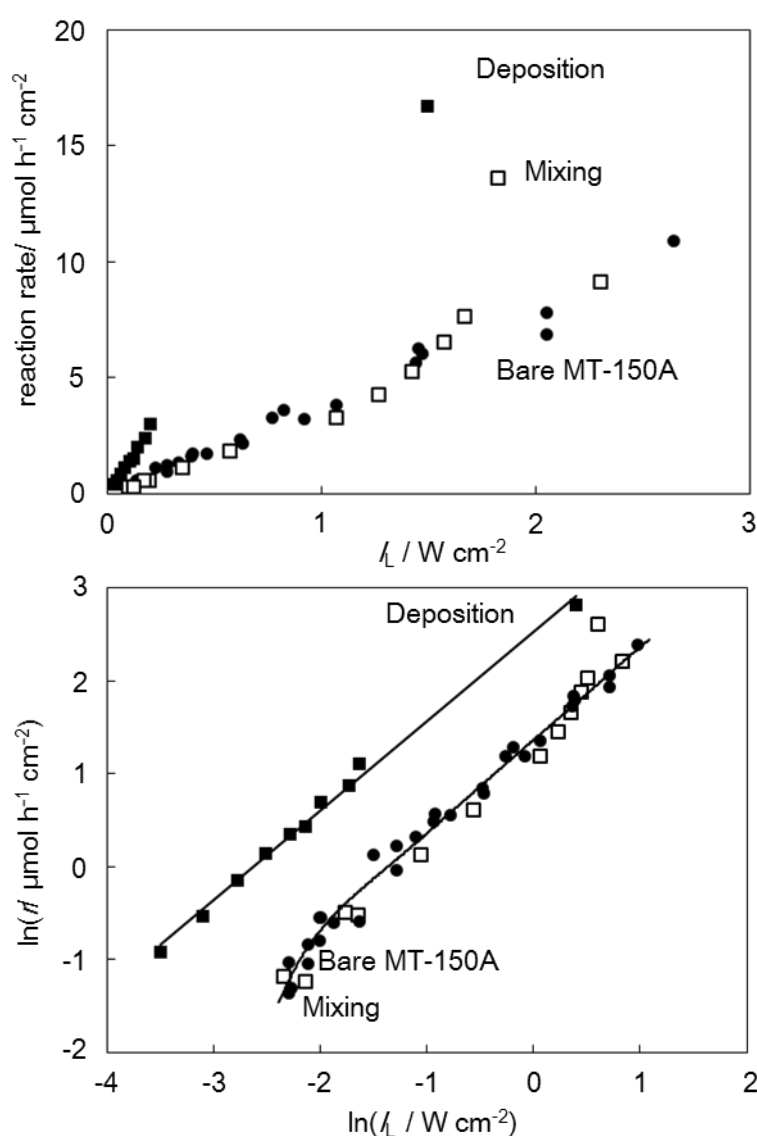
Fig. 4-2 light-intensity dependence of reaction rate and double-logarithm plot for 0.1 wt% MnO 2 deposited and mixed titania samples in the presence of IO 3 - as an electron acceptor.
