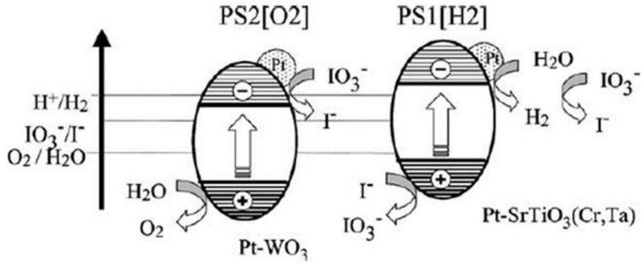
Fig. 1-2 Speculated reaction mechanism of Z-Scheme using an iodate( \text{IO}_3^- )/iodide ( \text{I}^- ) mediator [Sayama 2001]
