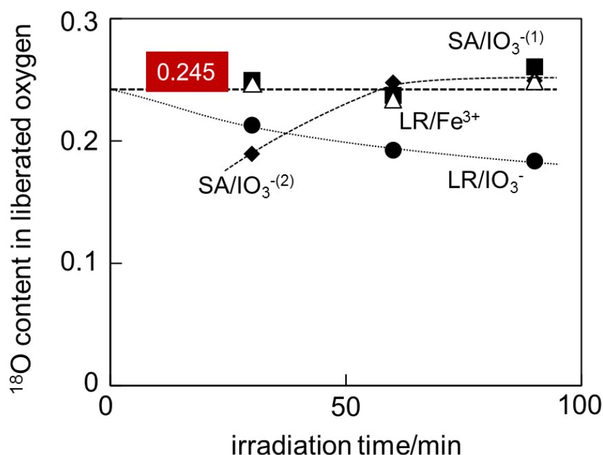
Fig. 3-8 ^{18}\text{O} content in oxygen liberated from the suspensions of SA and LR titania samples with \text{IO}_3^- and \text{Fe}^{3+} ions as an EA (Closed circle, triangle, closed square, and rhombus correspond to LR/ \text{IO}_3^- , LR/ \text{Fe}^{3+} , SA/ \text{IO}_3^- (first time), SA/ \text{IO}_3^- (second time), respectively.)
