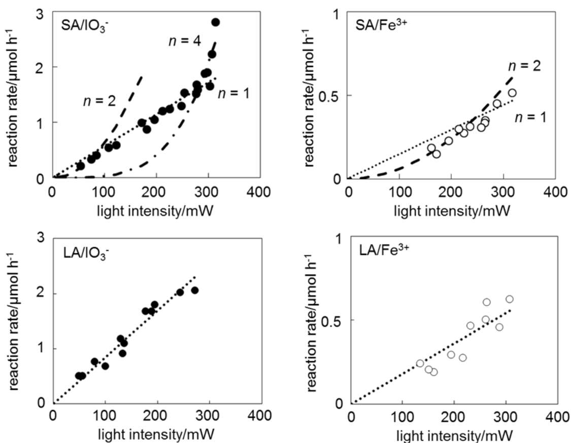
Fig.3-3 Light-intensity dependence of reaction rate of oxygen evolution using Anatase TiO 2 in the presence of electron acceptor (IO 3 - , Fe 3+ )
