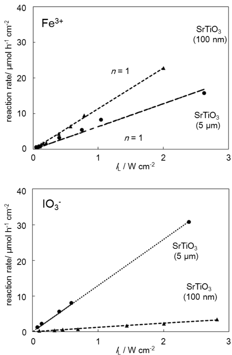
Fig.3-9 Light-intensity dependence of reaction rate of oxygen evolution using two type of \text{SrTiO}_3 samples in the presence of electron acceptor ( \text{IO}_3^- , \text{Fe}^{3+} )
