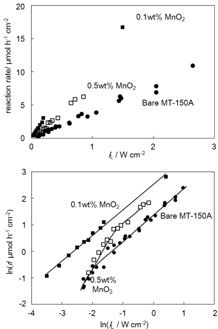
Fig. 4-3 Double-logarithm plot of light-intensity dependence of reaction rate for different amount \text{MnO}_2 loaded titania samples in the presence of \text{IO}_3^- as an electron acceptor.
