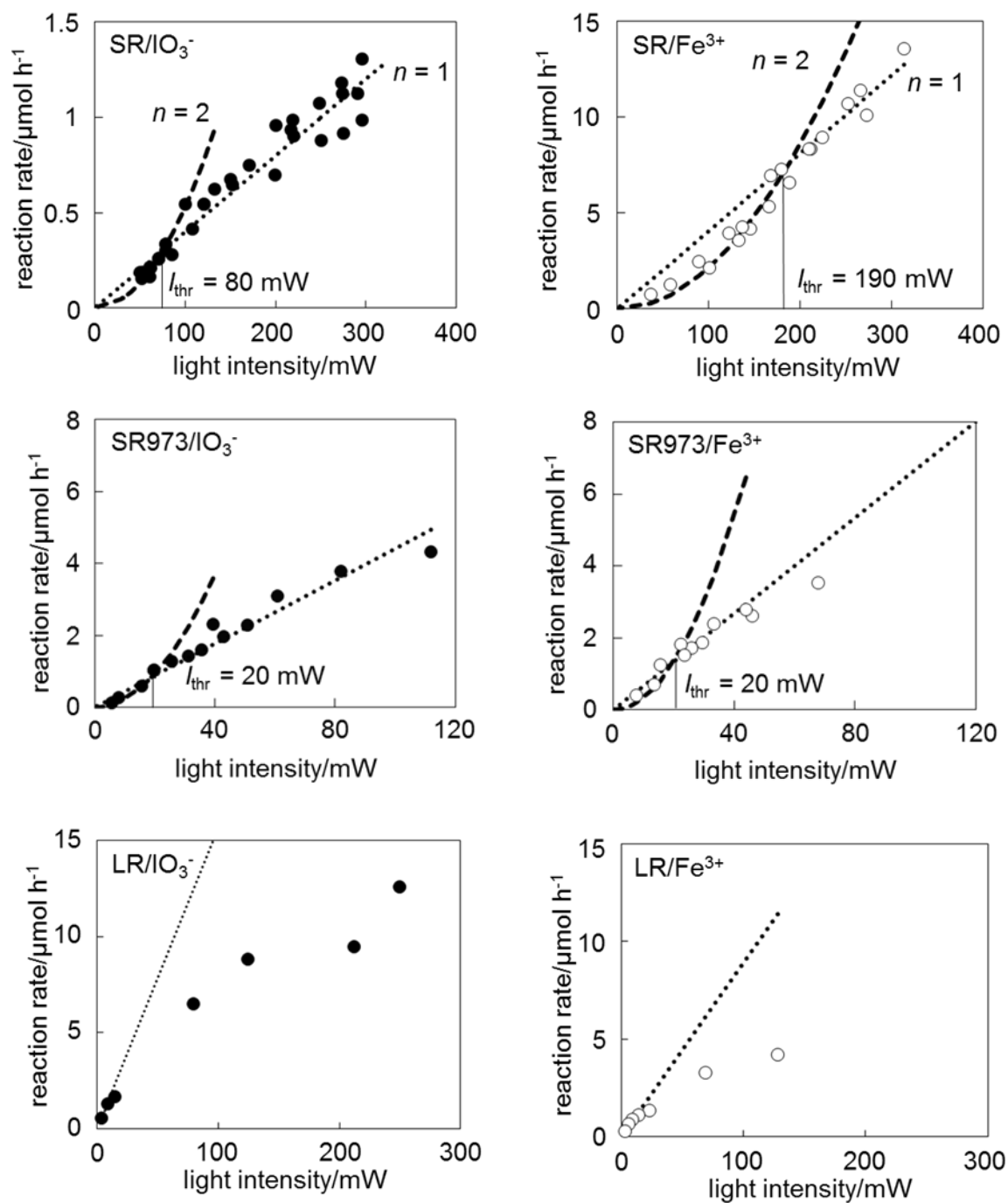
Fig.3-2 Light-intensity dependence of reaction rate of oxygen evolution using rutile \text{TiO}_2 in the presence of electron acceptor ( \text{IO}_3^- , \text{Fe}^{3+} )
