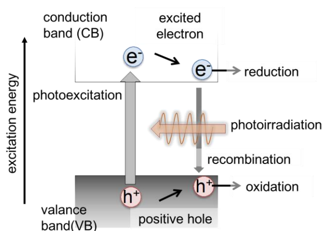
Fig.1-1 Principle of photocatalysis based on a band-structure model
