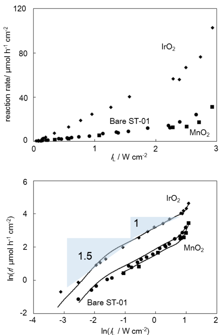
Fig. 4-4 Double-logarithm plot of light-intensity dependence of reaction rate for Co-catalyst loaded ST-01 in the presence of IO 3 - as an electron acceptor.
