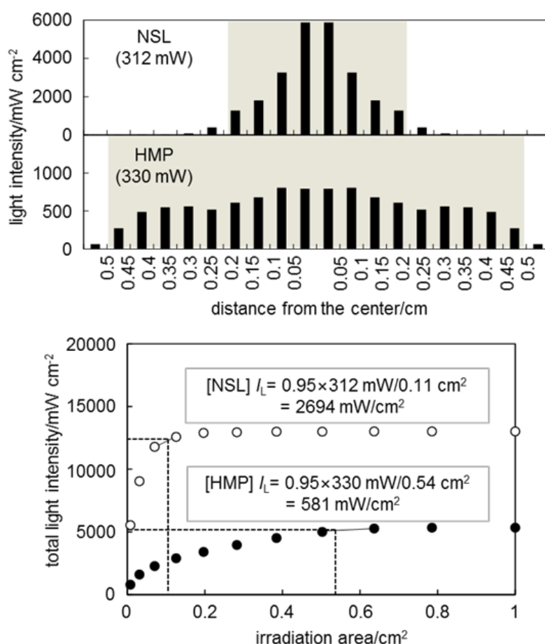
Fig.3-5 (upper) Examples of light-intensity distribution of NSL and HMP UV-LEDs. Colored areas indicate effective irradiation area ( A_{95} ). (lower) Calculation of A_{95} and I_L from light-intensity distributions.
