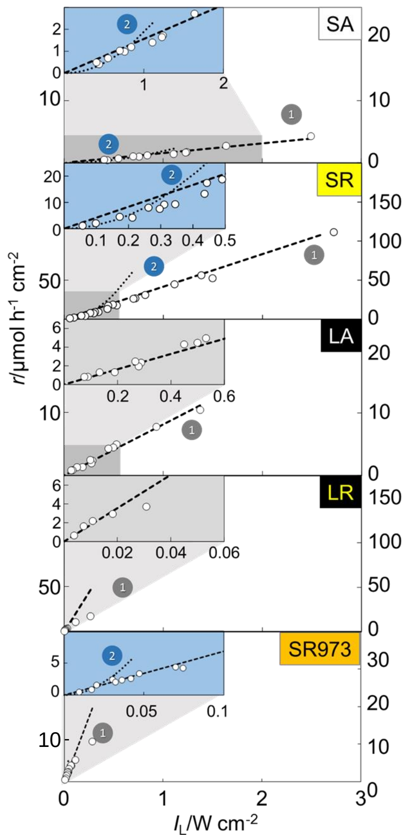
Fig. 3-8 Corrected light-intensity dependence of reaction rate for each titania samples in the presence of \text{Fe}^{3+} as an electron acceptor.
