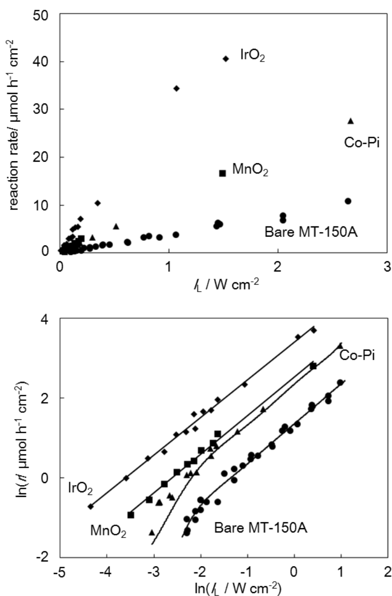
Fig. 4-1 light-intensity dependence of reaction rate and double-logarithm plot for each 0.1 wt% co-catalyst loaded titania samples in the presence of IO 3 - as an electron
