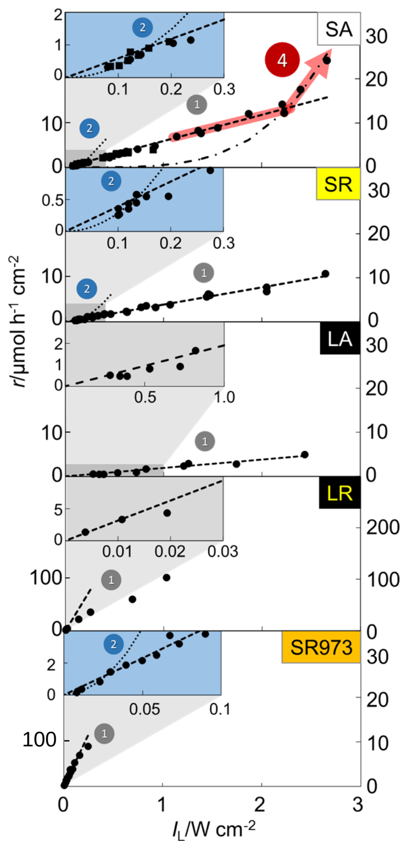
Fig. 3-6 Corrected light-intensity dependence of reaction rate for each titania samples in the presence of \text{IO}_3^- as an electron acceptor.
