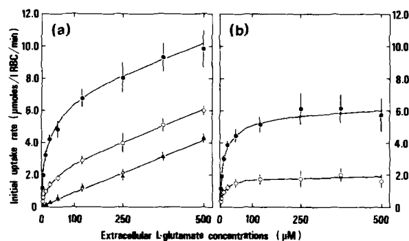
FIG. 1. Effect of Na + on L-glutamate transport in high K + and low K + dog erythrocytes. a, L-glutamate transport in the presence (● and ○) or absence (▲ and △) of extracellular Na + . ● and ▲, high K + dog erythrocytes (n = 8); ○ and △, low K + dog erythrocytes (n = 7). Uptakes were measured at 37 °C for 60 s in the medium containing 150 mM NaCl, 5 mM KCl, 2 mM MgCl 2 , 10 mM D-glucose, 0.1% (w/v) BSA, and 15 mM MOPS/NaOH (pH 7.5) when Na + was present. Choline chloride and MOPS/Tris (pH 7.5) were substituted for NaCl and MOPS/NaOH (pH 7.5), respectively, when Na + was absent. The detailed procedures of the L-glutamate uptake measurement are described under "Experimental Procedures." Data are expressed as mean \pm S.D. b, Na + gradient-dependent L-glutamate uptake in high K + (●) and low K + (○) dog cells. Data were obtained by subtracting the uptake rate in the absence of Na + from the uptake rate in the presence of Na + at each concentration of L-glutamate, and expressed as mean \pm S.D.
