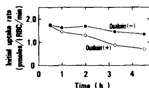
FIG. 3. Incubation time-dependent inhibitory effect of ouabain on L-glutamate transport in high K^+ dog erythrocytes. ●, incubated in the medium without ouabain; ○, incubated with 0.1 mM ouabain. Ouabain when present was added to the erythrocyte suspension at a concentration of 0.1 mM. Incubations were carried out for the appropriate time at 37^\circ\text{C} with a gentle shaking, and then L-glutamate uptake was measured at the extracellular nonlabeled L-glutamate concentration of 5 \mu\text{M} . In this experiment, the uptake was examined using only the medium containing 150 mM NaCl and 15 mM MOPS/NaOH (pH 7.5), since almost all of the uptake of L-glutamate at the extracellular concentration of 5 \mu\text{M} was \text{Na}^+ gradient-dependent (Fig. 1). Data are the mean values of two experiments.
