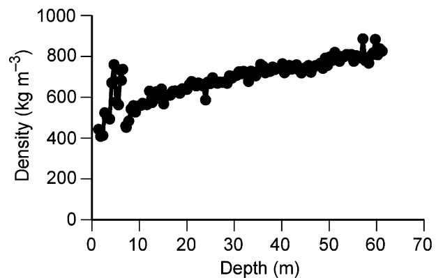
Fig. 5. Vertical profile of ice core density.
