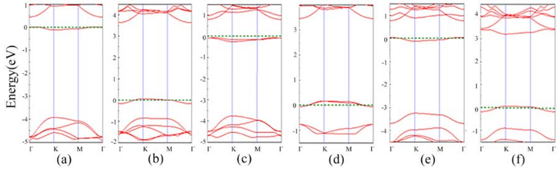
Fig. 2. (Color Online) The electronic band structures of the hypothetical materials. Figures 2(a) - 2(f) correspond to Figs. 1(a) - 1(f), respectively.
