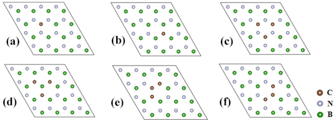
Fig. 1. (Color Online) Typical examples of odd number substitutions. (a) A carbon atom replaces a boron atom. (b) A carbon atom replaces a nitrogen atom. (c) Three carbon atoms replace three boron atoms. (d) Three carbon atoms replace three nitrogen atoms. (e) Three carbon atoms replace a boron atom and two nitrogen atoms. (f) Three carbon atoms replace two boron atoms and a nitrogen atom.
