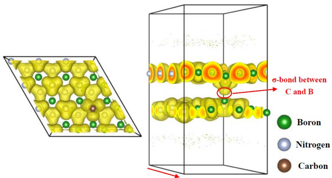
Fig. 10. The ELF distribution of “2C - iii”.
