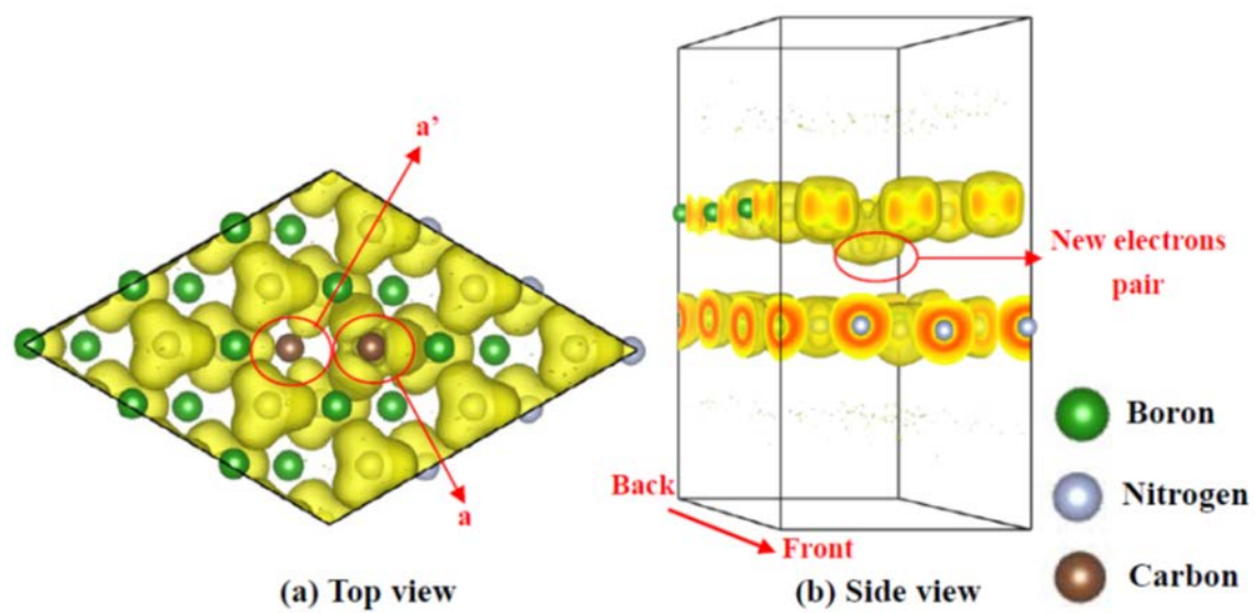
Fig. 8. The ELF distribution of "2C - ii".
