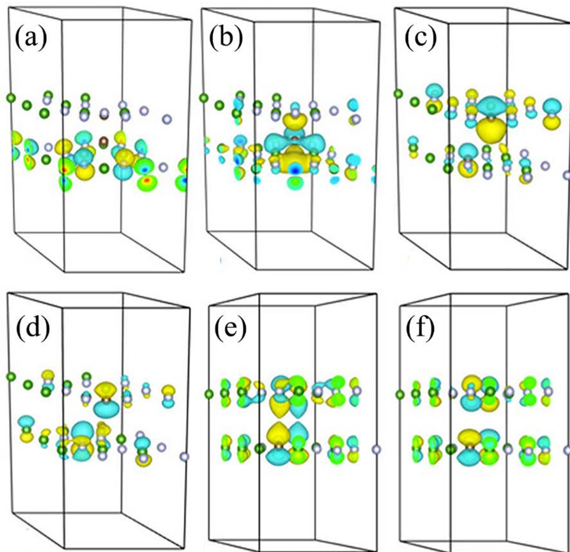
Fig. 6. (Color Online) HOMO and LUMO of the double-layered structures.
