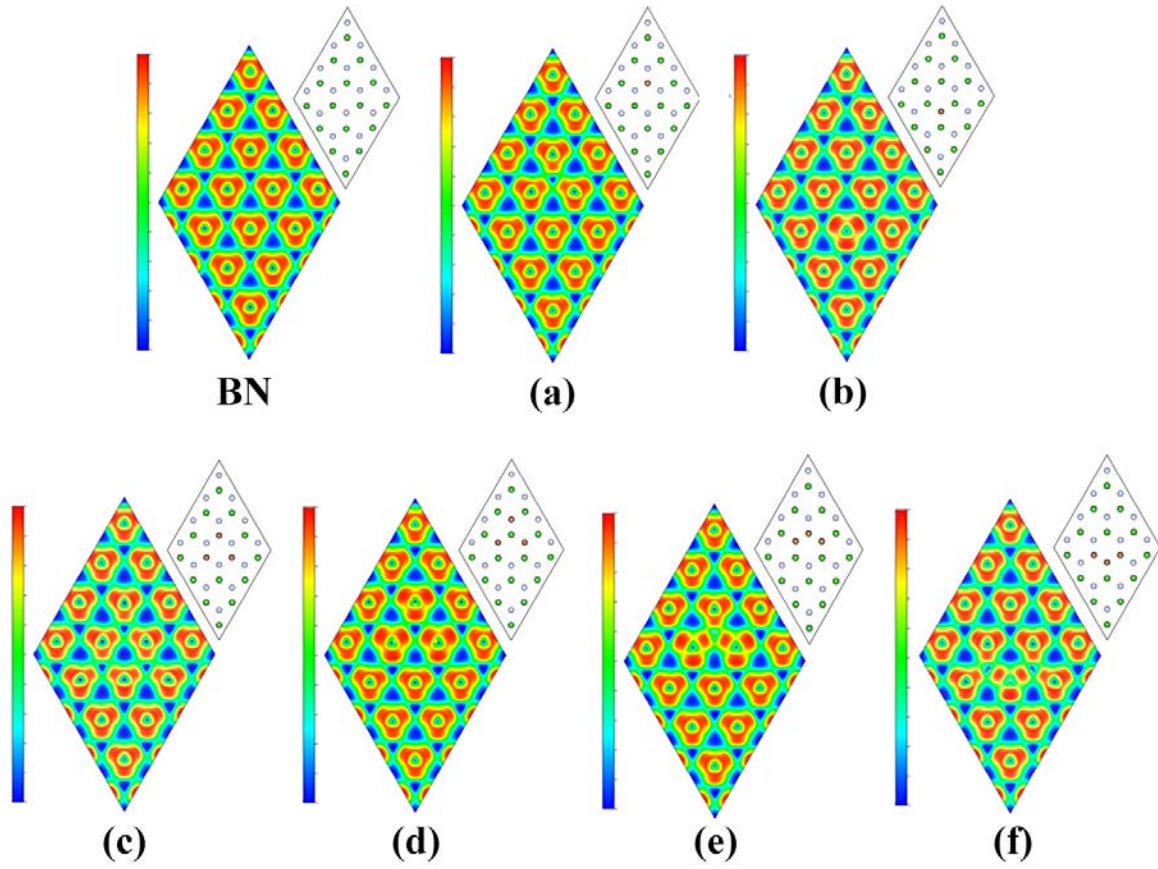
Fig. 3. (Color Online) 2D-electron localization function (ELF) distribution of the monolayer h-CBN structures. (a)~(f) correspond to those in Figs.1 and 2 as shown in the insets.
