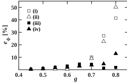
Fig. 5 The difference in \hat{\Phi} , e_\Phi , between the numerical and analytical solutions of the RTE with different g -values for Combinations (i) to (iv). Other details are the same as in Fig. 3.
