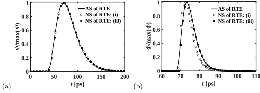
Fig. 4 Temporal profiles of the fluence rate, \Phi , in the numerical phantoms modeling the titanium dioxide suspensions as listed at Table 1: (a) g = 0.45 and (b) g = 0.80 , respectively. Open and solid squares represent the numerical solutions (NS) of the RTE for Combinations (i) and (iii), respectively; and solid lines the analytical solutions (AS) of the RTE (Eq. (10)).
