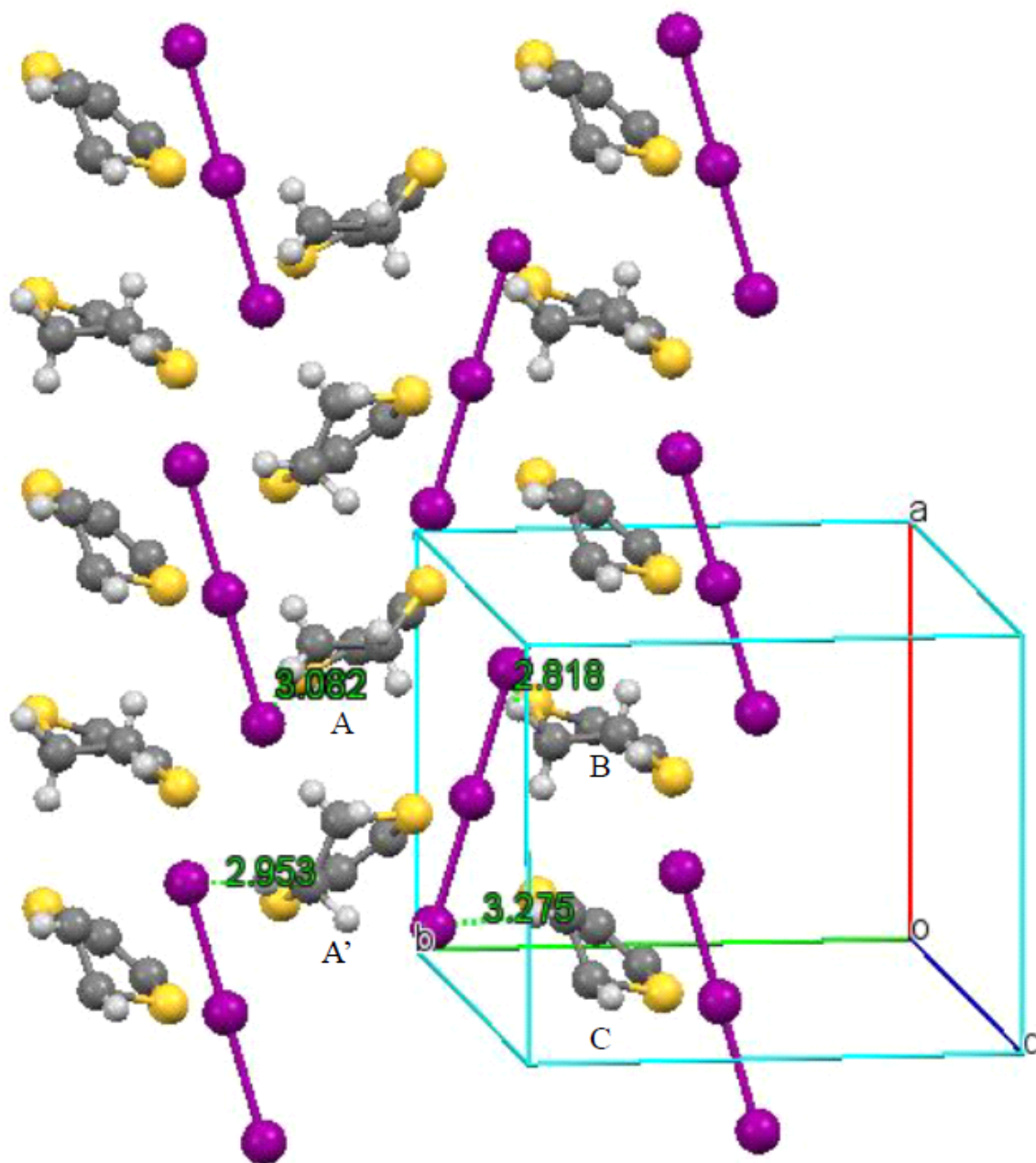
Figure 4.1: Crystal structure of \alpha -(BEDT-TTF) _2 I _3 along the c^* direction. Green numbers in the figure are hydrogen bond lengths between the hydrogen of a BEDT-TTF closest to I _3^- and end of the I _3^- .
