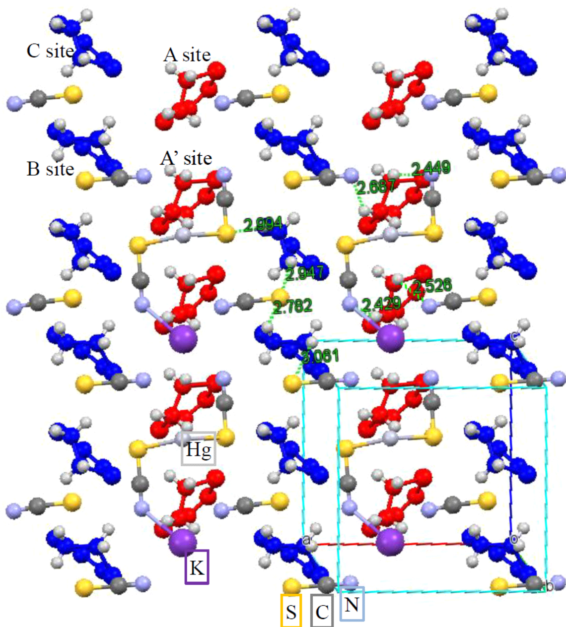
Figure 4.2: Crystal structure of \alpha -(BEDT-TTF) 2 KHg(SCN) 4 along the b^* direction. Green numbers in the figure are hydrogen bond lengths between the hydrogen of a BEDT-TTF closest to SCN - and a sulfur or a nitrogen of the SCN - . We focus on a sulfur and a nitrogen of SCN - in an anion layer, since they are located near a mercury ion with positive divalent and a potassium ion with positive monovalent and SCN - s are more closer to BEDT-TTF layer. BEDT-TTFs with red and blue belong to Column I and Column II, respectively.
