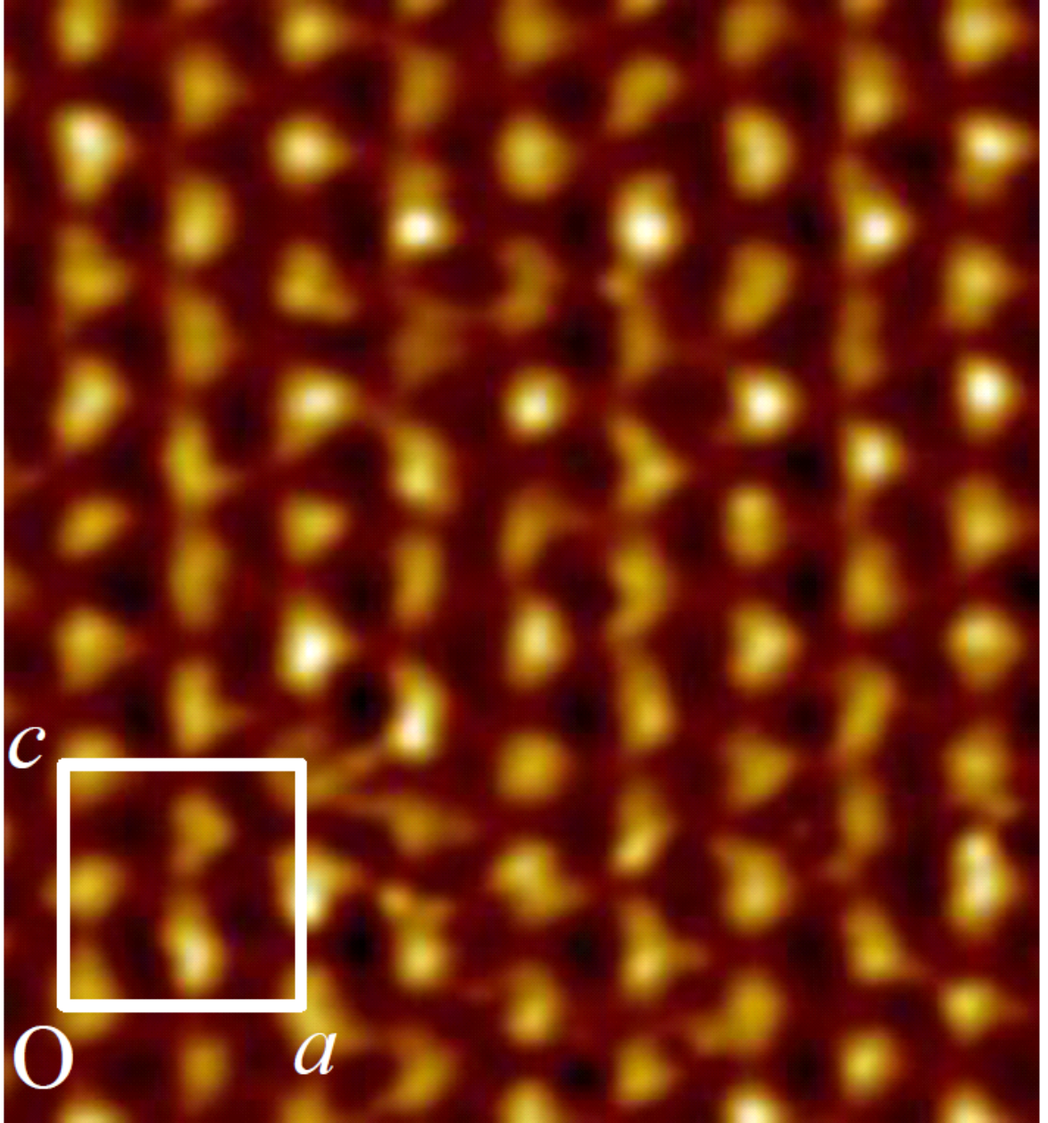
Figure 3.8: STM current image of \alpha -(BEDT-TTF) _2 RbHg(SCN) _4 at tunneling current I = 0.5 nA and bias voltage V = 15 mV with scanning area of 4.4 \text{ nm} \times 3.7 \text{ nm}
