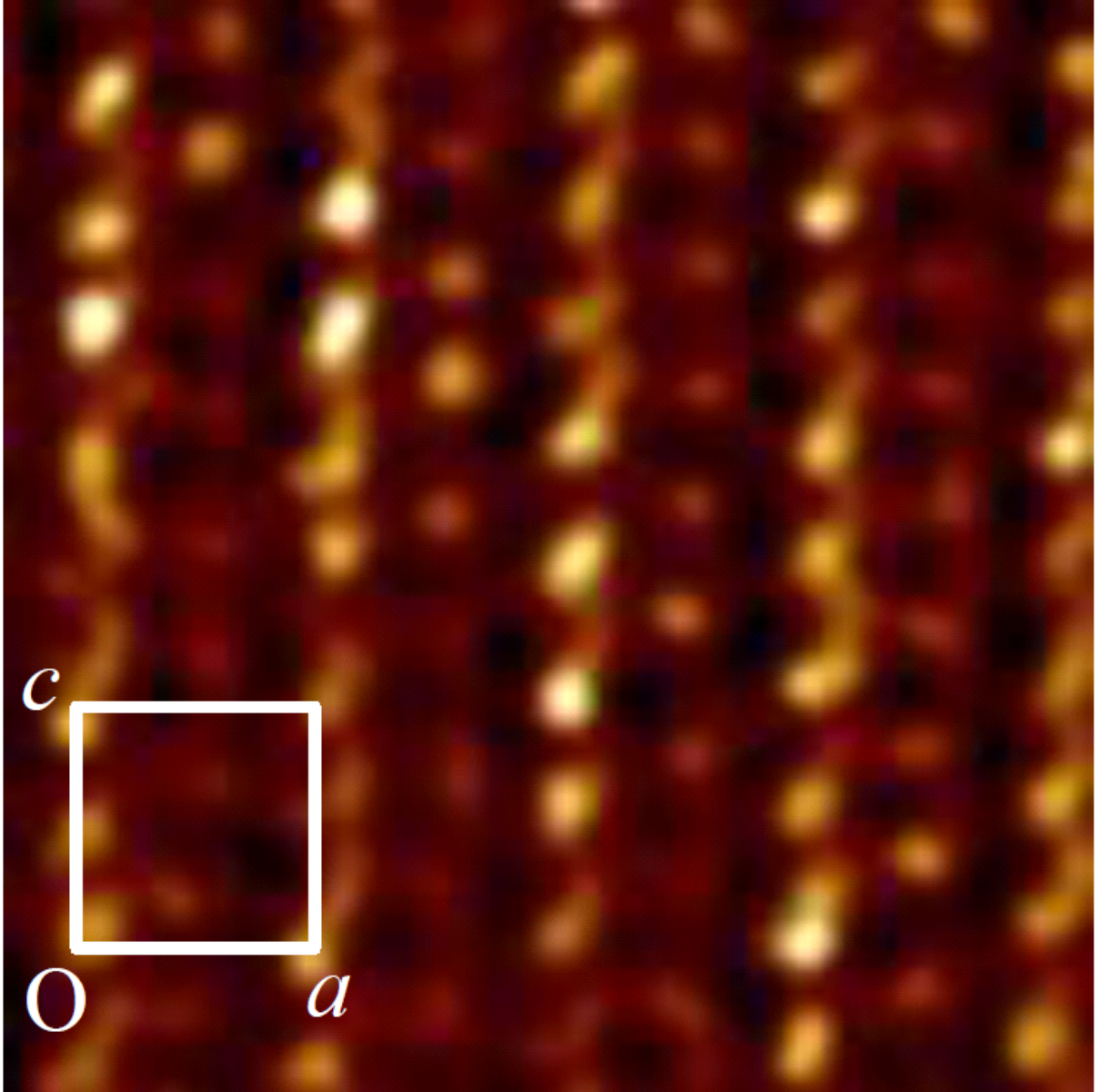
Figure 3.13: STM current image of \alpha -(BEDT-TTF) 2 RbHg(SCN) 4 at tunneling current I = 0.1 nA and bias voltage V = 15 mV with scanning area of 4.3 \text{ nm} \times 4.2 \text{ nm} .
