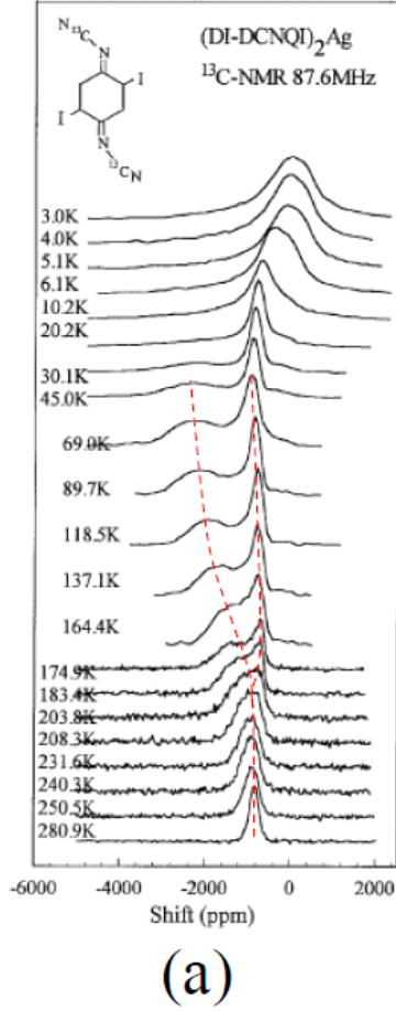
Figure 1.5: (a) ^{13}\text{C} -NMR spectra of (\text{DI-DCNQI})_2\text{Ag} at various temperature [14]. T_{\text{CO}} of (\text{DI-DCNQI})_2\text{Ag} is 220 K. Red break line indicate center of peaks of the spectra continuously. (b) Temperature dependence of magnetic susceptibility of (\text{TMTTF})_2\text{SbF}_6 at constant pressure (\chi_s)_p (circles) and at constant volume (\chi_s)_v (diamonds) [16]. T_{\text{CO}} of (\text{TMTTF})_2\text{SbF}_6 is 157 K.
