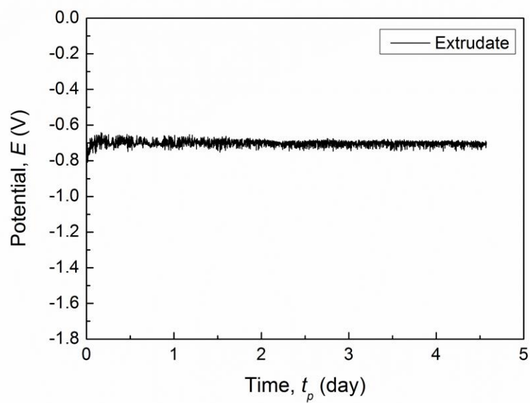
Fig. 2.13 Electrical potential change with respect to immersion time in 3.0 mass% NaCl aqueous solution at room temperature.
