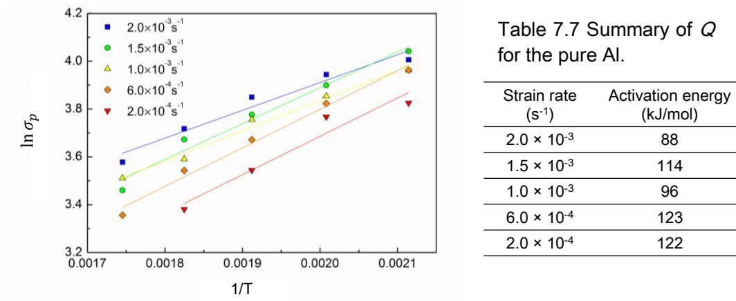
Fig. 7.14 Plots of natural logarithm of true stress versus reciprocal of temperatures for the pure Al.
