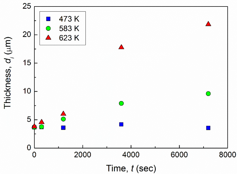
Fig. 2.7 Thickness change of IMC layer during heating at various temperatures.
