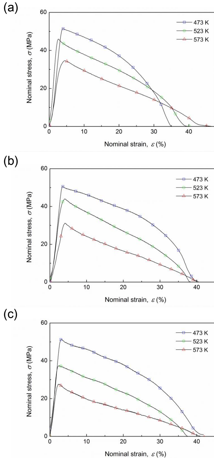
Fig. 7.12 Tensile behavior of the pure Al at various strain rates; (a) 2.0 \times 10^{-3} \text{ s}^{-1} , (b) 1.0 \times 10^{-3} \text{ s}^{-1} and (c) 6.0 \times 10^{-4} \text{ s}^{-1} .
