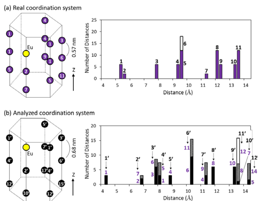
Fig. 7. (a) Real coordination system of Eu sites and (b) analyzed coordination system and its corresponding radial distribution functions.
