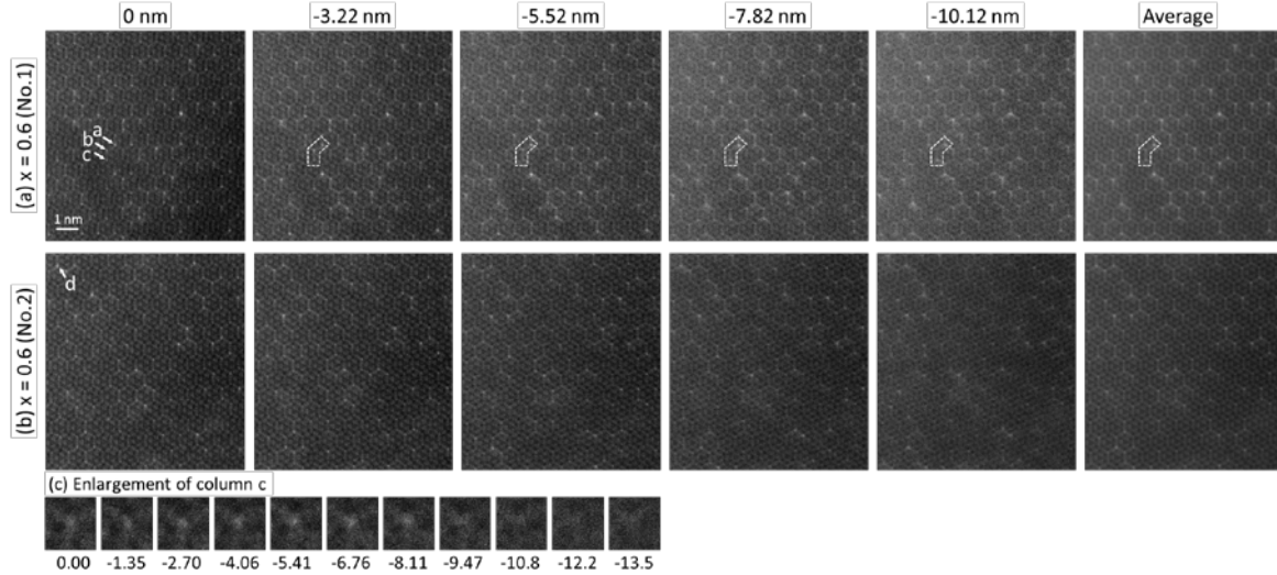
Fig. 4. HAADF-STEM images at different defocus values of Eu doped Ca- \alpha -SiAlON of x = 0.6 No. 1 (a) and No. 2 (b) with averaged HAADF-STEM images, which are the averages of 30 images obtained at different defocus values. (c) Enlargement of column c in Fig. 4(a) at each defocus level (nm).
