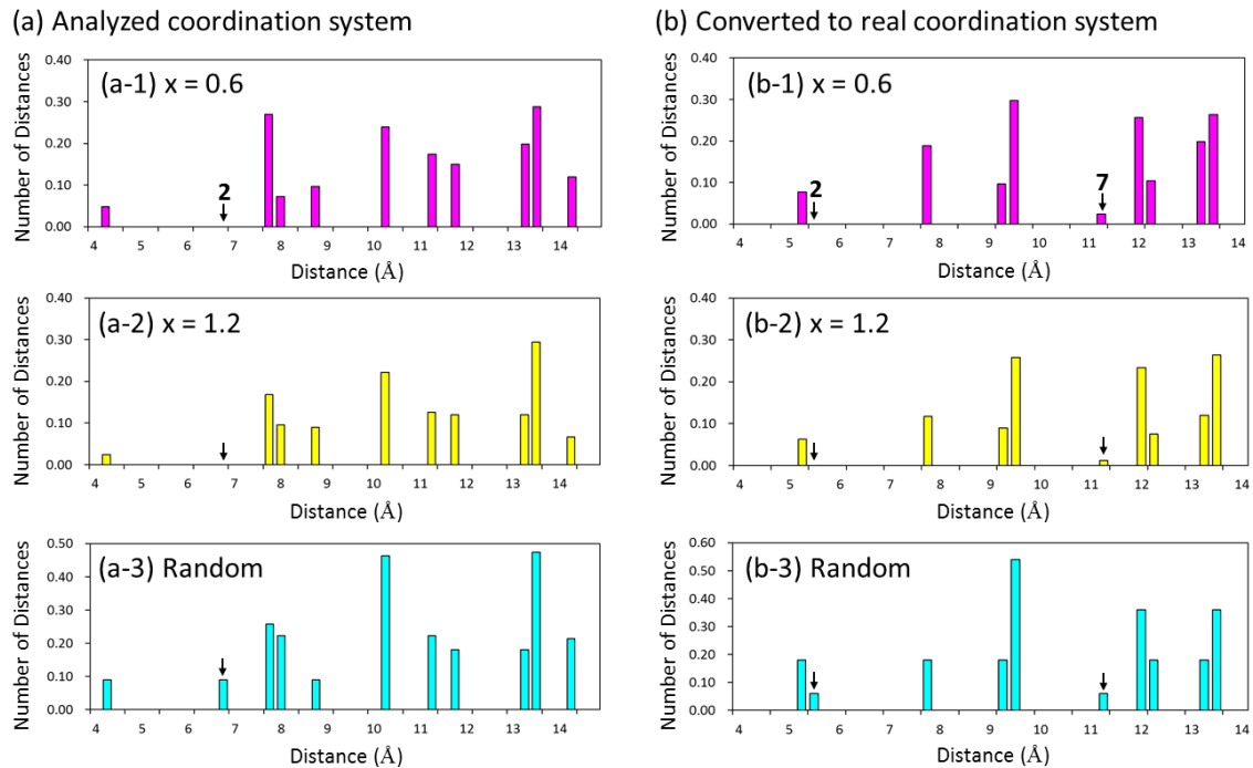
Fig. 8. Radial distribution functions of the analyzed coordination system (a) before and (b) after conversion to the real coordination system.
