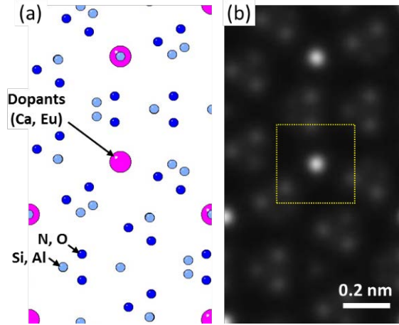
Fig. 1. (a) Atomic structure model of Eu-doped Ca- \alpha -SiAlON, in the [0001] direction. (b) Multi-slice simulated image of Eu-doped Ca- \alpha -SiAlON, in which one Eu atom is located at -5.48 nm along the z -direction and defocus is -5.52 nm (sample thickness: 20 nm, convergence semi-angle: 30 mrad).
