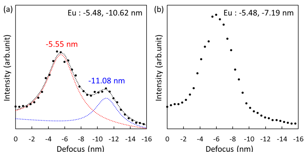
Fig. 3. Defocus profiles via multi-slice image simulation with two Eu atoms located at different depths of (a) -5.48 and -10.62 nm, and (b) -5.48 and -7.19 nm.
