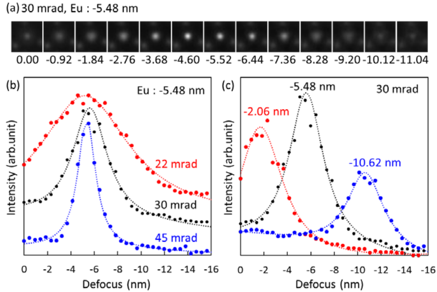
Fig. 2. (a) Simulated images of an Eu site with different levels of defocus from 0.00 to -11.04 nm. (b, c) defocus profiles of an Eu site evaluated via multi-slice simulation with different electron probe convergence semi-angles, and different depth positions of Eu atoms.
