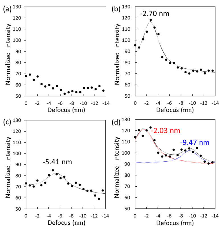
Fig. 5. Contrast profiles acquired from through-focus HAADF-STEM images of Eu-doped Ca- \alpha -SiAlON (x=0.6), in which (a-d) correspond to the arrows in Figs. 4(a, b).
