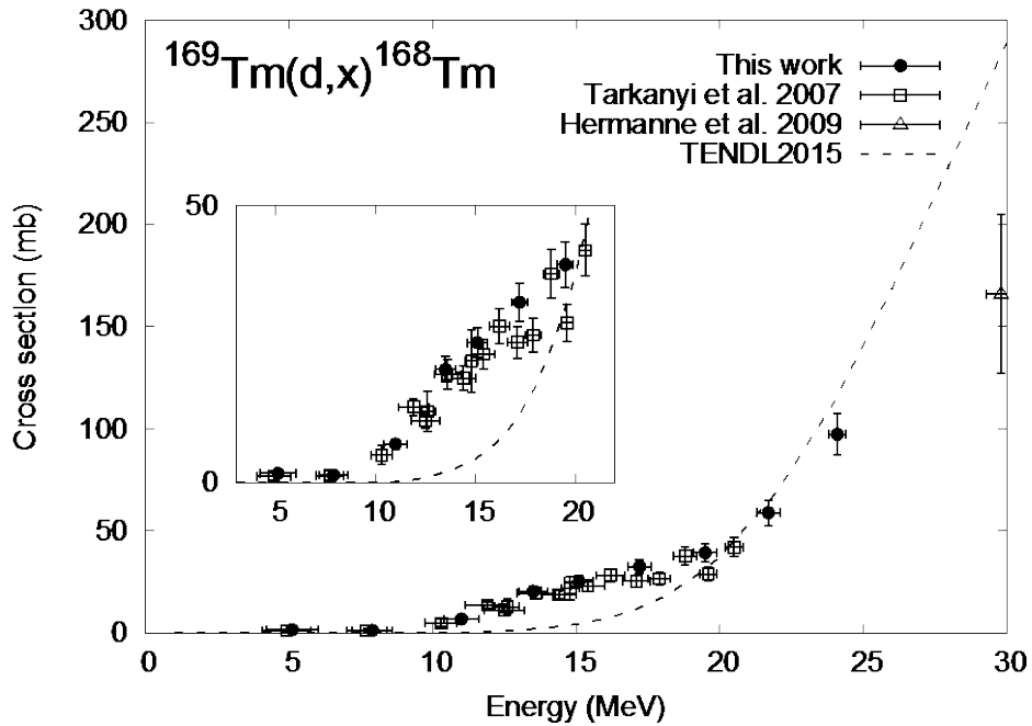
Fig. 4: The excitation function of the ^{169}\text{Tm}(d,x)^{168}\text{Tm} reaction in comparison with the result of the TALYS calculation and the experimental data measured earlier.
