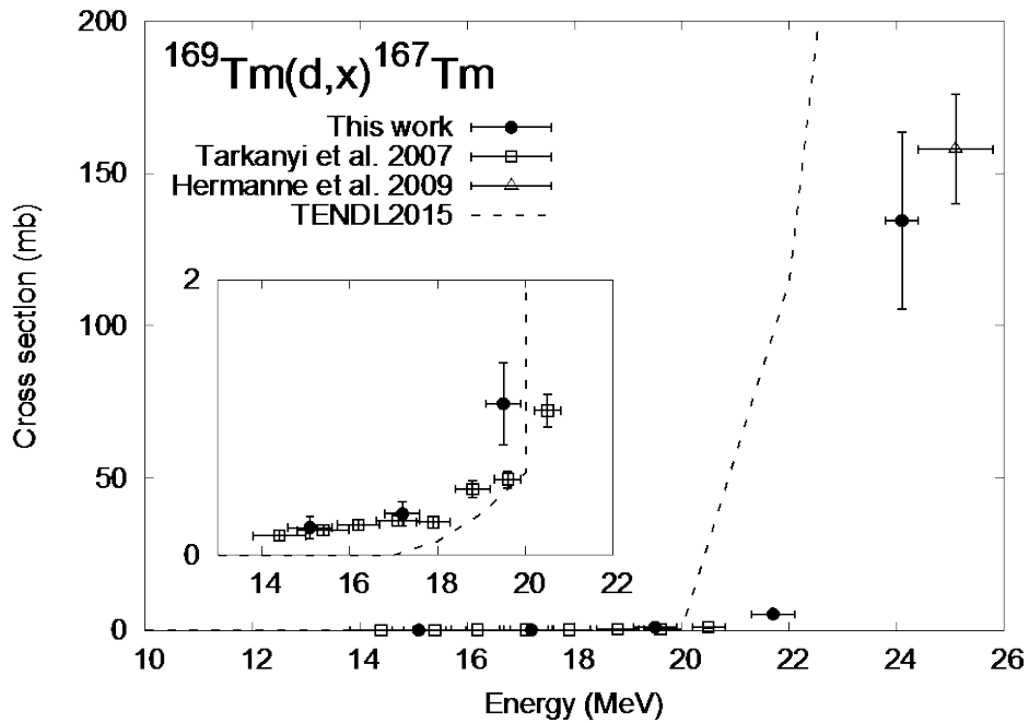
Fig. 5: The excitation function of the ^{169}\text{Tm}(d,x)^{167}\text{Tm} reaction in comparison with the result of the TALYS calculation and the experimental data measured earlier.
