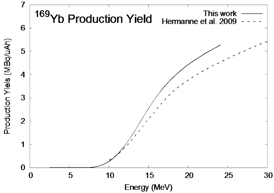
Fig. 6: The production yield of ^{169}\text{Yb} in comparison with the result of the experimental data measured earlier.
