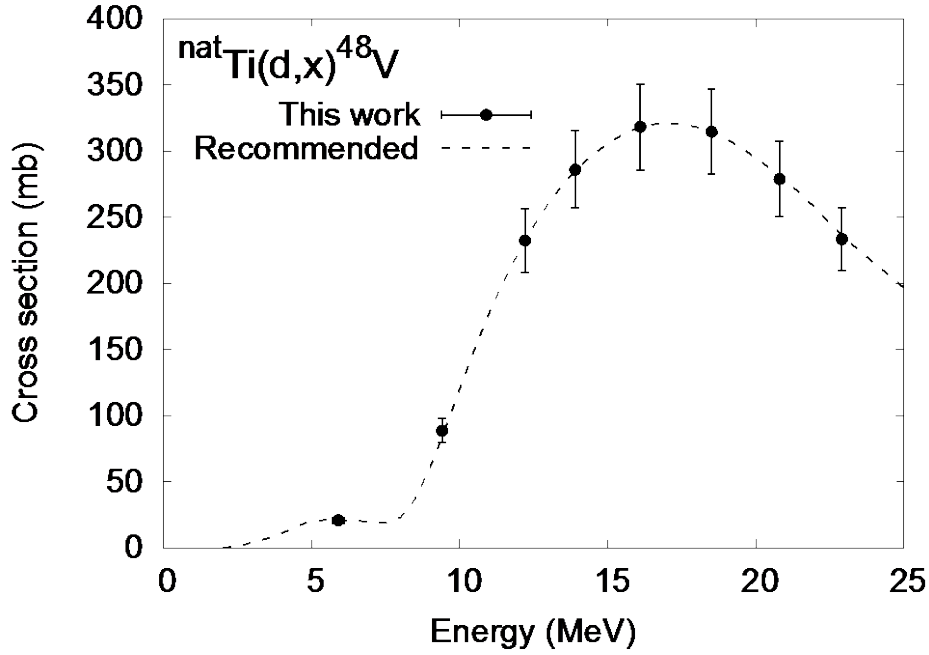
Fig. 1: The excitation function of the monitor reaction {}^{\text{nat}}\text{Ti}(\text{d},\text{x}){}^{48}\text{V} .
