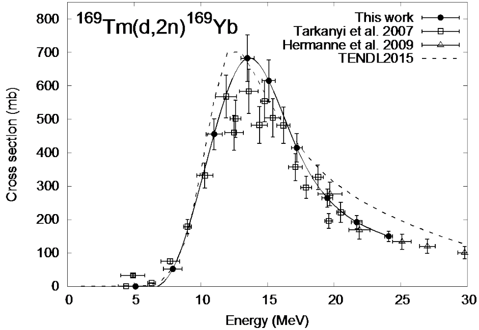
Fig. 2: The excitation function of the ^{169}\text{Tm}(d,2n)^{169}\text{Yb} reaction is shown with a spline fit over the experimental data. The result is compared with the previous experimental data (Tárkányi, 2007; Hermanne, 2009) and TENDL-2015 (TENDL-2015, 2015).
