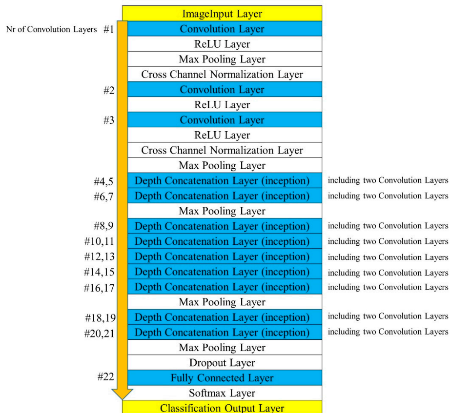
Figure 3. The CNN architecture, which has 22 convolutional layers.
