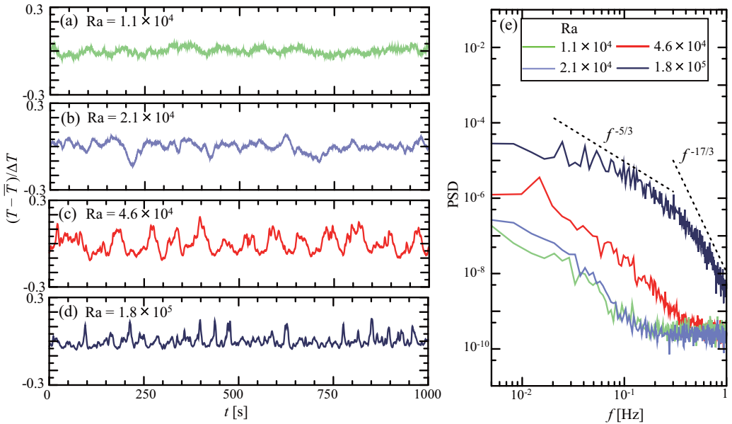
FIG. 9. Temperature fluctuations measured in the fluid layer (see Fig. 1 for the measurement point “T”) at (a) Ra = 1.1 \times 10^4 (four-roll structure), (b) Ra = 2.1 \times 10^4 (four-three transition), (c) Ra = 4.6 \times 10^4 (three-roll structure), (d) Ra = 1.8 \times 10^5 (cellular structure), and (e) PSDs of the temperature fluctuations. The dashed lines indicate the slopes of -5/3 and -17/3 .
