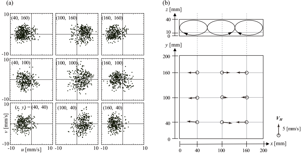
FIG. 4. (a) Scatter diagram of (u, v) at nine intersection points on z = 10 mm, and (b) time-averaged 2D velocity vectors on the horizontal plane, V_H (\bar{u}, \bar{v}) , with a schematic image representing a side view of the rolllike structure expected from the results; Ra = 4.6 \times 10^4 and “three-roll structure” regime.
