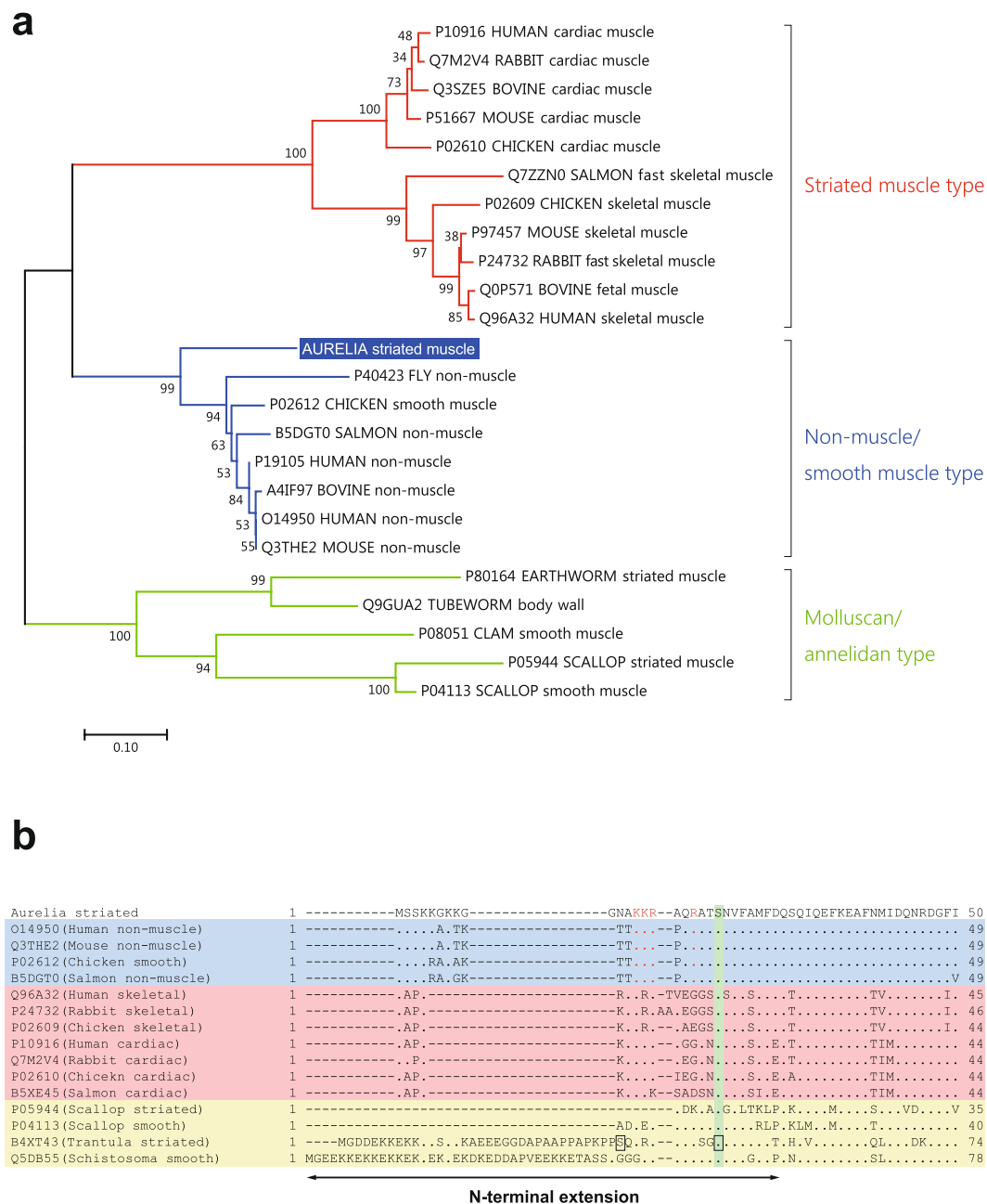
Figure 4. Neighbor-joining analysis of myosin regulatory light chain (MRLC) proteins. (a) Neighbor-joining tree generated with amino acid sequences of MRLC proteins. The accession numbers of amino acid sequences in the UniProtKB/TrEMBL are shown. (b) Comparison of N-terminal sequences. The N-terminal extension (NTE) is indicated. Residues identical to those of the Aurelia MRLC are represented by dots. The serine residues known to be primarily phosphorylated by myosin light chain kinase (MLCK) in vertebrate smooth muscles are shaded in green. The sequences of the non-muscle/smooth, striated, and invertebrate MRLC are shaded in blue, red, and yellow, respectively. Ser35 and Ser45 of tarantula striated muscle MRLC, which are reported to be phosphorylated, are boxed. The basic four residues important for the substrate recognition by smooth muscle MLCK are indicated in red font.
