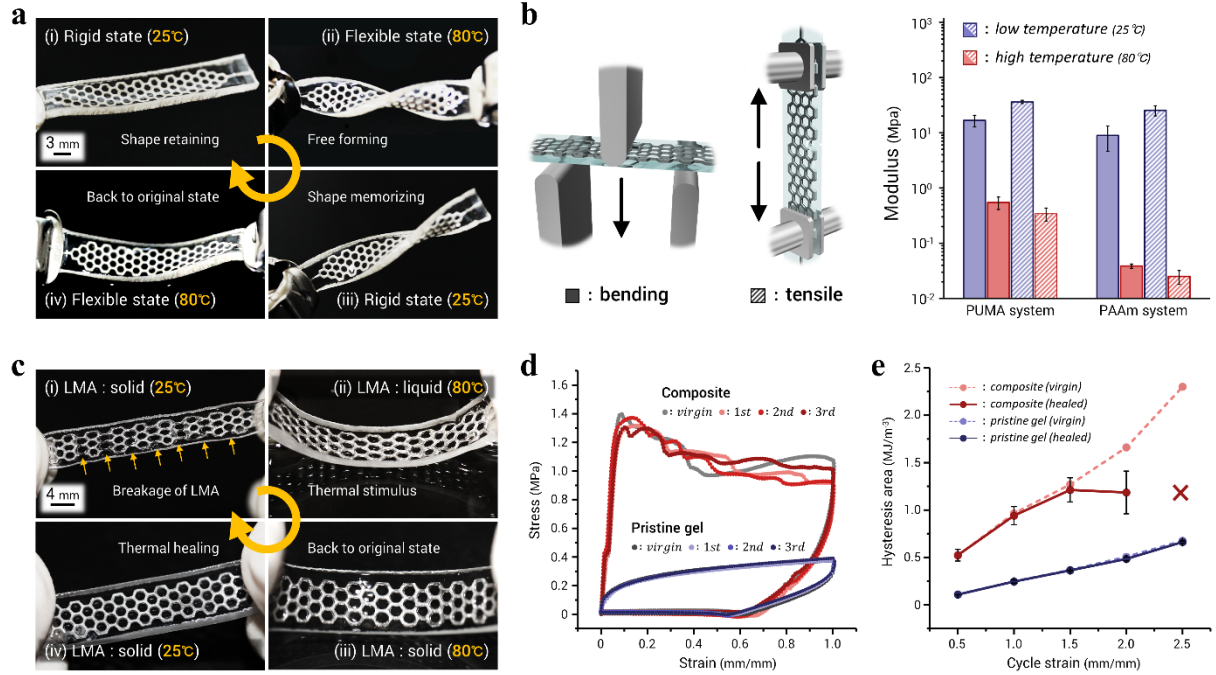
Figure 3. Thermal response and thermal healing of PUMA-LMA composites. (a) Demonstration of shape memory based on the solid-liquid phase transition of the LMA skeleton. (b) Bending (solid shade) and tensile (hashed) moduli of the composite at low (25°C, blue) and high (80°C, red) temperature. (c) Demonstration of thermal healing ability at a strain ratio of approximately 1.5. Inset arrows in (i) represent the broken points of the internal LMA skeleton. (d) Cyclic test curves of composite and pristine PUMA gels. (e) Mechanical hysteresis loss during loading and unloading testing at various strains (0.5-2.5). The data for the healed composite at a strain of 2.5 was not measured due to damage of the sample during the first cycle. Each measurement was performed 3-7 times. Error bars represent standard deviation, and are smaller than the marker unless explicitly shown.
