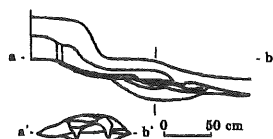
Sections of "kamado" in the pit-house №41.
