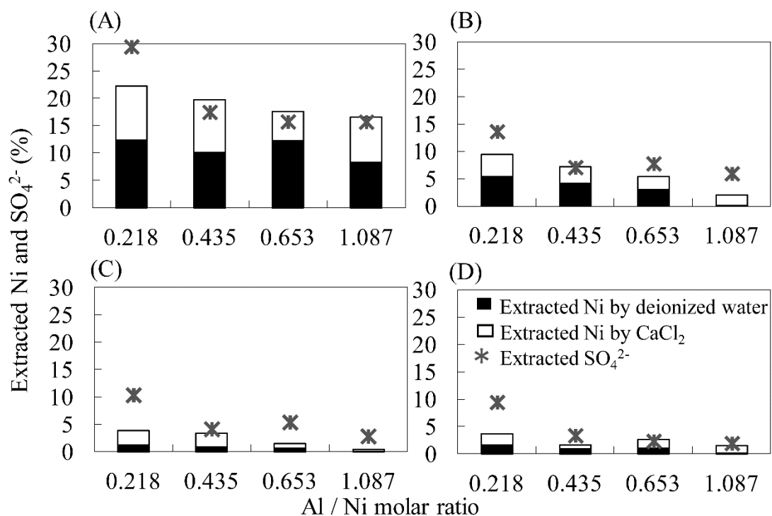
Fig. 5. Percentage of extracted and adsorbed fractions of Ni and \text{SO}_4^{2-} in the experiment with 200 mg/L Ni ion at (A) pH 5, (B) pH 6, (C) pH 7, and (D) pH 8.
