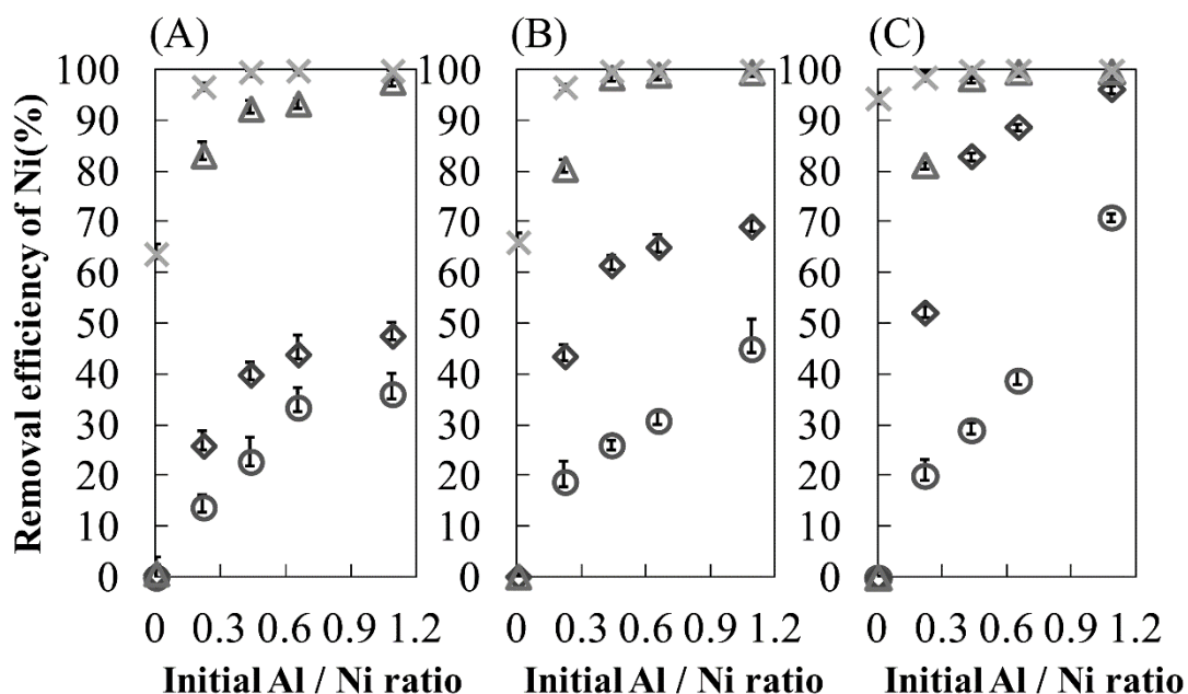
Fig. 1. Removal efficiency, with one standard deviation from the mean, of Ni at pH 5 (○), pH 6 (◊), pH 7 (△), and pH 8 (×). The initial Ni concentration is (A) 200 mg/L, (B) 1000 mg/L, and (C) 10000 mg/L.
