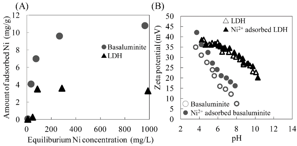
Fig. 4. (A) Adsorption isotherm of Ni for synthesized basaluminite and LDH and (B) zeta potential of the LDH and basaluminite before and after adsorption the experiments as a function of pH.
