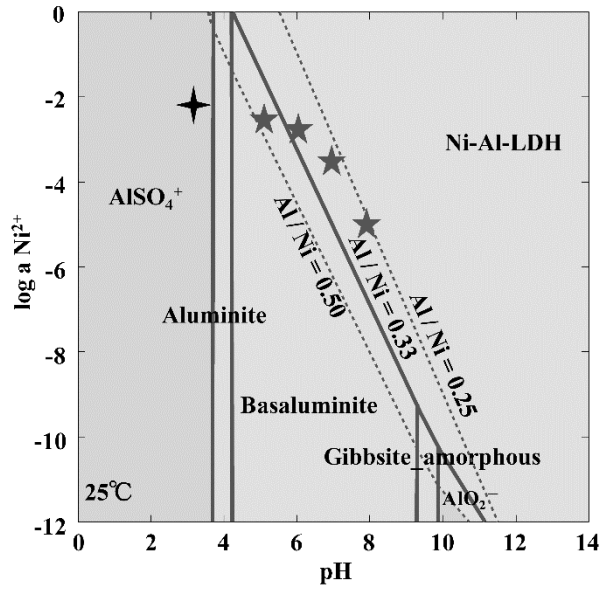
Fig. 6. Stability diagram of Al minerals in the Ni-Al-SO 4 -H 2 O system (Ni 200 mg/L, Al/Ni=0.435). Initial solution (+) and solution at 5–8 after co-precipitation(★).
