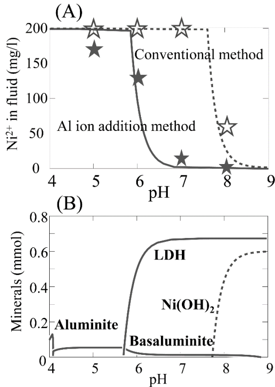
Fig. 7. Reaction models for Ni 2+ in fluid (A) and minerals (B) in the conventional method and the Al ion addition method. Ni 2+ 200 mg/L, Al 3+ 40 mg/L, and SO 4 2- 5.6 mmol/L (—); Ni 2+ 200 mg/L,
