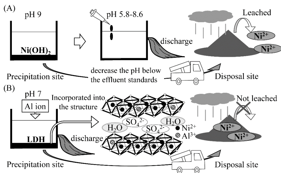
Fig. 9. Behavior of \text{Ni}^{2+} at the precipitation and disposal sites in (A) conventional method and (B) Al ion addition method.
