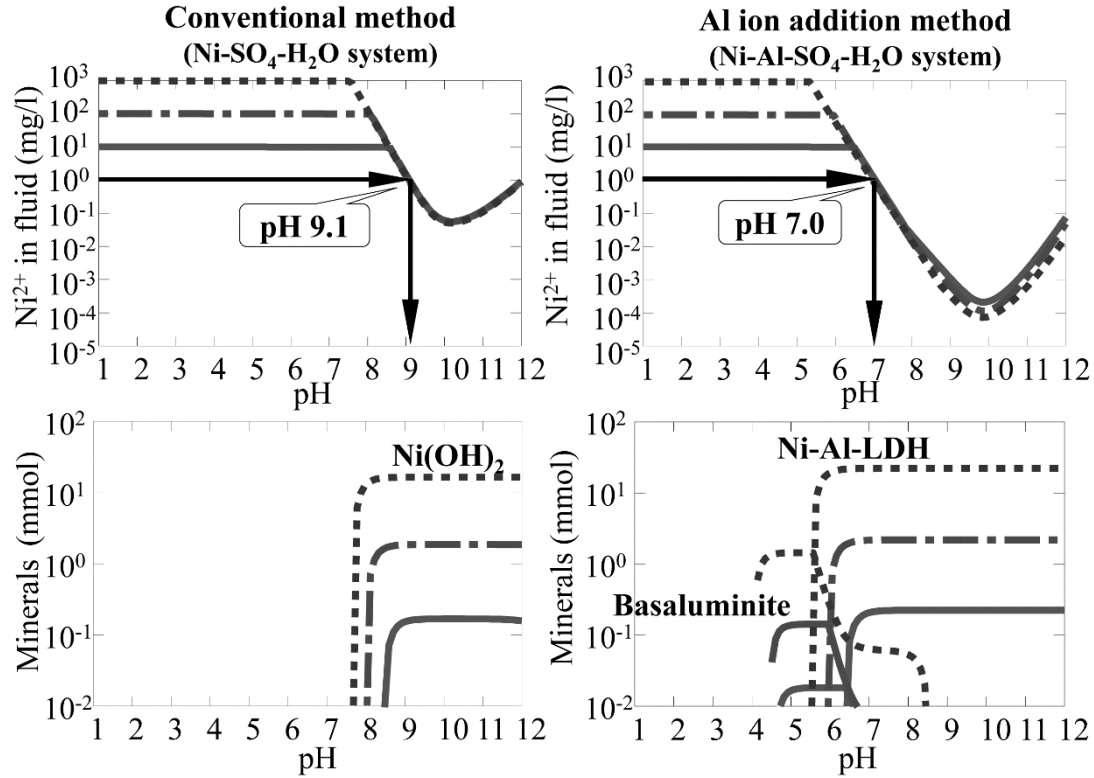
Fig. 10. Reaction models for \text{Ni}^{2+} in the fluid and minerals in (left) the conventional method and (right) the Al ion addition method with ( \text{SO}_4^{2-} 1000 mg/L) at 25°C. The broken arrows in the top row shows where the target Ni concentrations are achieved. Left panels (conventional method): \text{Ni}^{2+} 10 mg/L (—), \text{Ni}^{2+} 100 mg/L (— · —), and \text{Ni}^{2+} 1000 mg/L (·· ·) of the initial solutions. Right panels (Al ion addition method): \text{Ni}^{2+} 10 mg/L and \text{Al}^{3+} 2 mg/L (—), \text{Ni}^{2+} 100 mg/L and \text{Al}^{3+} 16 mg/L (— · —), and \text{Ni}^{2+} 1000 mg/L and \text{Al}^{3+} 160 mg/L (·· ·) of the initial solutions
