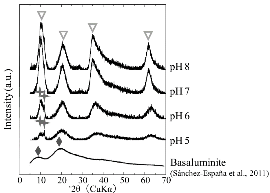
Fig. 2. X-ray diffraction patterns of precipitates (Ni = 200 mg/L, Al/Ni = 0.435) after co-precipitation. Crystalline phases: (∇) Ni-Al-LDH, (◊) basaluminite, and (+) aluminite.
