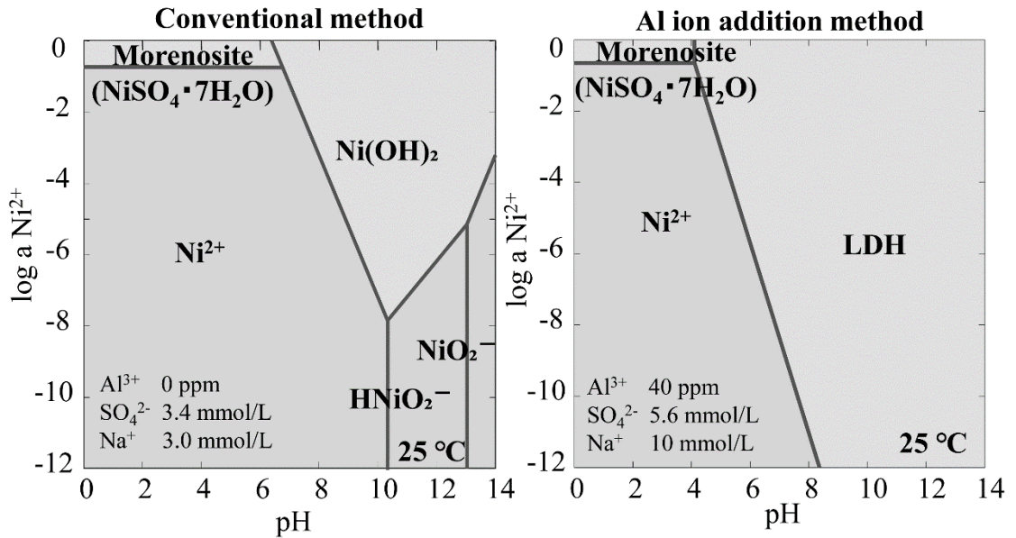
Fig. 8. Stability diagrams of (left panel) the conventional method (Ni-SO 4 -H 2 O system) and (right panel) the Al ion addition method (Ni-Al-SO 4 -H 2 O system).
