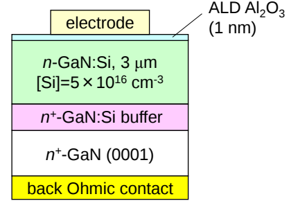
Figure 1 Structure of sample with Al 2 O 3 interlayer.
