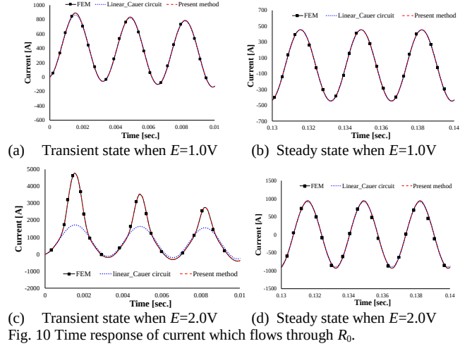
Fig. 10 Time response of current which flows through R_0 .
