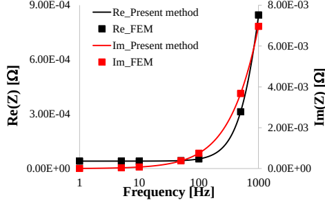
Fig. 8 Frequency response of impedance of the induction heating TABLE II Element values of Induction Heating in Cauer circuit.
