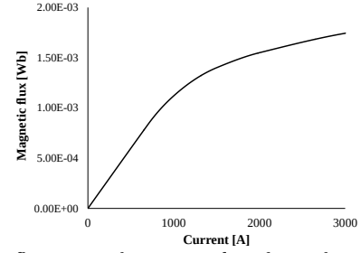
Fig. 9 Magnetic flux-current characteristic for induction heating.
