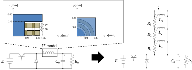
Fig. 3 Inductor in DC-DC converter.
