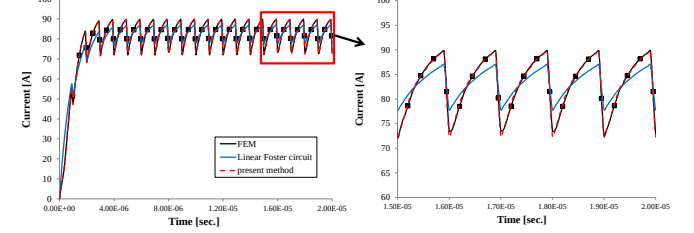
(a) E=5.0\text{V} , C_0=1\mu\text{F}
