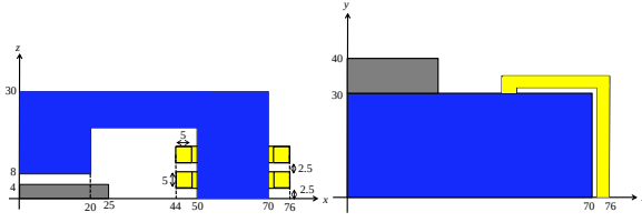
Fig. 7 Induction heating model (blue : magnetic core, yellow : coil, gray : conducting plate)
