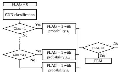
Fig. 4. Flow diagram of fitness evaluation
