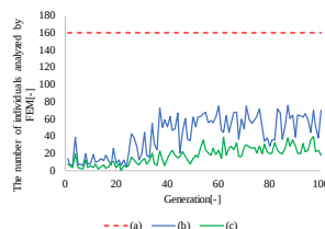
Fig. 8. Number of FEM evaluation
