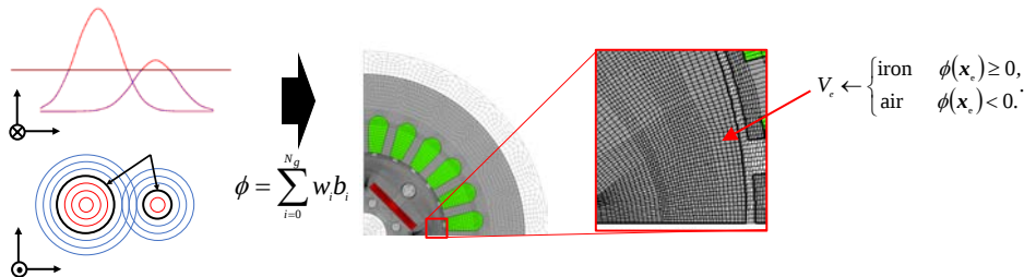
Fig. 1. NGnet-on/off method.
