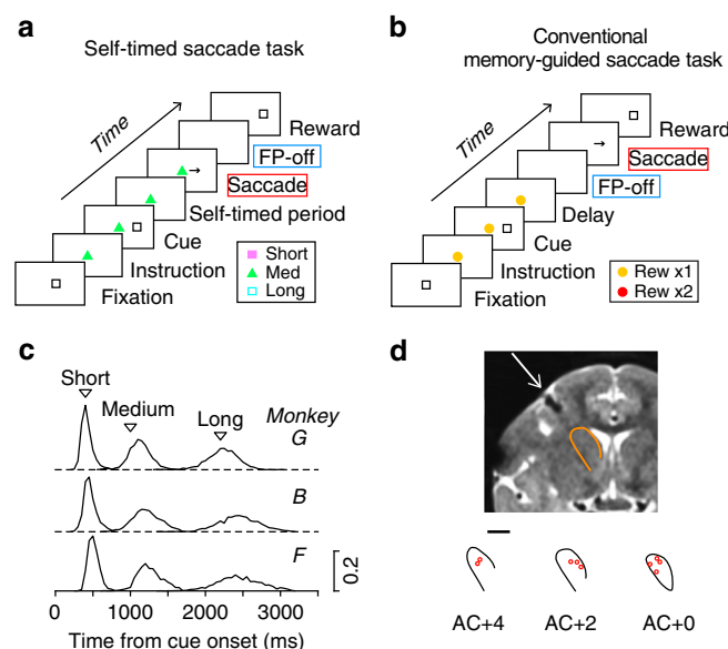
Fig. 1 Behavioral paradigms and the locations of recording sites. a In the self-timed saccade task, monkeys were trained to generate a self-initiated saccade to the location of a briefly presented visual cue (100 ms) after the mandatory delay interval (400, 1000, or 2200 ms). b In the conventional memory-guided saccade (MS) task, animals made a saccade in response to the fixation point (FP) offset that occurred 800–2500 ms after the visual cue. Each task condition was indicated by specific color and shape of the FP, and the stimulus set for monkey F is shown here. A different set of the FP color and shape was used for the other two monkeys (see Methods). The visual cue appeared 800–1700 ms following the onset of this instruction. c Distributions of self-timed saccade latency during LFP recording in three monkeys ( n = 3225 , 4373, and 4588 trials for monkeys G, B, and F, respectively). Inverted triangles indicate the minimal mandatory intervals to obtain reward. d Coronal MR image (AC + 2) and recording sites (red circles) in monkey F. Scale bar represents 5 mm. Recording sites were reconstructed from histological sections in monkey G (Supplementary Figure 1). AC, anterior commissure
