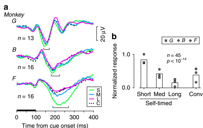
Fig. 2 Contextual modulation of visually evoked potentials. a Time courses of striatal LFPs aligned with the cue onset in the contralateral visual field. Colored traces indicate the self-timed trials with different interval conditions. Black dashed traces indicate the conventional MS trials. The horizontal black bar denotes the timing of cue presentation. Brackets indicate the ranges of maximal response timing. b Comparison of the magnitude of visually evoked response. Each bar summarizes normalized response obtained from 45 sites. Different symbols plot the means of different monkeys. A one-way repeated measures ANOVA revealed a statistically significant difference across the interval conditions ( F_{2,88} = 50.4 , p < 10^{-14} ). Conv, conventional memory-guided saccade (MS) task
