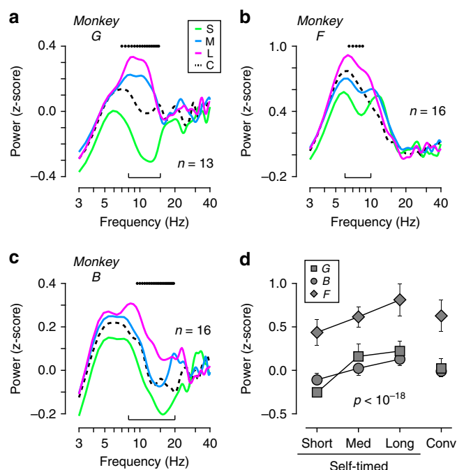
Fig. 5 Spectral analysis of LFP during the pre-cue period. a–c Power spectra for monkeys G ( a , n = 13 sites), F ( b , n = 16 ), and B ( c , n = 16 ). On each panel, black dots above the traces represent a significant difference across the interval conditions (one-way factorial ANOVA, 2 Hz bin with 0.5 Hz step, p < 0.01 , see Methods). Brackets denote the frequency bands used for further quantification. d Comparison of the powers of low-frequency components. Different symbols denote different animals. Error bars indicate 95% CIs. The LFP power differed significantly across the interval conditions (repeated measures ANOVA, F_{2,88} = 71.5 , p < 10^{-18} )
