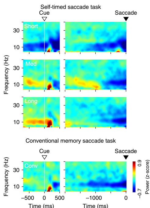
Fig. 3 Color-coded power spectra of LFP in monkey G ( n = 13 sites) for the self-timed and the conventional MS tasks. Zero in the abscissa indicates either the cue onset (left panels) or saccade initiation (right). Data for the other two monkeys are shown in Supplementary Figure 2
