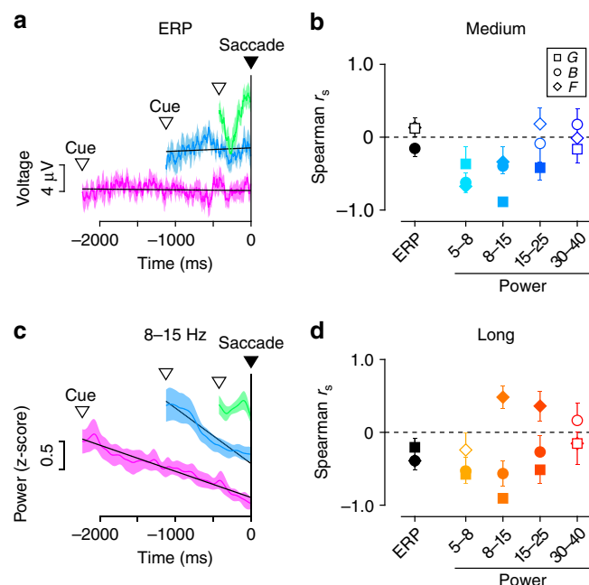
Fig. 4 Temporally variable LFP components during the self-timed period in the self-timed task. a Time courses of event-related potentials (ERP) during saccade preparation in monkey G ( n = 13 sites). Green, blue, and magenta traces indicate the means ( \pm 95\% CIs) for the short, medium, and long interval conditions, respectively. Inverted open triangles indicate the means of cue onset time relative to saccades. The traces are shifted vertically for presentation purpose only. Black lines indicate linear regressions for the average traces in the medium and long interval conditions. b Spearman's rank correlation coefficients ( r_s ) computed between time (10 bins) and ERP or the power of different LFP components in the medium interval (1000 ms) condition. Different shapes of symbols represent different animals. Filled symbols indicate the data showing a significant difference from zero (one-sample t -test, n = 13 or 16 , p < 0.05 ). Error bars indicate 95% CIs. c Similar configuration as in a , but for the time courses of LFP power at 8–15 Hz. d Rank correlation coefficients computed for the long interval (2200 ms) condition
