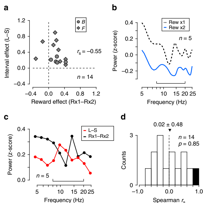
Fig. 6 Effects of reward amount on the striatal LFP. a Comparison between the effects of reward amount and delay interval. Each point represents single site and compares the alteration in power at the low-frequency bands indicated by brackets in Fig. 5b, c. b Effects of reward amount for a broader frequency band in monkey B ( n = 5 sites). The bracket indicates the frequency band used for the analysis in a . c Comparison of spectral modulation associated with interval condition (red, Long minus Short) with that associated with reward amount (black, Reward \times 2 minus \times 1 ). Data were divided into 10 groups. d Distribution of rank correlation coefficients computed for the two power spectra shown in c for individual sites in two monkeys. The black bar indicates statistically significant correlation ( p < 0.05 ). Overall, the values were not statistically different from zero (two-tailed t -test, t_{13} = 0.19 , p = 0.85 )
