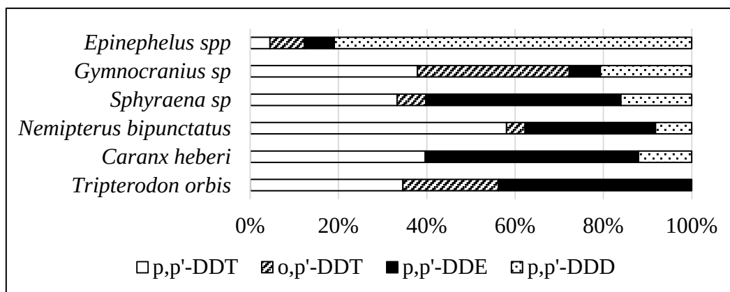
Figure 2 Relative abundance of DDT congeners in marine fish from Maputo Bay, Mozambique.
