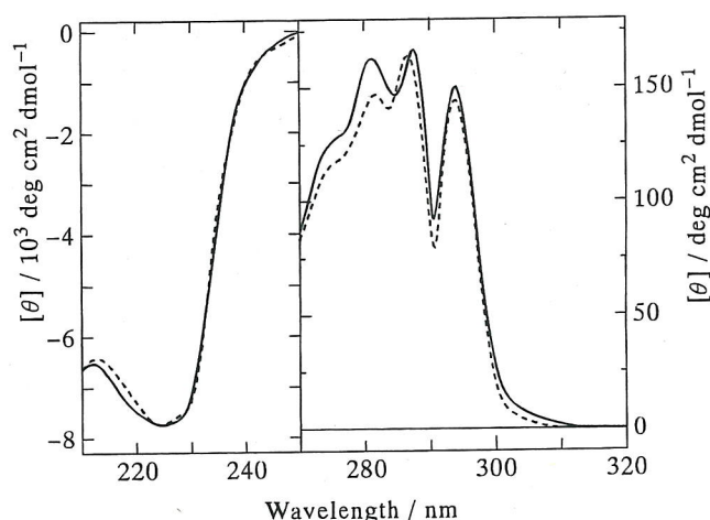
Fig. 3. Circular dichroism spectra of canine milk lysozyme. Solid line: apolysozyme in 0.1 M TES (pH 7.2), 0.1 M KCl, 1 mM EDTA. Dashed line: holo-lysozyme in 0.1 M TES (pH 7.2), 0.1 M KCl, 1 mM EDTA, 2 mM CaCl_2 .
