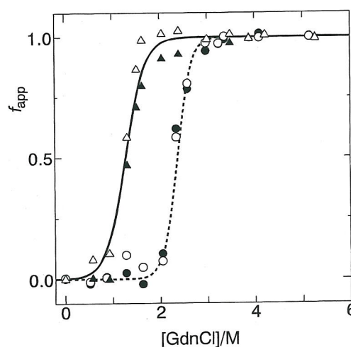
Fig. 4. GdnCl induced transition curves of echidna milk lysozyme in 0.1 M TES buffer (pH 7.2, 25°C). Triangles: apolysozyme with 1 mM EDTA. Circles: holo-lysozyme with 1 mM EDTA and 2 mM CaCl_2 . Open and filled symbols illustrate the values of f_{app} calculated from the ellipticity at 294 and 222 nm, respectively. Lines were calculated with the parameters obtained with Equation 2.
