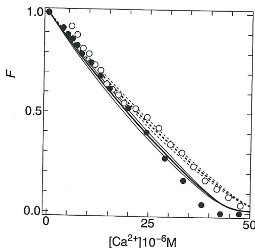
Fig. 1. Titration of Quin-2 in the presence of EML (open circles) and CML (filled circles). Free fraction ( F ) of Quin-2 is plotted against the total concentration of calcium ions. The concentrations of Quin-2 were 15.5 \mu M for EML and 13.5 \mu M for CML, respectively. The concentrations of lysozymes were 34.5 and 26.6 \mu M for EML and CML, respectively. Thick lines are the best fitted curves calculated with the parameters listed in Table 1 by Equation 1. Accompanying thin lines are calculated using the binding constants 1 \times 10^6 M less/more than the best fitted values.
