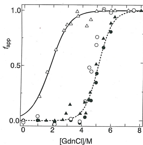
Fig. 5. GdnCl induced transition curves of canine milk lysozyme in 0.1 M TES buffer (pH 7.2, 25 °C). Triangles: apolysozyme with 1 mM EDTA. Circles: holo-lysozyme with 1 mM EDTA and 2 mM CaCl 2 . Open and filled symbols illustrate the values of f_{app} calculated from the ellipticity at 294 and 222 nm, respectively. Lines were calculated with the parameters obtained from Figure 6 and shown in Table 3.
