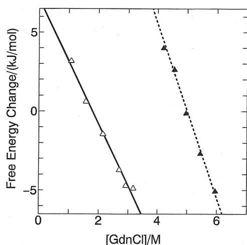
Fig. 6. GdnCl concentration dependence of the free energy changes of the unfolding of canine apolysozyme. Symbols are the same as in Figure 5.
