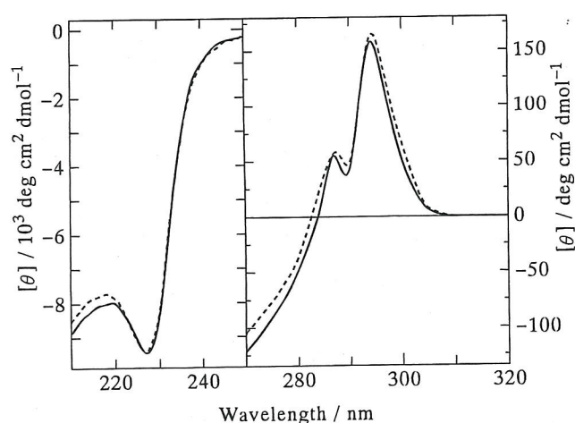
Fig. 2. Circular dichroism spectra of echidna milk lysozyme. Solid line: apolysozyme in 0.1 M TES (pH 7.2), 0.1 M KCl, 1 mM EDTA. Dashed line: holo-lysozyme in 0.1 M TES (pH 7.2), 0.1 M KCl, 1 mM EDTA, 2 mM CaCl_2 .
