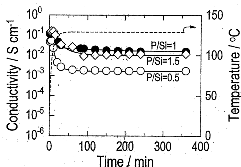
Fig. 2. Variations in conductivities of the phosphosilicate gels containing various amounts of phosphorus with holding time at 130^\circ\text{C} for 400 min. The R.H. of the measuring atmosphere was 0.7%, and the broken line has the same meaning as in Fig. 1. Open circles, closed circles and open diamonds represent phosphosilicate gels with the P/Si molar ratios of 0.5, 1.0 and 1.5, respectively.
