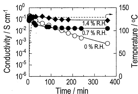
Fig. 3. Variations in conductivities with holding time under 0 (open circles), 0.7 (closed circles) and 1.4 (closed diamonds) % R.H. at 130°C for the gels with the P/Si molar ratio of 1.0. The broken line has the same meaning as in Fig. 1.
