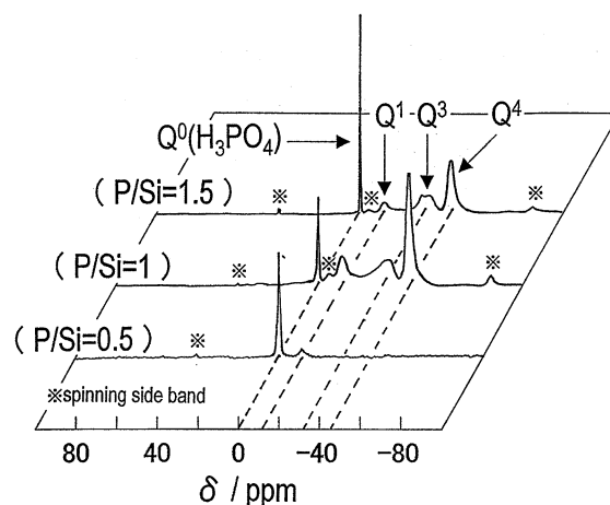
Fig. 4. ^{31}\text{P} MAS NMR spectra of phosphosilicate gels, which were heat-treated at 150°C for 5 h, with the P/Si molar ratios of 0.5, 1.0 and 1.5.
