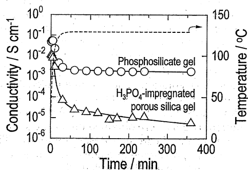
Fig. 1. Variations in conductivities of the phosphosilicate (open circles) and \text{H}_3\text{PO}_4 -impregnated porous silica (open triangles) gels with holding time at 130^\circ\text{C} for 400 min. The R.H. of the measuring atmosphere was 0.7%. The temperature profile for the samples is shown by the broken line.
