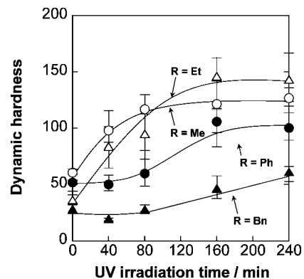
Fig. 4. Changes in dynamic hardness of the 80\text{RSiO}_{3/2}\cdot 20\text{TiO}_2 ( R = \text{Me} , Et, Ph and Bn) hybrid films with UV irradiation. Error bars show the range between the maximum and minimum values of the repeated measurements.
