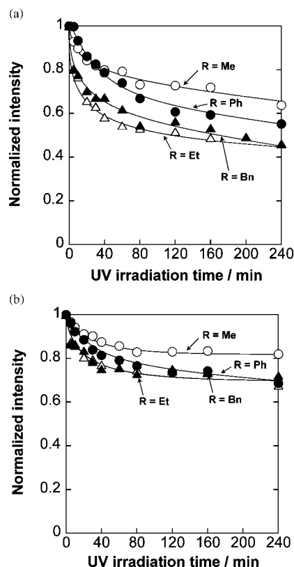
Fig. 1. Changes in the normalized intensities of the absorption peaks assigned to (a) Si-C and (b) Si-O-Ti bonds in the FT-IR spectra of 80\text{RSiO}_{3/2} \cdot 20\text{TiO}_2 ( R = \text{Me, Et, Ph and Bn} ) hybrid films with UV irradiation. The intensities of the absorption peaks were normalized with those of the film before the irradiation.
