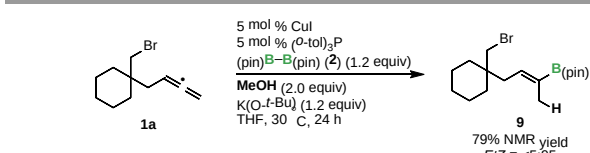
Scheme 3 Protonolysis of the allylcopper(I) intermediate.
