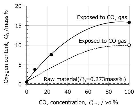
Fig. 13 Oxidation behavior of Ti powder under various gases.
