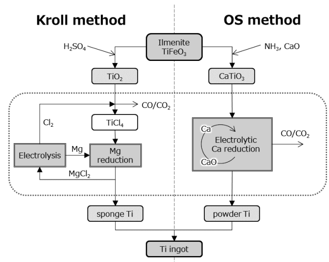
Fig. 2 Flowsheet of designed procedure starting from Ilmenite to Ti ingot via \text{CaTiO}_3 in comparison with Kroll process.
