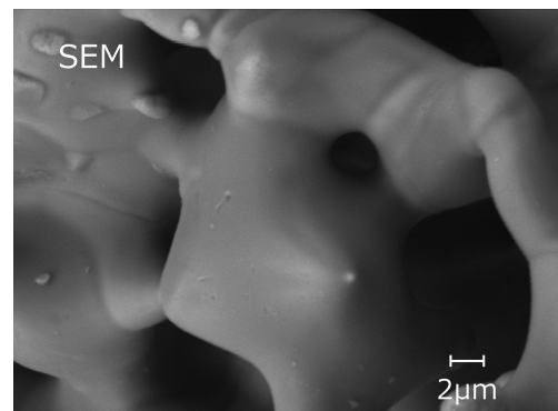
Fig. 11 SEM image of the reduced sample (#F), to which Q/Q_0 = 600\% was given. The sample was cooled in EX-Ar.
