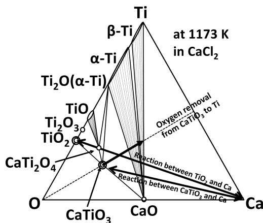
Fig. 1 Phase equilibria in \text{Ca-Ti-O} system coexisted with \text{CaCl}_2 melt 30 . Reduction route from \text{CaTiO}_3 to metallic Ti is inserted when oxygen is removed as \text{CaO} .
