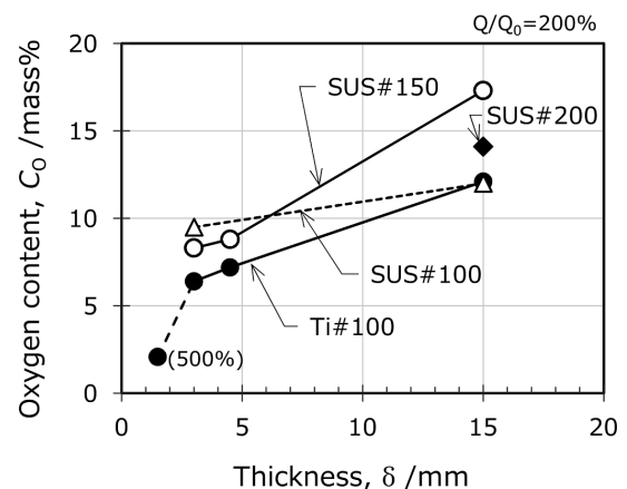
Fig. 6 Residual oxygen in the cathodic powder.
