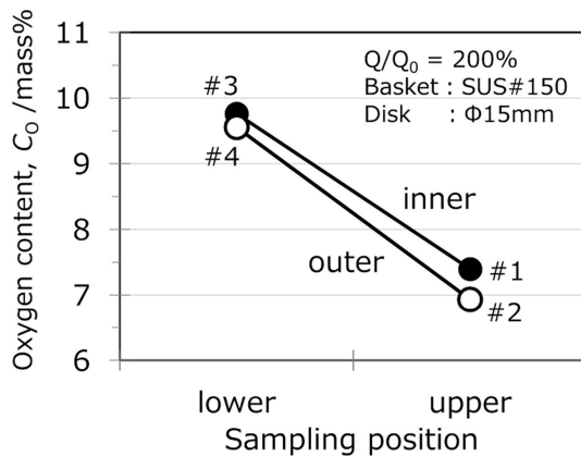
Fig. 4 Oxygen contents in the sample reduced at Q/Q_0 = 200\% .
