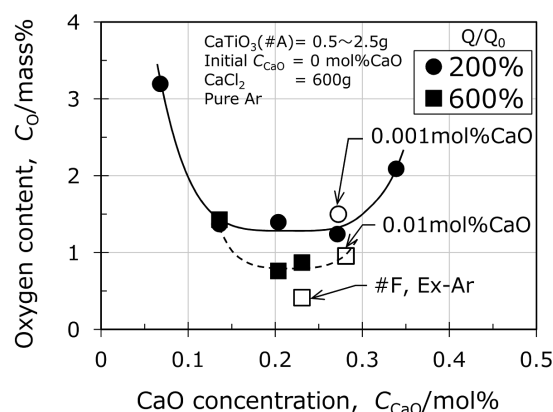
Fig. 8 \text{CaO} concentration dependency of oxygen concentration in the obtained sample after the electrolysis at Q/Q_0 = 200 and 600\% .
