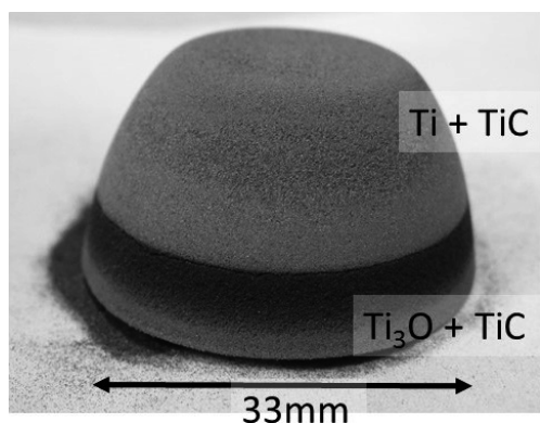
Fig. 12 Photo of the Ti powder after picked up from the cup-type alumina crucible. The powder was heated in \text{CO}_2 gas at 1173 K for 7.2 ks, and the bottom side of slightly sintered powder was reversed for photography.
