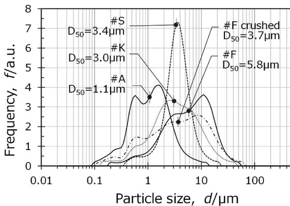
Fig. 9 Particle size distribution of \text{CaTiO}_3 powders from four producers, #A, #K, #S and #F.
