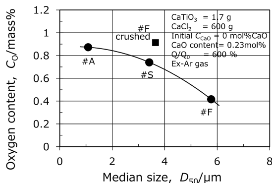
Fig. 10 Particle size dependency of oxygen concentration in the obtained sample after the electrolysis at Q/Q_0 = 600\% .
