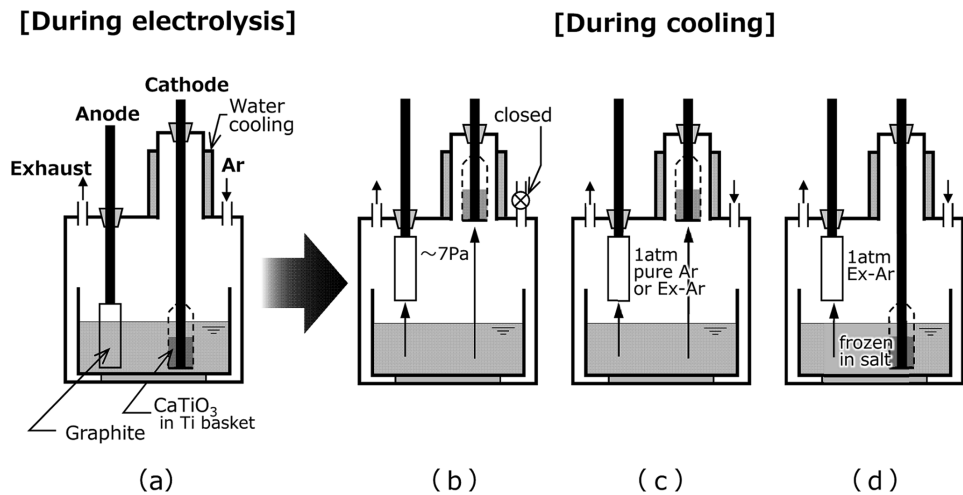
Fig. 14 (a) experimental setup during electrolysis, (b) cooling in vacuum where the cathode was cooled at the upper part, (c) cooling in pure Ar or Ex-Ar, and (d) cooling in the frozen salt.
