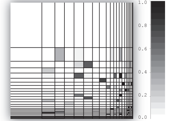
(f) Enron (RDIRM)
