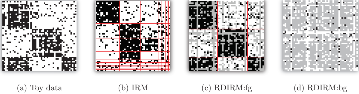
Figure 3.2: Toy data example: (a) synthetic 50 \times 50 relational data (white corresponds to zero, and black corresponds to one); (b) IRM solution (rows and columns are sorted by obtained cluster indices); (c) and (d) RDIRM solutions: (c) shows the area assigned to foreground ( r_{i,j} = 1 ), and (d) shows the area assigned to background ( r_{i,j} = 0 ) (gray area indicates that the corresponding entries are assigned to another layer).
