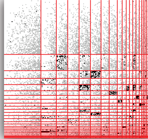
(f) Enron (RDIRM), TDLL = -0.046
