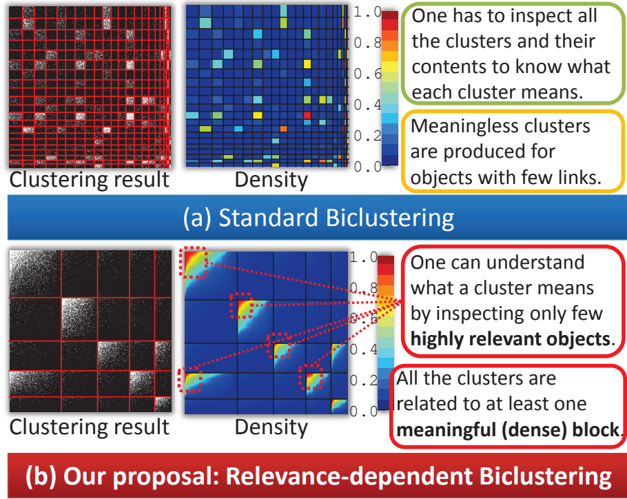
Figure 1.1: Diagrams of (a) standard biclustering and (b) relevance-dependent biclustering.
