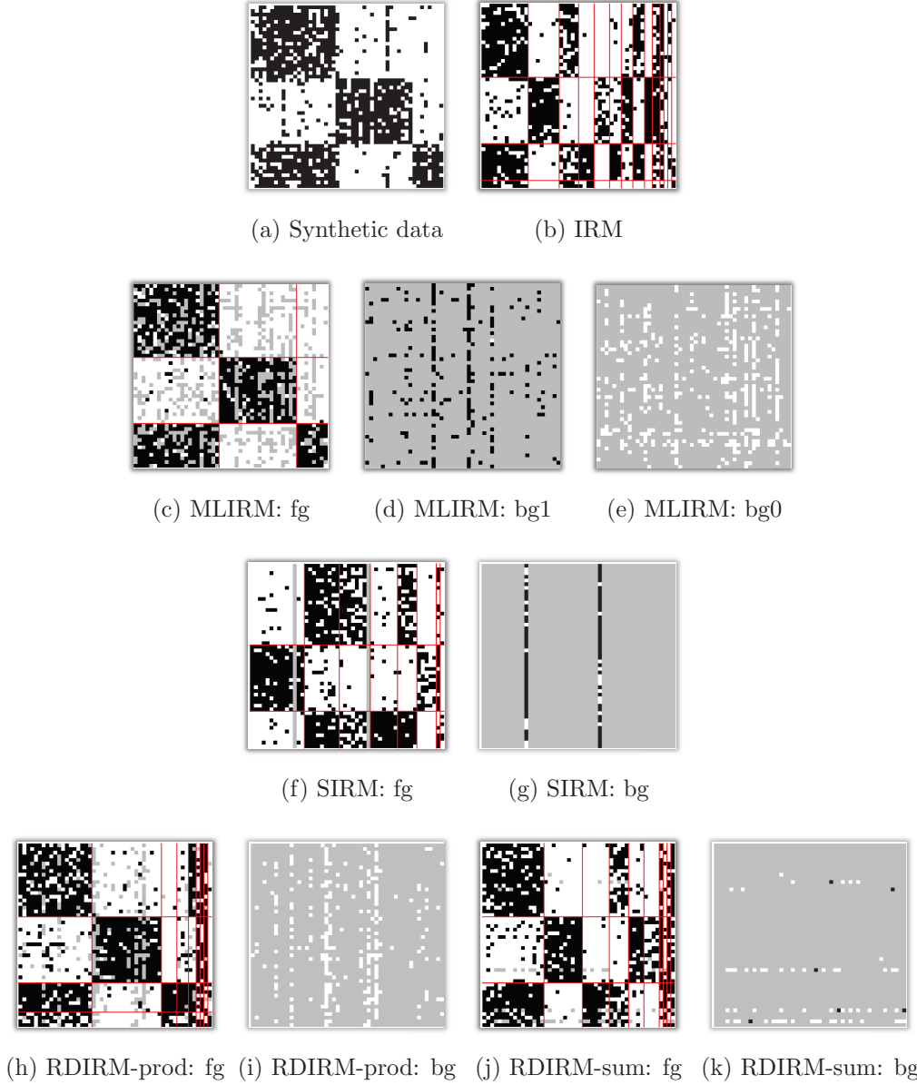
Figure 4.3: Synthetic data example. (a) Synthetic 50 \times 50 relational data (white corresponds to zero, black to one). (b) IRM solution (rows and columns are sorted by the estimated cluster indices). (c)–(e) MLIRM solutions. (c) shows the area assigned to the clustering layer r_{i,j} = \text{fg} , (d) to the first background layer r_{i,j} = \text{bg1} , and (e) to the background layer r_{i,j} = \text{bg0} (gray area indicates that corresponding entries are assigned to other layers). (f)–(k) Solutions produced by SIRM, RDIRM-prod, and RDIRM-sum, respectively.
